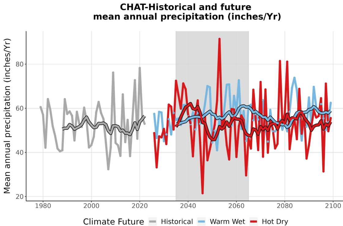
Figure 4. This graph compares observed average annual precipitation at CHAT (inches/year) (1979-2022) with projected average annual precipitation for the two climate futures over the period 2023-2099. The historically observed data is shown in gray, the Warm Wet climate future in blue, and the Hot Dry climate future in red. The smooth line running through each projection is the 10-year running average for historical observations and future projections. The gray-shaded area represents the time period that was averaged (2035-2065) to summarize future projections for the year 2050 (Appendix 1).
