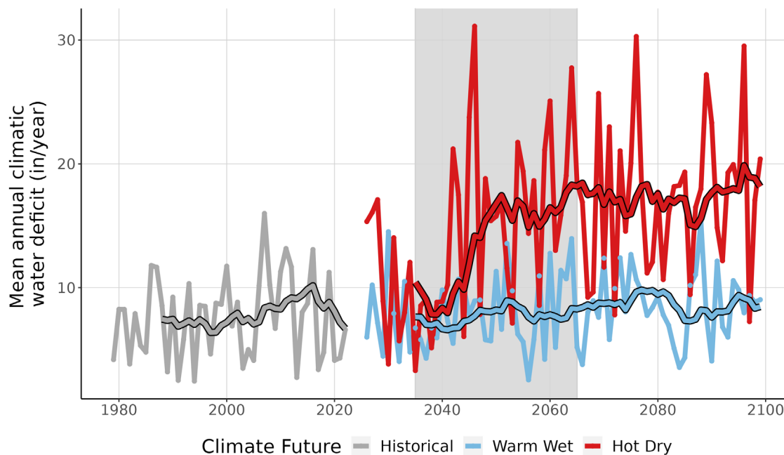
Figure 9. This line graph compares observed climatic water deficit at CHAT (inches/year) (1979-2022) with projected climatic water deficit for the two climate futures over the period 2023-2099. The historical observation data is shown in gray, the Warm Wet climate future in blue, and the Hot Dry climate future in red. The smooth line running through each projection is the 10-year running average for historical observations and future projections. Gray-shaded area represents the time period that was averaged (2035-2065) to summarize future projections for the year 2050.
