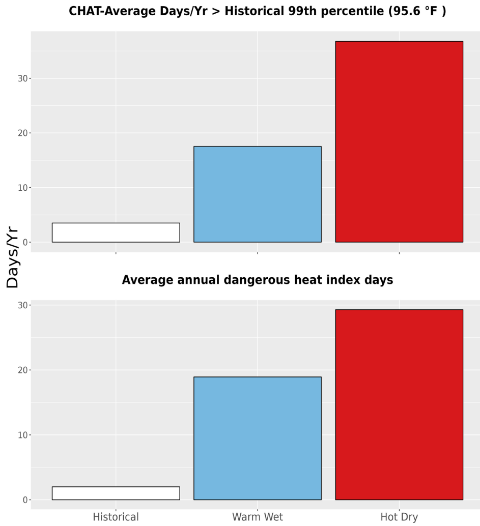
Figure 5. The upper bar graph represents the average number of days annually with temperatures greater than the historical 99th percentile (95.6 °F) historically (1979-2012) and for the two climate futures (2050). The bottom bar graph represents the average annual number of dangerous heat index days historically and for the two climate futures. Dangerous heat index days are days that exceed 105 °F.
