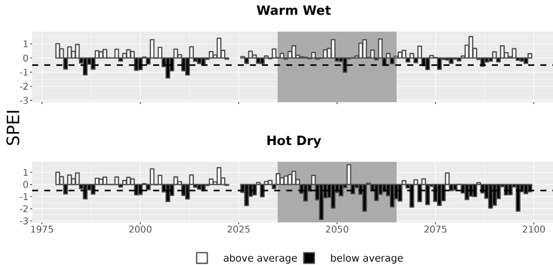
Figure 7. Drought metrics for CHAT. Drought index (SPEI; units = standard deviations from historical) timeseries for each climate future. Below-average SPEI (black bars) indicates dry conditions. The dotted line (SPEI = -0.5) indicates drought conditions.
