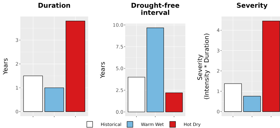
Figure 8. Drought metrics for CHAT. (Left) Average drought duration (years) historically (1979-2012) and under each climate future. (Middle) Average drought return interval (years), indicating the expected amount of time between periods of drought, historically and under each climate future. (Right) Average drought severity, a measure of drought intensity multiplied by duration, historically and under each climate future.
