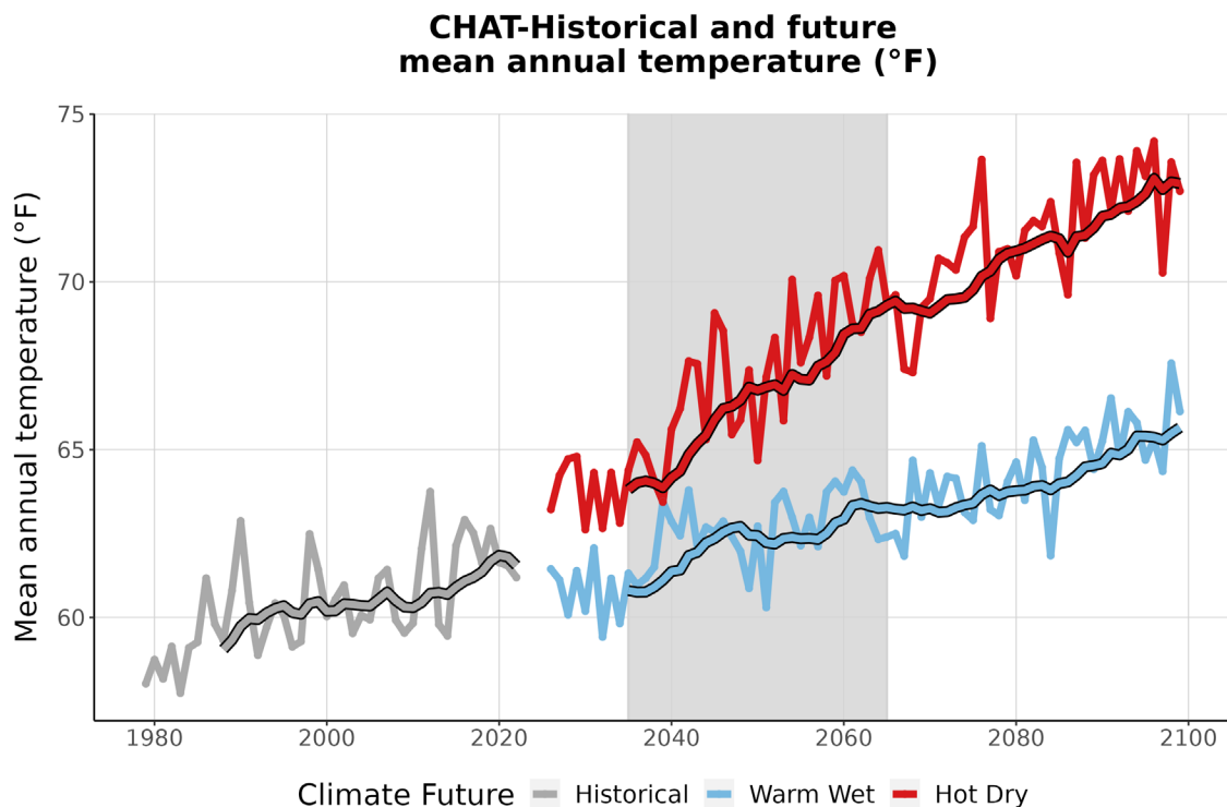
Figure 3. This graph compares observed average annual temperature at CHAT (°F) (1979-2022) with projected average annual temperature for the two climate futures over the period 2023-2099. The historically observed data
