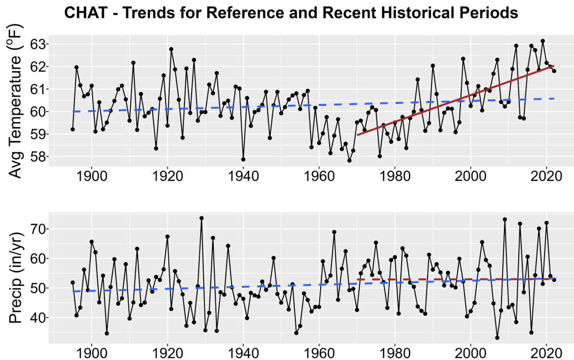
Figure 1. Historical trends in annual average temperature (upper plot) and annual total precipitation (lower plot) for CHAT from 1895-2022. Black points show yearly values while blue lines are linear regressions for the entire period record and red lines for 1970-2022 trends. Solid lines are significant trends (i.e., p < 0.05 ); dashed lines are not statistically significant.
