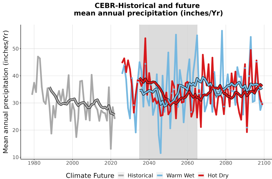
Figure 4. This graph compares observed average annual precipitation at CEBR (inches/year) (1979-2022) with projected average annual precipitation for the two climate futures over the period 2023-2099. The historically observed data is shown in gray, the Warm Wet climate future in blue, and the Hot Dry climate future in red. The smooth line running through each projection is the 10-year running average for historical observations and future projections. The gray-shaded area represents the time period that was averaged (2035-2065) to summarize future projections for the year 2050 (Appendix 1).
