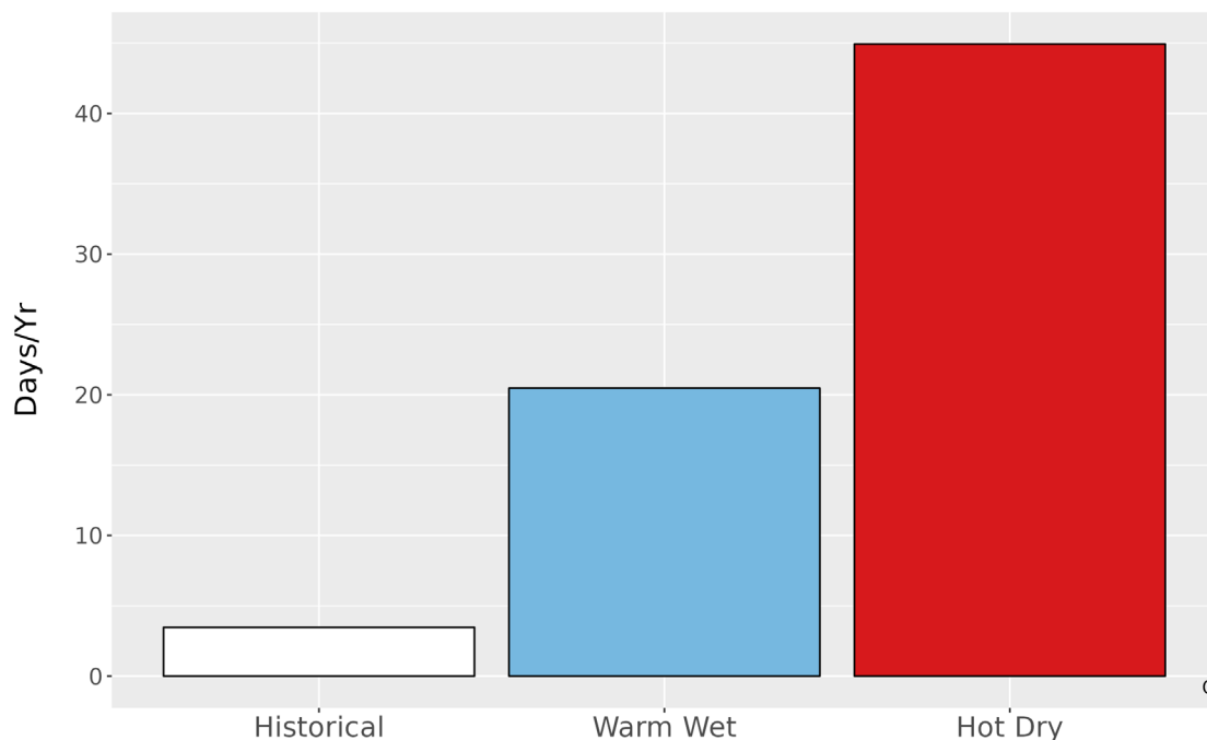
Figure 5. Metrics of extreme temperature at CEBR. The bar graph represents the average number of days annually with temperatures greater than the historical 99th percentile (76.4 °F) historically (1979-2012) and for the two climate futures (2050).
