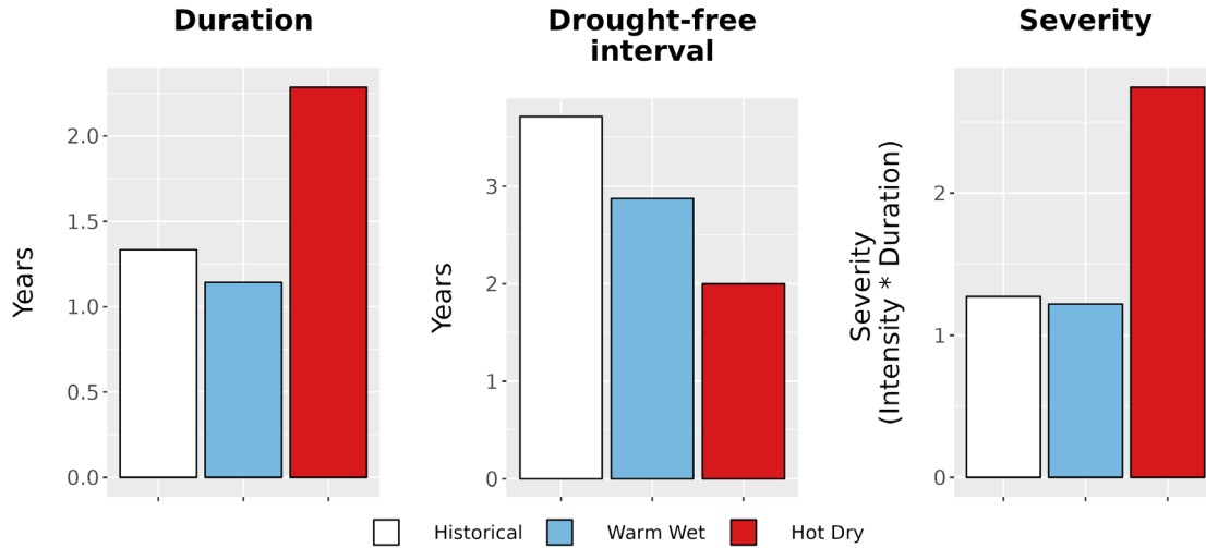
Figure 8. Drought metrics for CEBR. (Left) Average drought duration (years) historically (1979-2012) and under each climate future. (Middle) Average drought return interval (years), indicating the expected amount of time between periods of drought, historically and under each climate future. (Right) Average drought severity, a measure of drought intensity multiplied by duration, historically and under each climate future.
