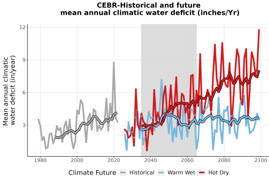
Figure 9. This line graph compares observed climatic water deficit at CEBR (inches/year) (1979-2022) with projected climatic water deficit for the two climate futures over the period 2023-2099. The historical observation data is shown in gray, the Warm Wet climate future in blue, and the Hot Dry climate future in red. The smooth line running through each projection is the 10-year running average for historical observations and future projections. Gray-shaded area represents the time period that was averaged (2035-2065) to summarize future projections for the year 2050.
