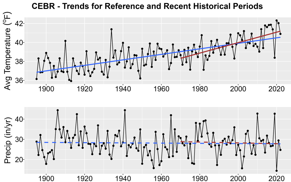
Figure 1. Historical trends in annual average temperature (upper plot) and annual total precipitation (lower plot) for CEBR from 1895-2022. Black points show yearly values while blue lines are linear regressions for the entire period record and red lines for 1970-2022 trends. Solid lines are significant trends (i.e., p < 0.05 ); dashed lines are not statistically significant.
