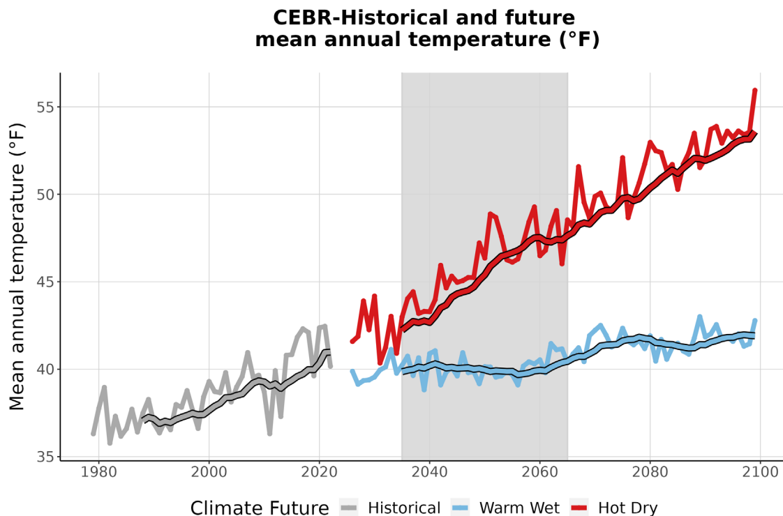
Figure 3. This graph compares observed average annual temperature at CEBR (°F) (1979-2022) with projected average annual temperature for the two climate futures over the period 2023-2099. The historically observed data
