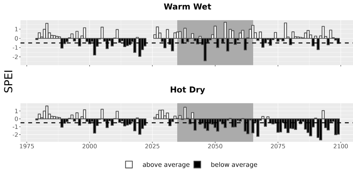
Figure 7. Drought metrics for CEBR. Drought index (SPEI; units = standard deviations from historical) timeseries for each climate future. Below-average SPEI (black bars) indicates dry conditions. The dotted line (SPEI = -0.5) indicates drought conditions.
