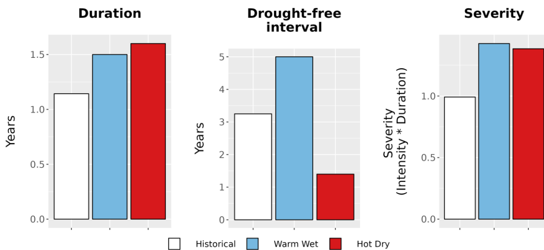
Figure 8. Drought metrics for CAWO. (Left) Average drought duration (years) historically (1979-2012) and under each climate future. (Middle) Average drought return interval (years), indicating the expected amount of time between periods of drought, historically and under each climate future. (Right) Average drought severity, a measure of drought intensity multiplied by duration, historically and under each climate future.
