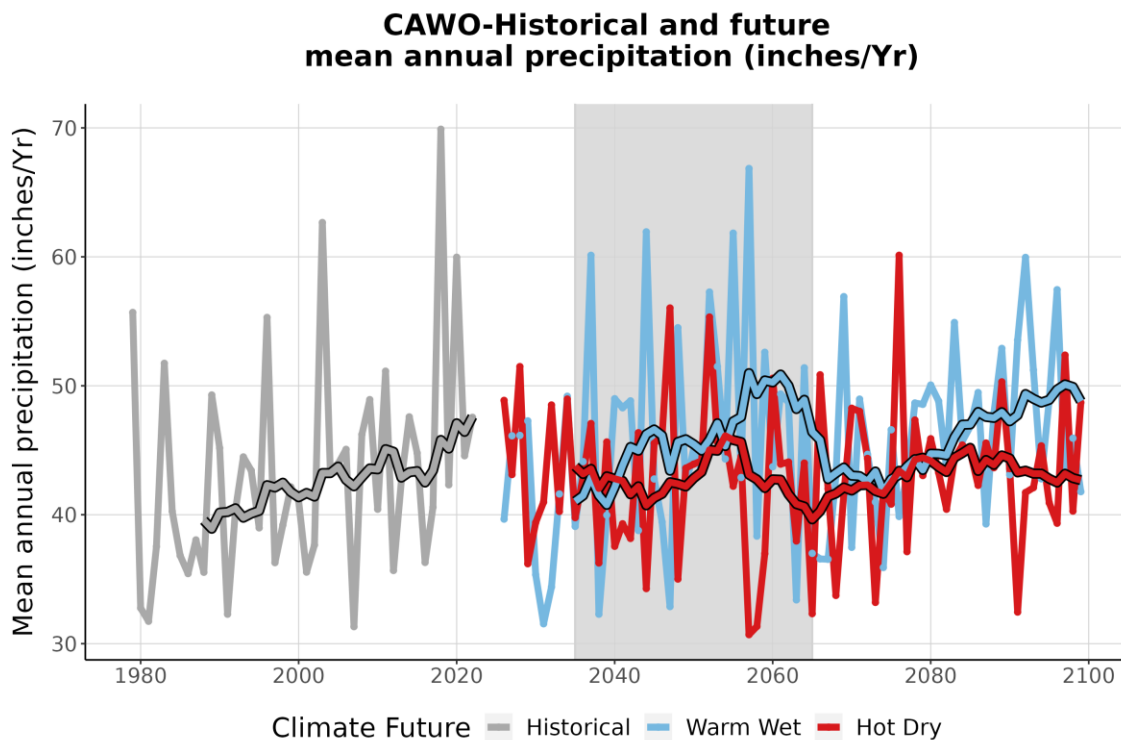
Figure 4. This graph compares observed average annual precipitation at CAWO (inches/year) (1979-2022) with projected average annual precipitation for the two climate futures over the period 2023-2099. The historically observed data is shown in gray, the Warm Wet climate future in blue, and the Hot Dry climate future in red. The smooth line running through each projection is the 10-year running average for historical observations and future projections. The gray-shaded area represents the time period that was averaged (2035-2065) to summarize future projections for the year 2050 (Appendix 1).
