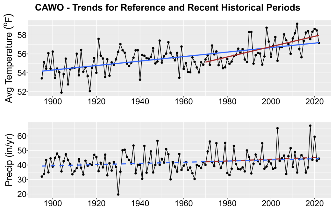
Figure 1. Historical trends in annual average temperature (upper plot) and annual total precipitation (lower plot) for CAWO from 1895-2022. Black points show yearly values while blue lines are linear regressions for the entire period record and red lines for 1970-2022 trends. Solid lines are significant trends (i.e., p < 0.05 ); dashed lines are not statistically significant.
