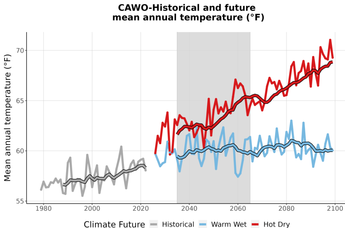
Figure 3. This graph compares observed average annual temperature at CAWO (°F) (1979-2022) with projected average annual temperature for the two climate futures over the period 2023-2099. The historically observed data
