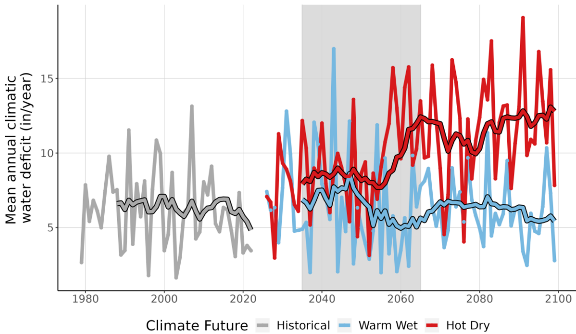
Figure 9. This line graph compares observed climatic water deficit at CAWO (inches/year) (1979-2022) with projected climatic water deficit for the two climate futures over the period 2023-2099. The historical observation data is shown in gray, the Warm Wet climate future in blue, and the Hot Dry climate future in red. The smooth line running through each projection is the 10-year running average for historical observations and future projections. Gray-shaded area represents the time period that was averaged (2035-2065) to summarize future projections for the year 2050.
