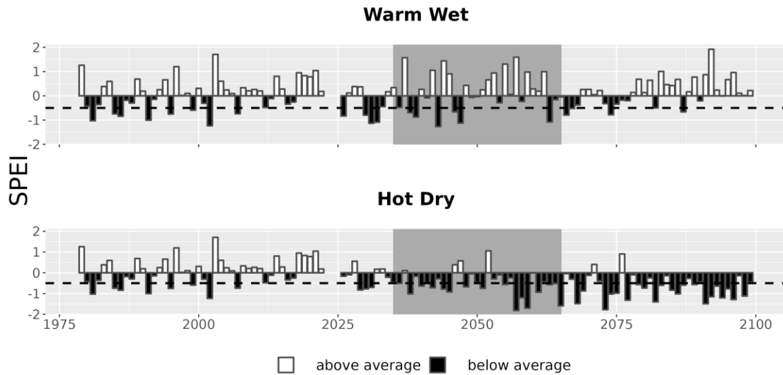
Figure 7. Drought metrics for CAWO. Drought index (SPEI; units = standard deviations from historical) timeseries for each climate future. Below-average SPEI (black bars) indicates dry conditions. The dotted line (SPEI = -0.5) indicates drought conditions.
