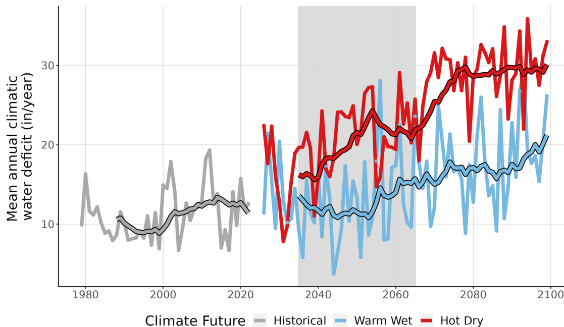
Figure 9. This line graph compares observed climatic water deficit at CAVO (inches/year) (1979-2022) with projected climatic water deficit for the two climate futures over the period 2023-2099. The historical observation data is shown in gray, the Warm Wet climate future in blue, and the Hot Dry climate future in red. The smooth line running through each projection is the 10-year running average for historical observations and future projections. Gray-shaded area represents the time period that was averaged (2035-2065) to summarize future projections for the year 2050.
