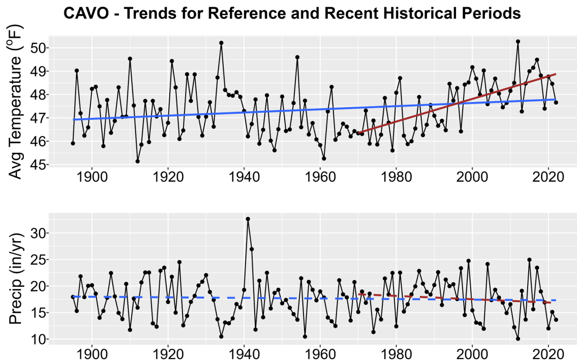
Figure 1. Historical trends in annual average temperature (upper plot) and annual total precipitation (lower plot) for CAVO from 1895-2022. Black points show yearly values while blue lines are linear regressions for the entire period record and red lines for 1970-2022 trends. Solid lines are significant trends (i.e., p < 0.05 ); dashed lines are not statistically significant.
