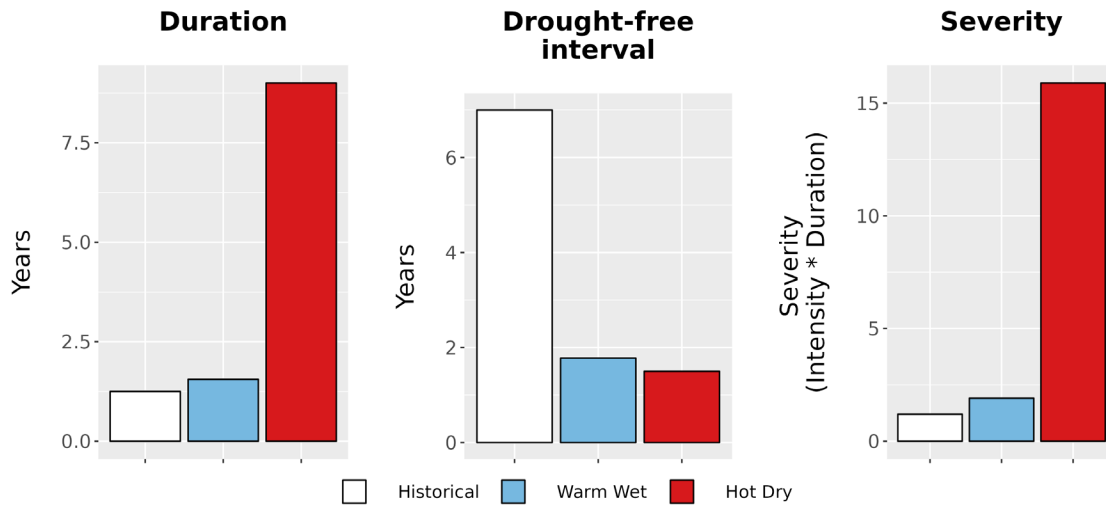
Figure 8. Drought metrics for CAVO. (Left) Average drought duration (years) historically (1979-2012) and under each climate future. (Middle) Average drought return interval (years), indicating the expected amount of time between periods of drought, historically and under each climate future. (Right) Average drought severity, a measure of drought intensity multiplied by duration, historically and under each climate future.
