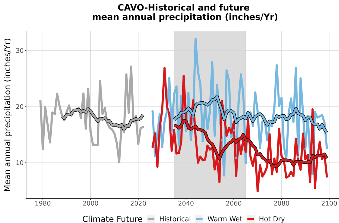
Figure 4. This graph compares observed average annual precipitation at CAVO (inches/year) (1979-2022) with projected average annual precipitation for the two climate futures over the period 2023-2099. The historically observed data is shown in gray, the Warm Wet climate future in blue, and the Hot Dry climate future in red. The smooth line running through each projection is the 10-year running average for historical observations and future projections. The gray-shaded area represents the time period that was averaged (2035-2065) to summarize future projections for the year 2050 (Appendix 1).
