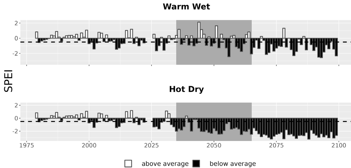
Figure 7. Drought metrics for CAVO. Drought index (SPEI; units = standard deviations from historical) timeseries for each climate future. Below-average SPEI (black bars) indicates dry conditions. The dotted line (SPEI = -0.5) indicates drought conditions.
