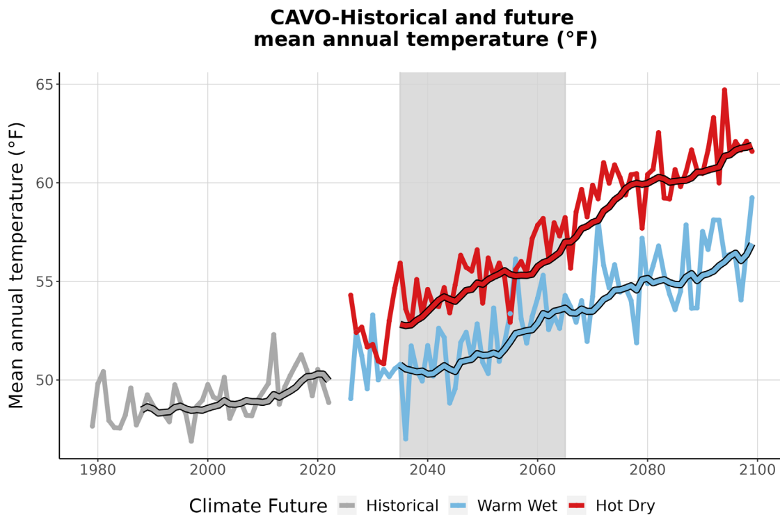
Figure 3. This graph compares observed average annual temperature at CAVO (°F) (1979-2022) with projected average annual temperature for the two climate futures over the period 2023-2099. The historically observed data is shown in gray, the Warm Wet climate future in blue, and the Hot Dry climate future in red. The smooth line
