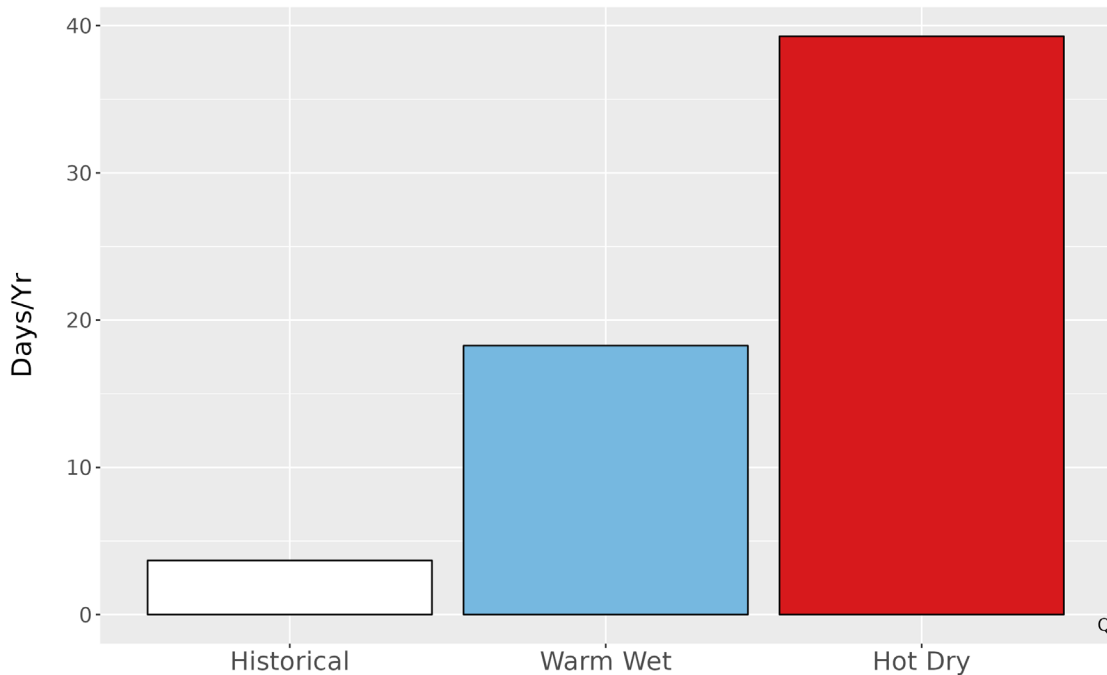
Figure 5. Metrics of extreme temperature at CAVO. The bar graph represents the average number of days annually with temperatures greater than the historical 99th percentile (89.1 °F) historically (1979-2012) and for the two climate futures (2050).
