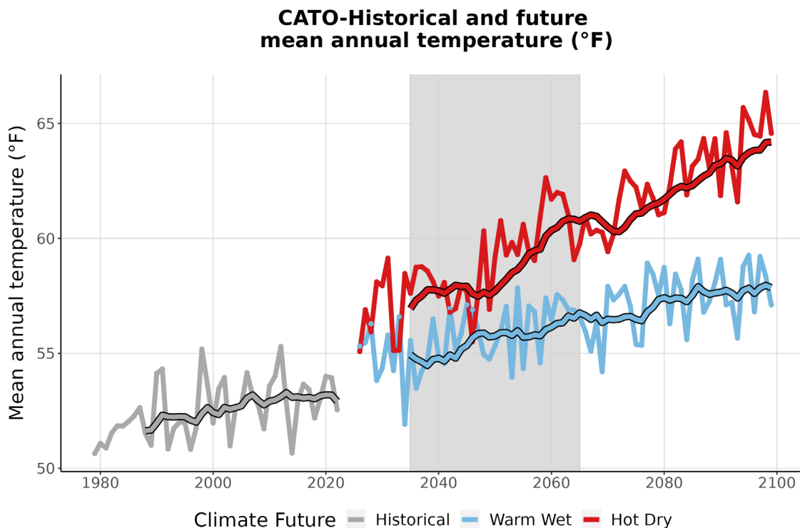
Figure 3. This graph compares observed average annual temperature at CATO (°F) (1979-2022) with projected average annual temperature for the two climate futures over the period 2023-2099. The historically observed data
