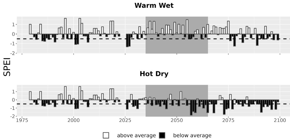
Figure 7. Drought metrics for CATO. Drought index (SPEI; units = standard deviations from historical) timeseries for each climate future. Below-average SPEI (black bars) indicates dry conditions. The dotted line (SPEI = -0.5) indicates drought conditions.
