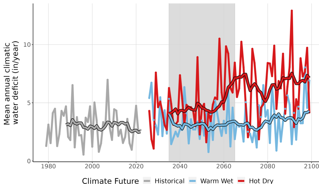
Figure 9. This line graph compares observed climatic water deficit at CATO (inches/year) (1979-2022) with projected climatic water deficit for the two climate futures over the period 2023-2099. The historical observation data is shown in gray, the Warm Wet climate future in blue, and the Hot Dry climate future in red. The smooth line running through each projection is the 10-year running average for historical observations and future projections. Gray-shaded area represents the time period that was averaged (2035-2065) to summarize future projections for the year 2050.
