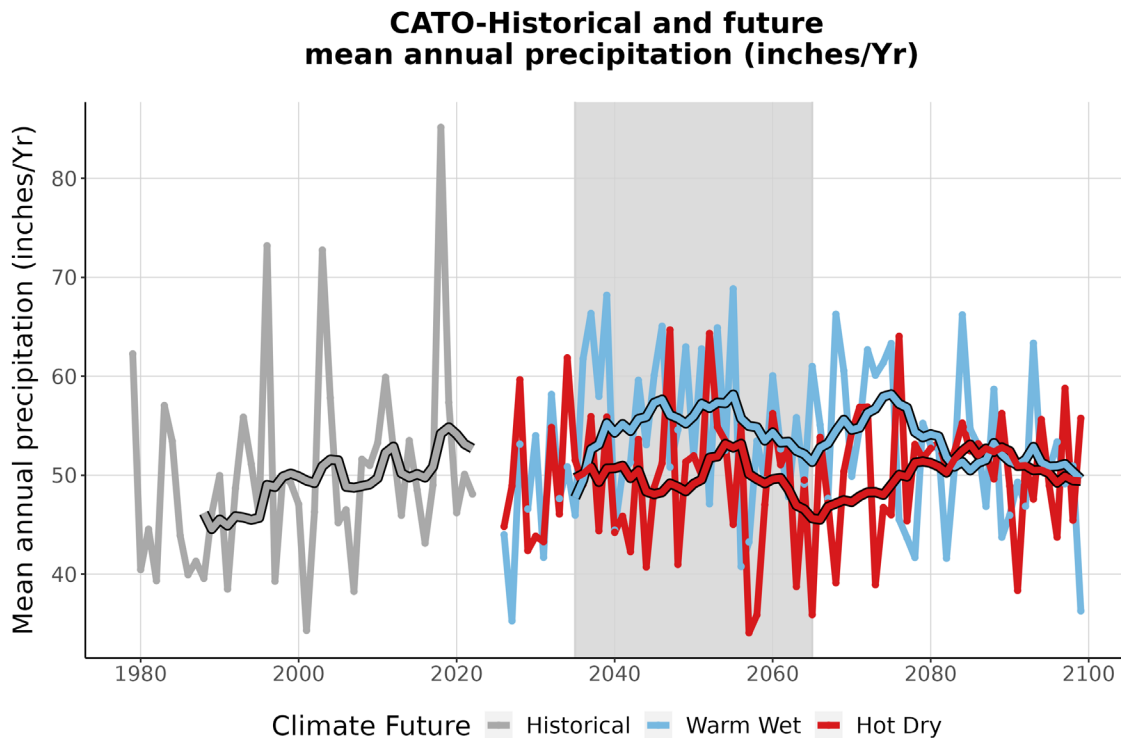
Figure 4. This graph compares observed average annual precipitation at CATO (inches/year) (1979-2022) with projected average annual precipitation for the two climate futures over the period 2023-2099. The historically observed data is shown in gray, the Warm Wet climate future in blue, and the Hot Dry climate future in red. The smooth line running through each projection is the 10-year running average for historical observations and future projections. The gray-shaded area represents the time period that was averaged (2035-2065) to summarize future projections for the year 2050 (Appendix 1).
