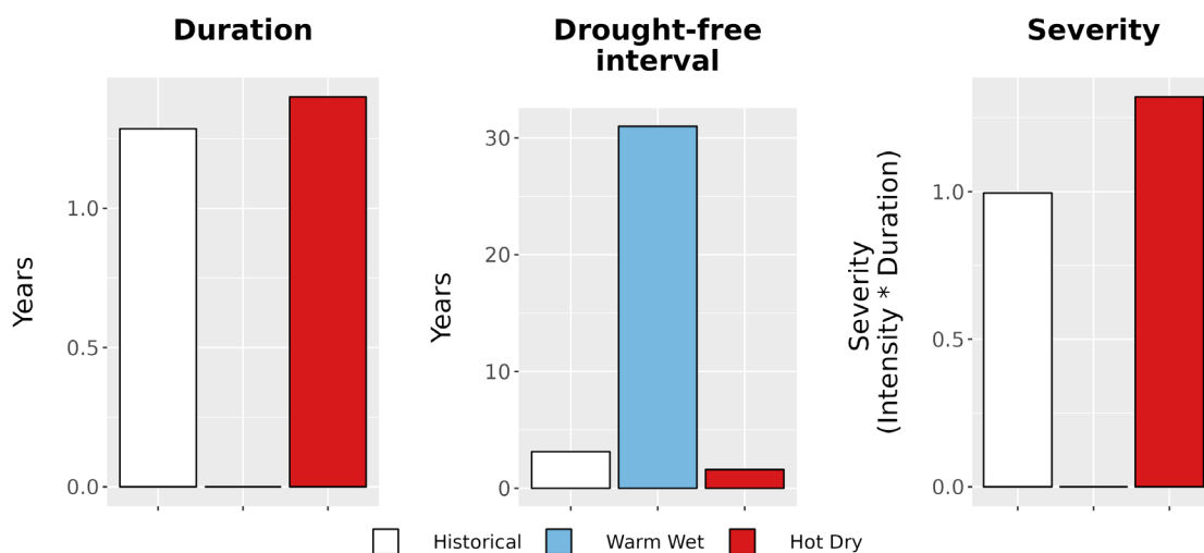
Figure 8. Drought metrics for CATO. (Left) Average drought duration (years) historically (1979-2012) and under each climate future. (Middle) Average drought return interval (years), indicating the expected amount of time between periods of drought, historically and under each climate future. (Right) Average drought severity, a measure of drought intensity multiplied by duration, historically and under each climate future.
