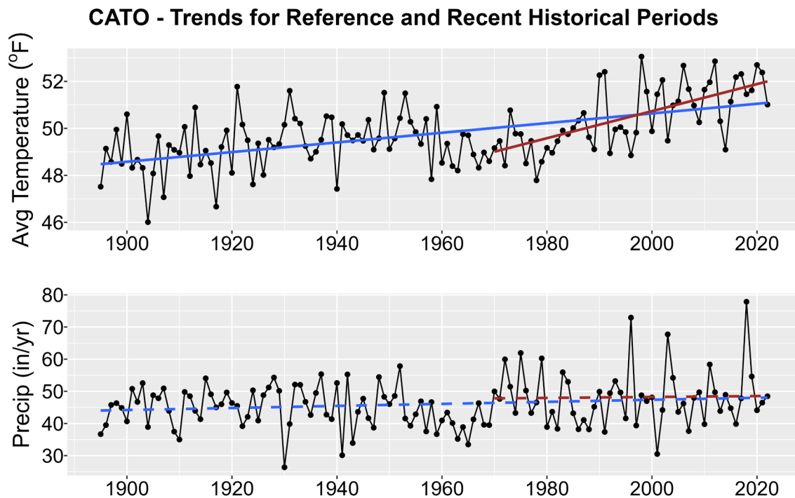
Figure 1. Historical trends in annual average temperature (upper plot) and annual total precipitation (lower plot) for CATO from 1895-2022. Black points show yearly values while blue lines are linear regressions for the entire period record and red lines for 1970-2022 trends. Solid lines are significant trends (i.e., p < 0.05 ); dashed lines are not statistically significant.
