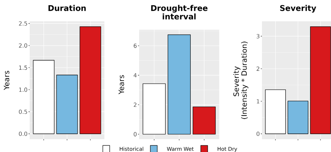
Figure 8. Drought metrics for CASA. (Left) Average drought duration (years) historically (1979-2012) and under each climate future. (Middle) Average drought return interval (years), indicating the expected amount of time between periods of drought, historically and under each climate future. (Right) Average drought severity, a measure of drought intensity multiplied by duration, historically and under each climate future.
