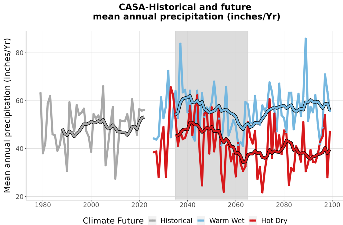
Figure 4. This graph compares observed average annual precipitation at CASA (inches/year) (1979-2022) with projected average annual precipitation for the two climate futures over the period 2023-2099. The historically observed data is shown in gray, the Warm Wet climate future in blue, and the Hot Dry climate future in red. The smooth line running through each projection is the 10-year running average for historical observations and future projections. The gray-shaded area represents the time period that was averaged (2035-2065) to summarize future projections for the year 2050 (Appendix 1).
