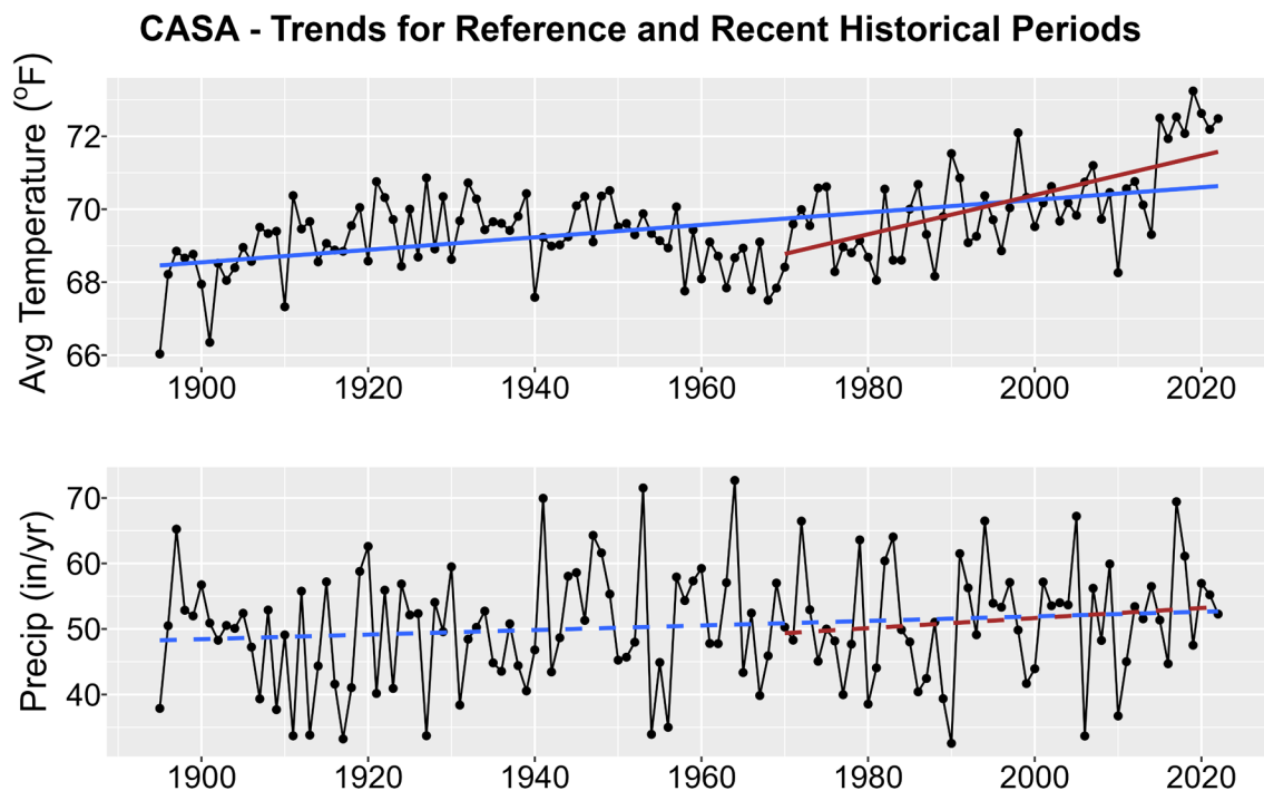
Figure 1. Historical trends in annual average temperature (upper plot) and annual total precipitation (lower plot) for CASA from 1895-2022. Black points show yearly values while blue lines are linear regressions for the entire period record and red lines for 1970-2022 trends. Solid lines are significant trends (i.e., p < 0.05 ); dashed lines are not statistically significant.
