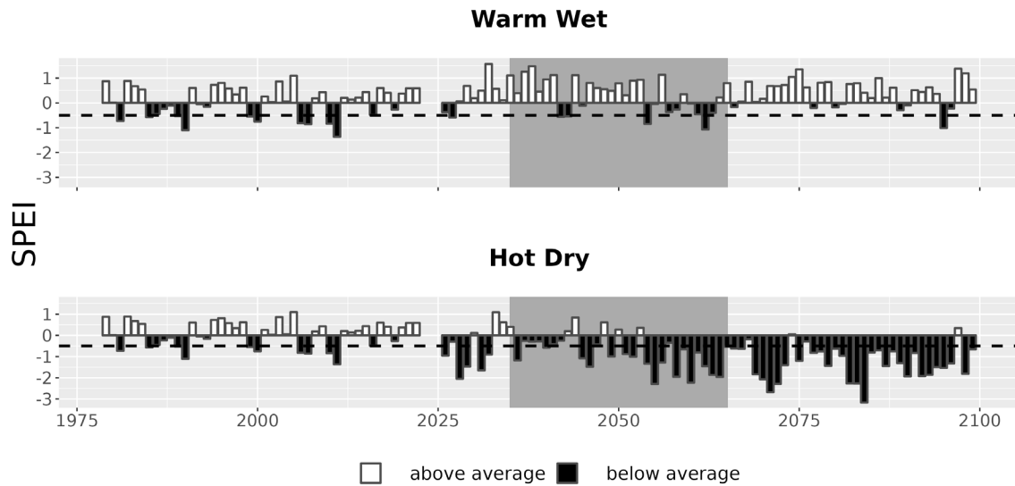
Figure 7. Drought metrics for CASA. Drought index (SPEI; units = standard deviations from historical) timeseries for each climate future. Below-average SPEI (black bars) indicates dry conditions. The dotted line (SPEI = -0.5) indicates drought conditions.
