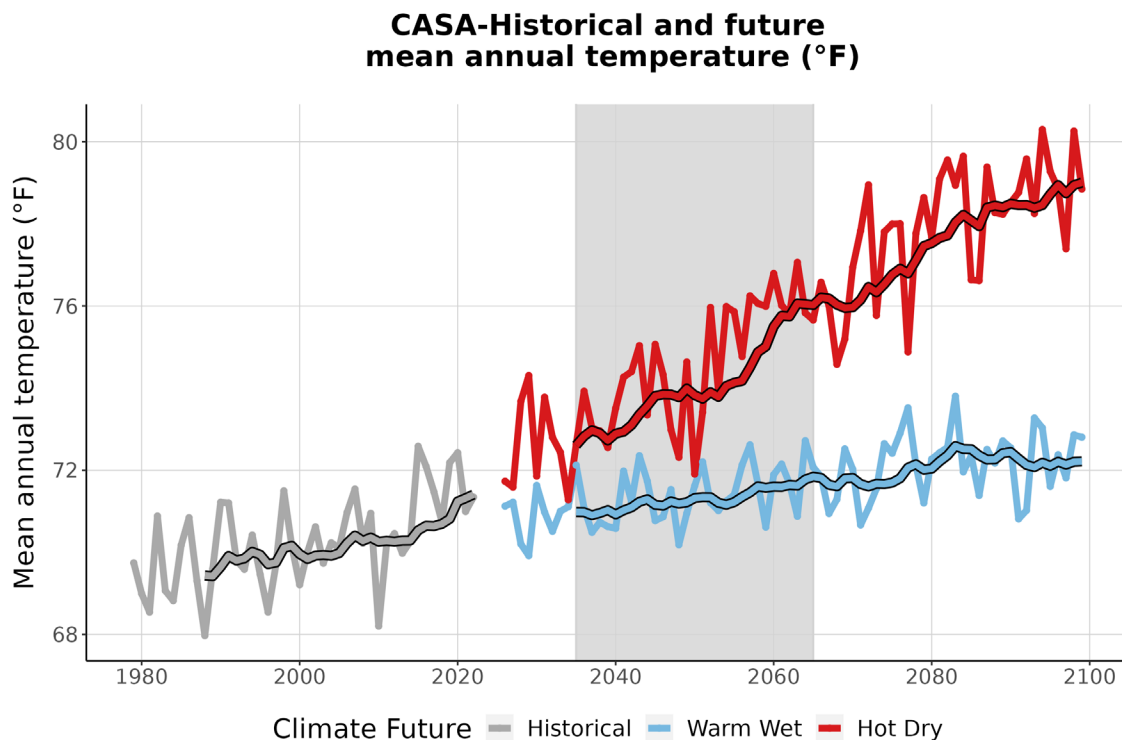
Figure 3. This graph compares observed average annual temperature at CASA (°F) (1979-2022) with projected average annual temperature for the two climate futures over the period 2023-2099. The historically observed data
