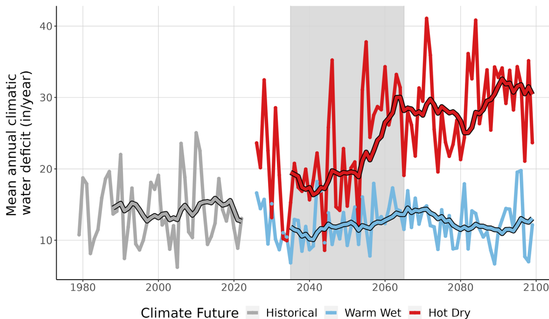
Figure 9. This line graph compares observed climatic water deficit at CASA (inches/year) (1979-2022) with projected climatic water deficit for the two climate futures over the period 2023-2099. The historical observation data is shown in gray, the Warm Wet climate future in blue, and the Hot Dry climate future in red. The smooth line running through each projection is the 10-year running average for historical observations and future projections. Gray-shaded area represents the time period that was averaged (2035-2065) to summarize future projections for the year 2050.
