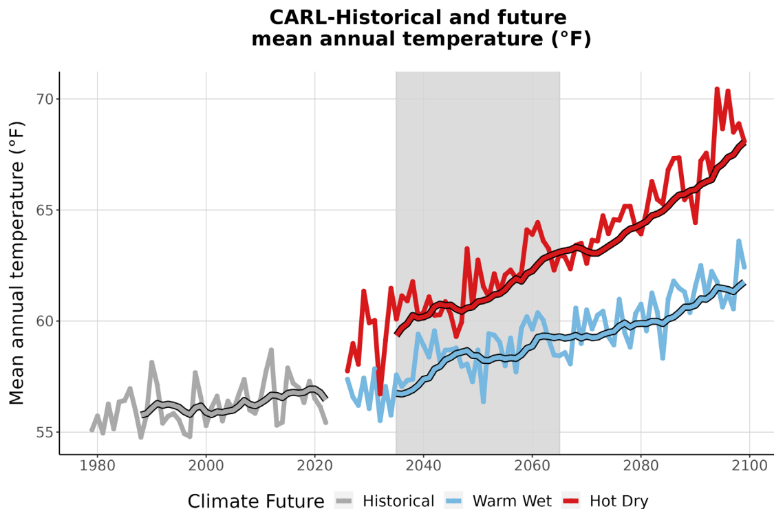
Figure 3. This graph compares observed average annual temperature at CARL (°F) (1979-2022) with projected average annual temperature for the two climate futures over the period 2023-2099. The historically observed data
