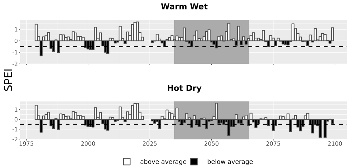
Figure 7. Drought metrics for CARL. Drought index (SPEI; units = standard deviations from historical) timeseries for each climate future. Below-average SPEI (black bars) indicates dry conditions. The dotted line (SPEI = -0.5) indicates drought conditions.
