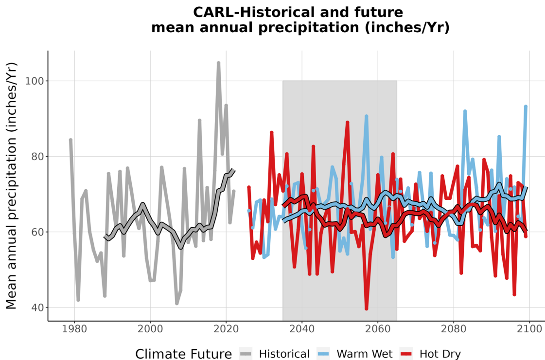
Figure 4. This graph compares observed average annual precipitation at CARL (inches/year) (1979-2022) with projected average annual precipitation for the two climate futures over the period 2023-2099. The historically observed data is shown in gray, the Warm Wet climate future in blue, and the Hot Dry climate future in red. The smooth line running through each projection is the 10-year running average for historical observations and future projections. The gray-shaded area represents the time period that was averaged (2035-2065) to summarize future projections for the year 2050 (Appendix 1).
