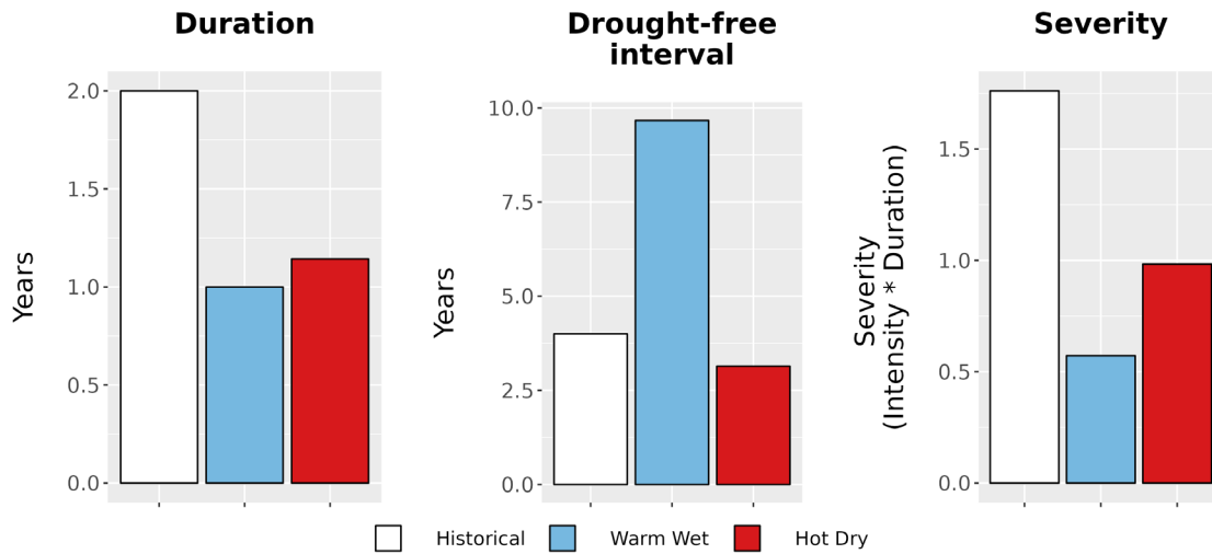
Figure 8. Drought metrics for CARL. (Left) Average drought duration (years) historically (1979-2012) and under each climate future. (Middle) Average drought return interval (years), indicating the expected amount of time between periods of drought, historically and under each climate future. (Right) Average drought severity, a measure of drought intensity multiplied by duration, historically and under each climate future.
