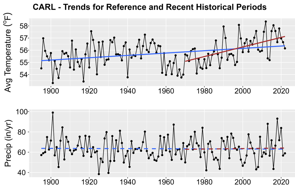
Figure 1. Historical trends in annual average temperature (upper plot) and annual total precipitation (lower plot) for CARL from 1895-2022. Black points show yearly values while blue lines are linear regressions for the entire period record and red lines for 1970-2022 trends. Solid lines are significant trends (i.e., p < 0.05 ); dashed lines are not statistically significant.
