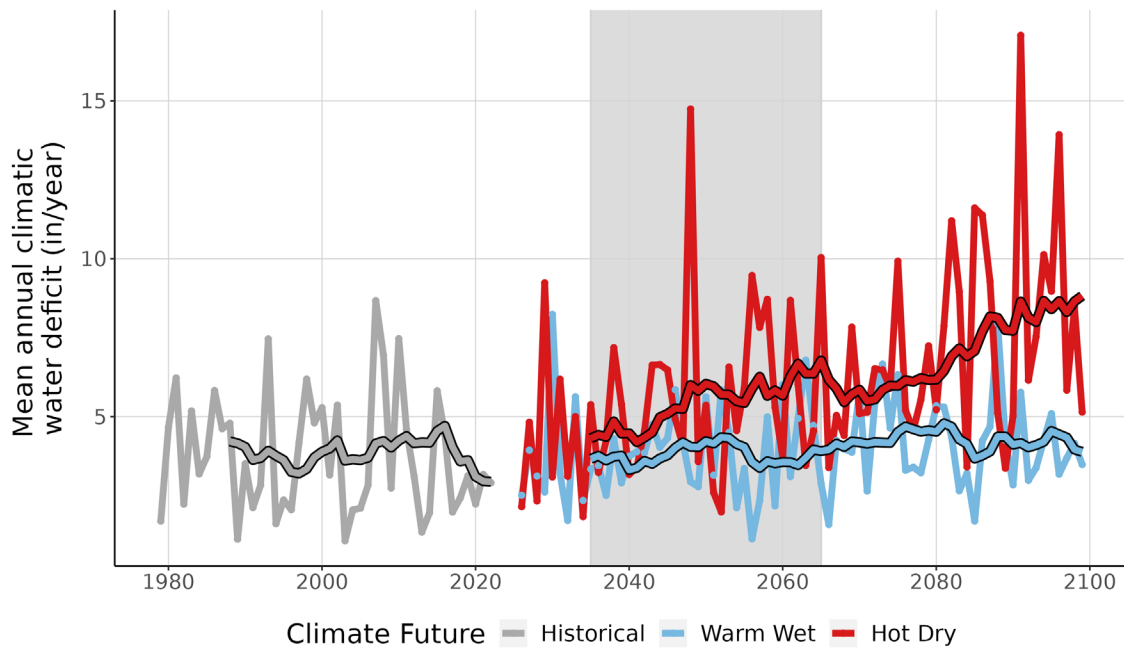
Figure 9. This line graph compares observed climatic water deficit at CARL (inches/year) (1979-2022) with projected climatic water deficit for the two climate futures over the period 2023-2099. The historical observation data is shown in gray, the Warm Wet climate future in blue, and the Hot Dry climate future in red. The smooth line running through each projection is the 10-year running average for historical observations and future projections. Gray-shaded area represents the time period that was averaged (2035-2065) to summarize future projections for the year 2050.
