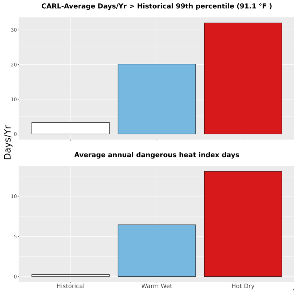
Figure 5. The upper bar graph represents the average number of days annually with temperatures greater than the historical 99th percentile (91.1 °F) historically (1979-2012) and for the two climate futures (2050). The bottom bar graph represents the average annual number of dangerous heat index days historically and for the two climate futures. Dangerous heat index days are days that exceed 105 °F.
