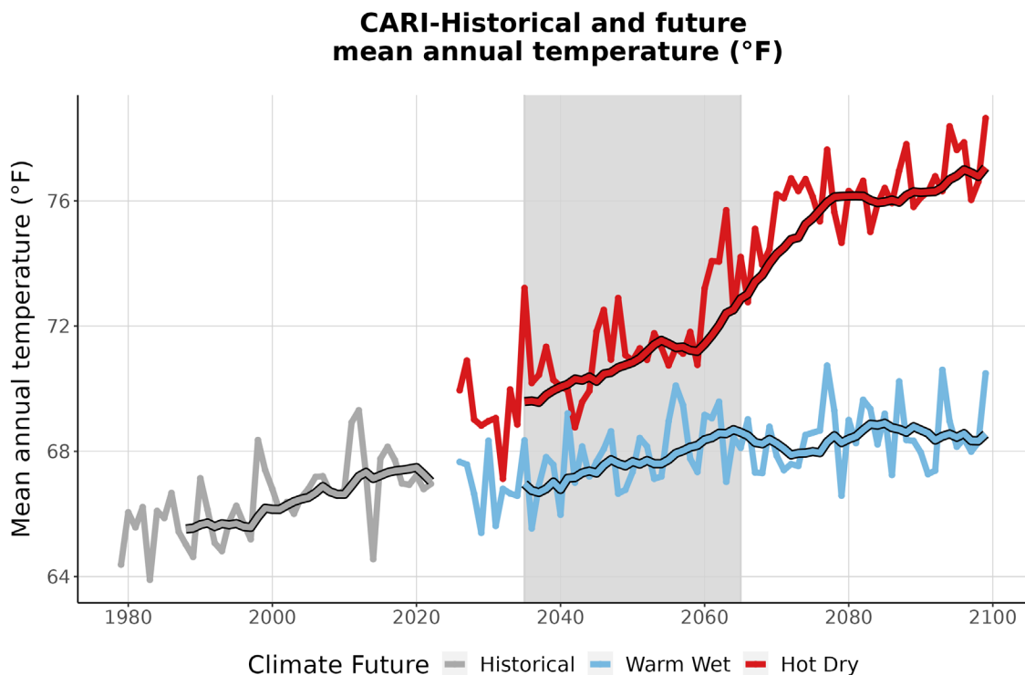
Figure 3. This graph compares observed average annual temperature at CARI (°F) (1979-2022) with projected average annual temperature for the two climate futures over the period 2023-2099. The historically observed data
