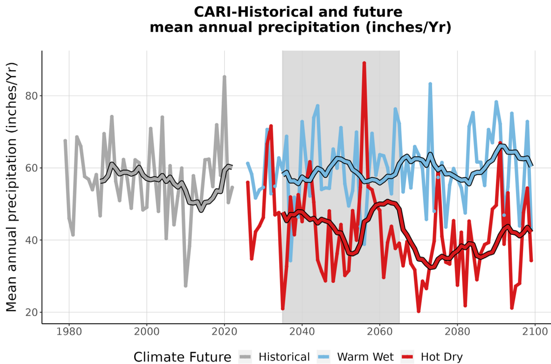
Figure 4. This graph compares observed average annual precipitation at CARI (inches/year) (1979-2022) with projected average annual precipitation for the two climate futures over the period 2023-2099. The historically observed data is shown in gray, the Warm Wet climate future in blue, and the Hot Dry climate future in red. The smooth line running through each projection is the 10-year running average for historical observations and future projections. The gray-shaded area represents the time period that was averaged (2035-2065) to summarize future projections for the year 2050 (Appendix 1).
