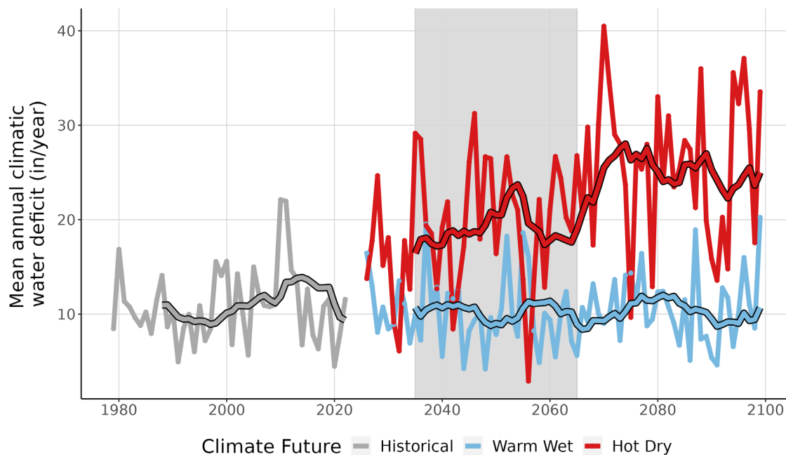
Figure 9. This line graph compares observed climatic water deficit at CARI (inches/year) (1979-2022) with projected climatic water deficit for the two climate futures over the period 2023-2099. The historical observation data is shown in gray, the Warm Wet climate future in blue, and the Hot Dry climate future in red. The smooth line running through each projection is the 10-year running average for historical observations and future projections. Gray-shaded area represents the time period that was averaged (2035-2065) to summarize future projections for the year 2050.
