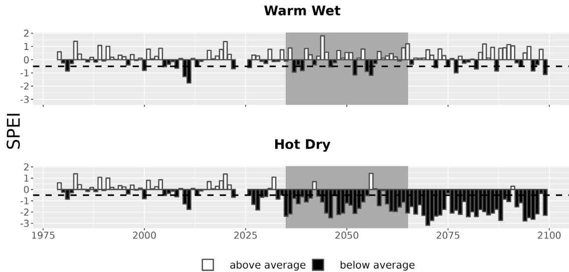
Figure 7. Drought metrics for CARI. Drought index (SPEI; units = standard deviations from historical) timeseries for each climate future. Below-average SPEI (black bars) indicates dry conditions. The dotted line (SPEI = -0.5) indicates drought conditions.
