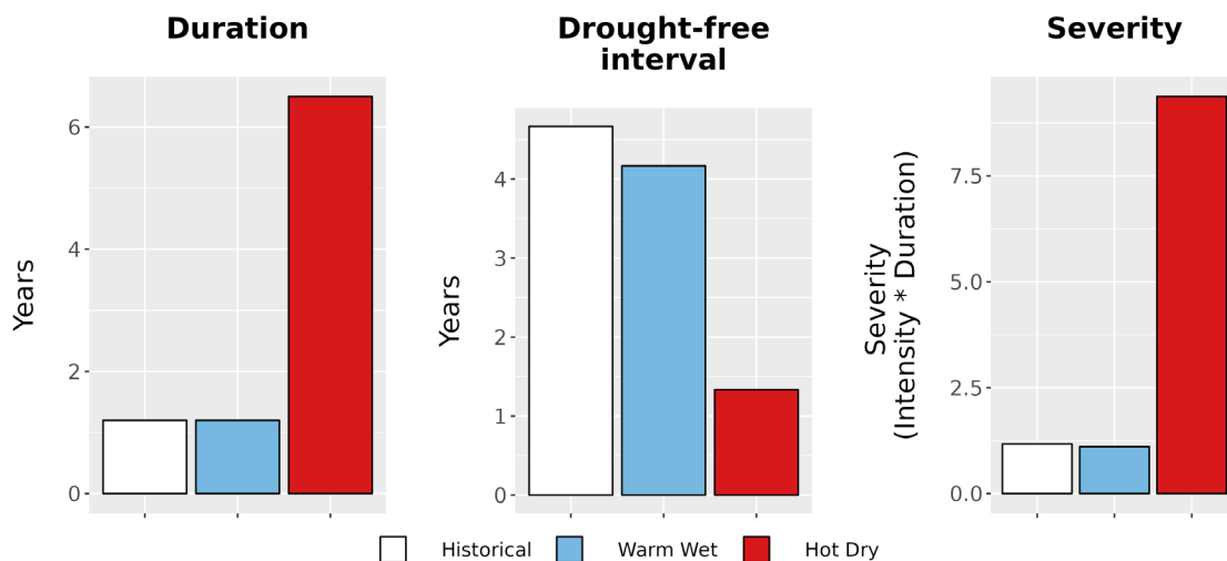
Figure 8. Drought metrics for CARI. (Left) Average drought duration (years) historically (1979-2012) and under each climate future. (Middle) Average drought return interval (years), indicating the expected amount of time between periods of drought, historically and under each climate future. (Right) Average drought severity, a measure of drought intensity multiplied by duration, historically and under each climate future.
