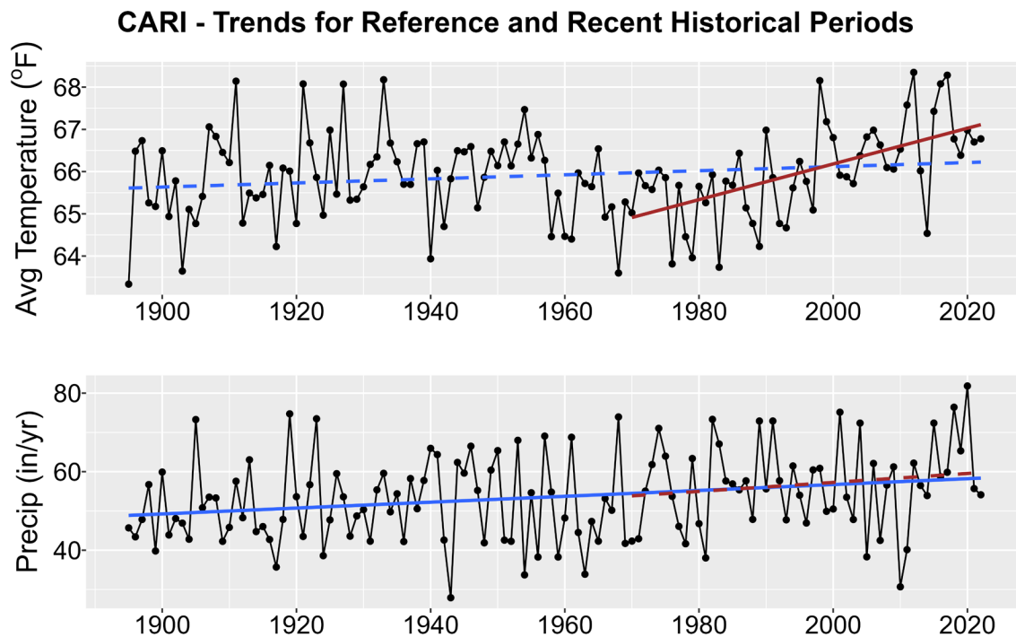
Figure 1. Historical trends in annual average temperature (upper plot) and annual total precipitation (lower plot) for CARI from 1895-2022. Black points show yearly values while blue lines are linear regressions for the entire period record and red lines for 1970-2022 trends. Solid lines are significant trends (i.e., p < 0.05 ); dashed lines are not statistically significant.
