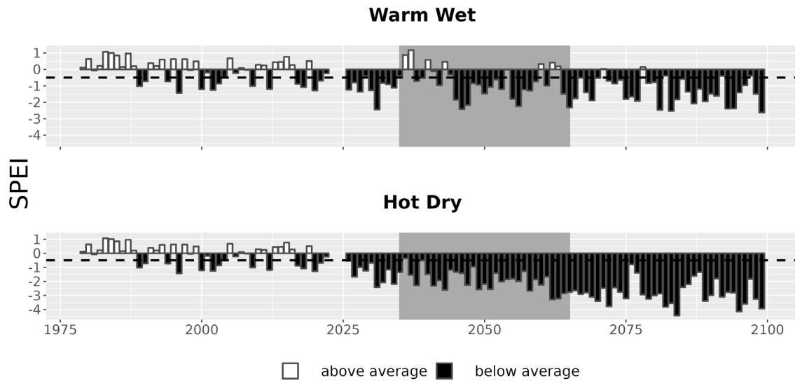
Figure 7. Drought metrics for CANY. Drought index (SPEI; units = standard deviations from historical) timeseries for each climate future. Below-average SPEI (black bars) indicates dry conditions. The dotted line (SPEI = -0.5) indicates drought conditions.
