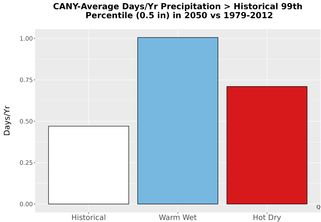
Figure 6. Average number of days annually with precipitation exceeding the 99th percentile (0.5 in.) of precipitation from the historical period 1979-2012 and for each climate future.
