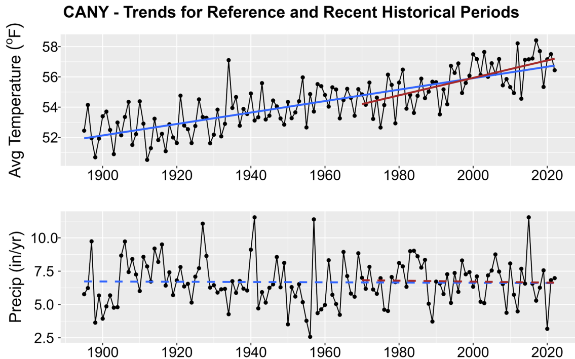
Figure 1. Historical trends in annual average temperature (upper plot) and annual total precipitation (lower plot) for CANY from 1895-2022. Black points show yearly values while blue lines are linear regressions for the entire period record and red lines for 1970-2022 trends. Solid lines are significant trends (i.e., p < 0.05 ); dashed lines are not statistically significant.
