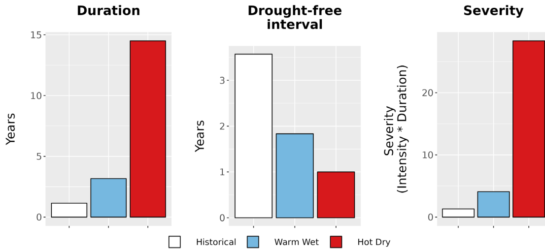
Figure 8. Drought metrics for CANY. (Left) Average drought duration (years) historically (1979-2012) and under each climate future. (Middle) Average drought return interval (years), indicating the expected amount of time between periods of drought, historically and under each climate future. (Right) Average drought severity, a measure of drought intensity multiplied by duration, historically and under each climate future.
