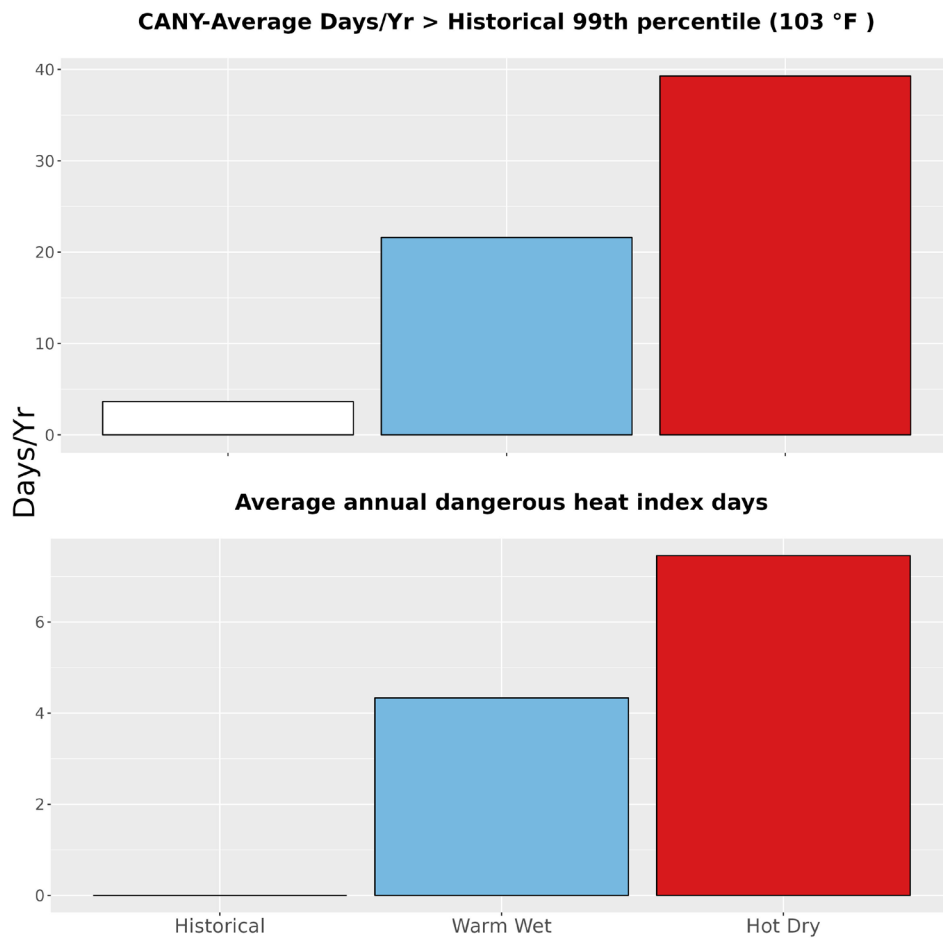
Figure 5. The upper bar graph represents the average number of days annually with temperatures greater than the historical 99th percentile (103 °F) historically (1979-2012) and for the two climate futures (2050). The bottom bar graph represents the average annual number of dangerous heat index days historically and for the two climate futures. Dangerous heat index days are days that exceed 105 °F.
