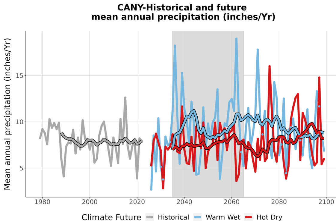
Figure 4. This graph compares observed average annual precipitation at CANY (inches/year) (1979-2022) with projected average annual precipitation for the two climate futures over the period 2023-2099. The historically observed data is shown in gray, the Warm Wet climate future in blue, and the Hot Dry climate future in red. The smooth line running through each projection is the 10-year running average for historical observations and future projections. The gray-shaded area represents the time period that was averaged (2035-2065) to summarize future projections for the year 2050 (Appendix 1).
