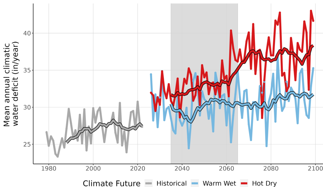
Figure 9. This line graph compares observed climatic water deficit at CANY (inches/year) (1979-2022) with projected climatic water deficit for the two climate futures over the period 2023-2099. The historical observation data is shown in gray, the Warm Wet climate future in blue, and the Hot Dry climate future in red. The smooth line running through each projection is the 10-year running average for historical observations and future projections. Gray-shaded area represents the time period that was averaged (2035-2065) to summarize future projections for the year 2050.
