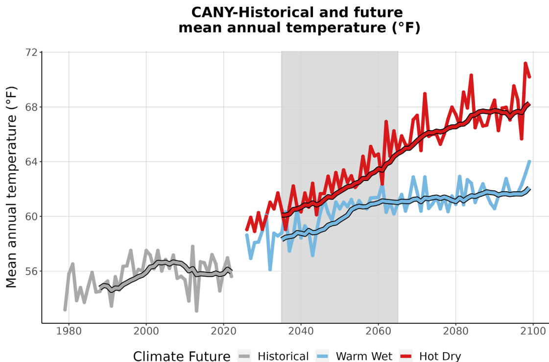
Figure 3. This graph compares observed average annual temperature at CANY (°F) (1979-2022) with projected average annual temperature for the two climate futures over the period 2023-2099. The historically observed data
