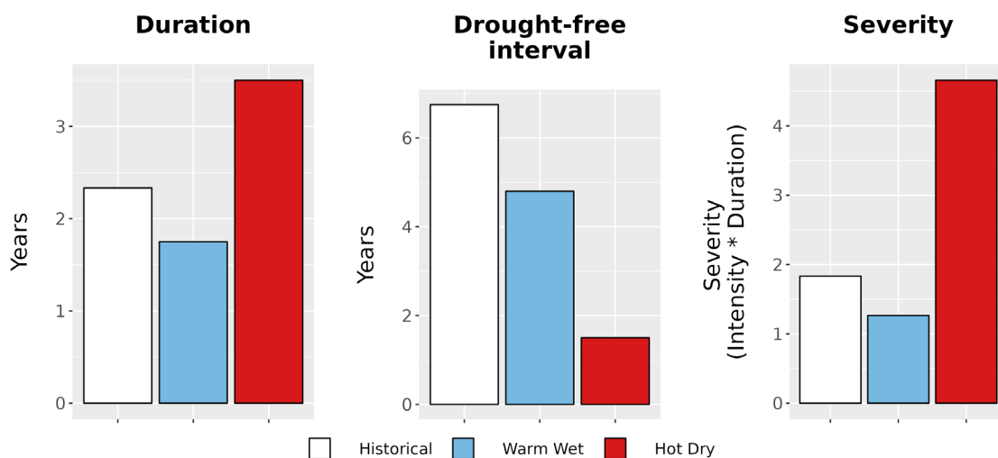
Figure 8. Drought metrics for CANE. (Left) Average drought duration (years) historically (1979-2012) and under each climate future. (Middle) Average drought return interval (years), indicating the expected amount of time between periods of drought, historically and under each climate future. (Right) Average drought severity, a measure of drought intensity multiplied by duration, historically and under each climate future.
