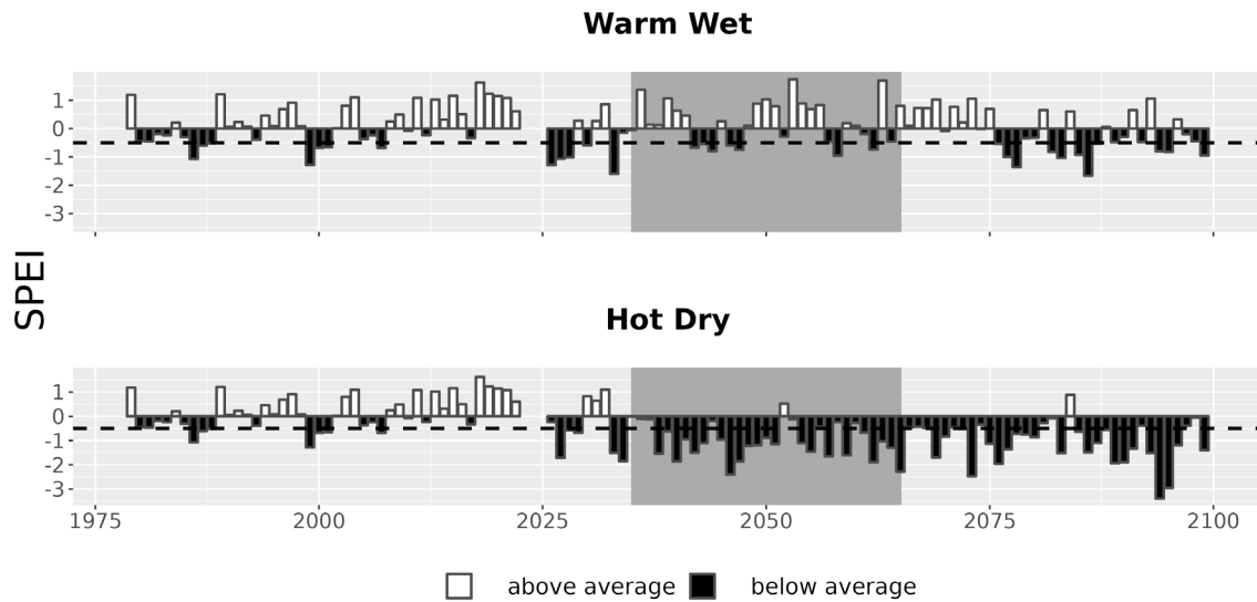
Figure 7. Drought metrics for CANE. Drought index (SPEI; units = standard deviations from historical) timeseries for each climate future. Below-average SPEI (black bars) indicates dry conditions. The dotted line (SPEI = -0.5) indicates drought conditions.
