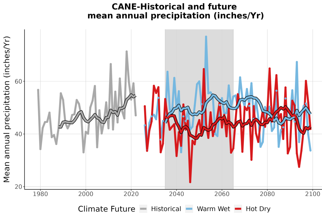
Figure 4. This graph compares observed average annual precipitation at CANE (inches/year) (1979-2022) with projected average annual precipitation for the two climate futures over the period 2023-2099. The historically observed data is shown in gray, the Warm Wet climate future in blue, and the Hot Dry climate future in red. The smooth line running through each projection is the 10-year running average for historical observations and future projections. The gray-shaded area represents the time period that was averaged (2035-2065) to summarize future projections for the year 2050 (Appendix 1).
