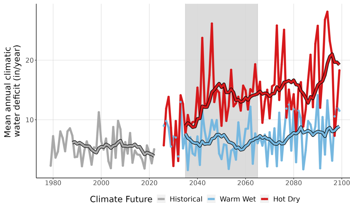
Figure 9. This line graph compares observed climatic water deficit at CANE (inches/year) (1979-2022) with projected climatic water deficit for the two climate futures over the period 2023-2099. The historical observation data is shown in gray, the Warm Wet climate future in blue, and the Hot Dry climate future in red. The smooth line running through each projection is the 10-year running average for historical observations and future projections. Gray-shaded area represents the time period that was averaged (2035-2065) to summarize future projections for the year 2050.
