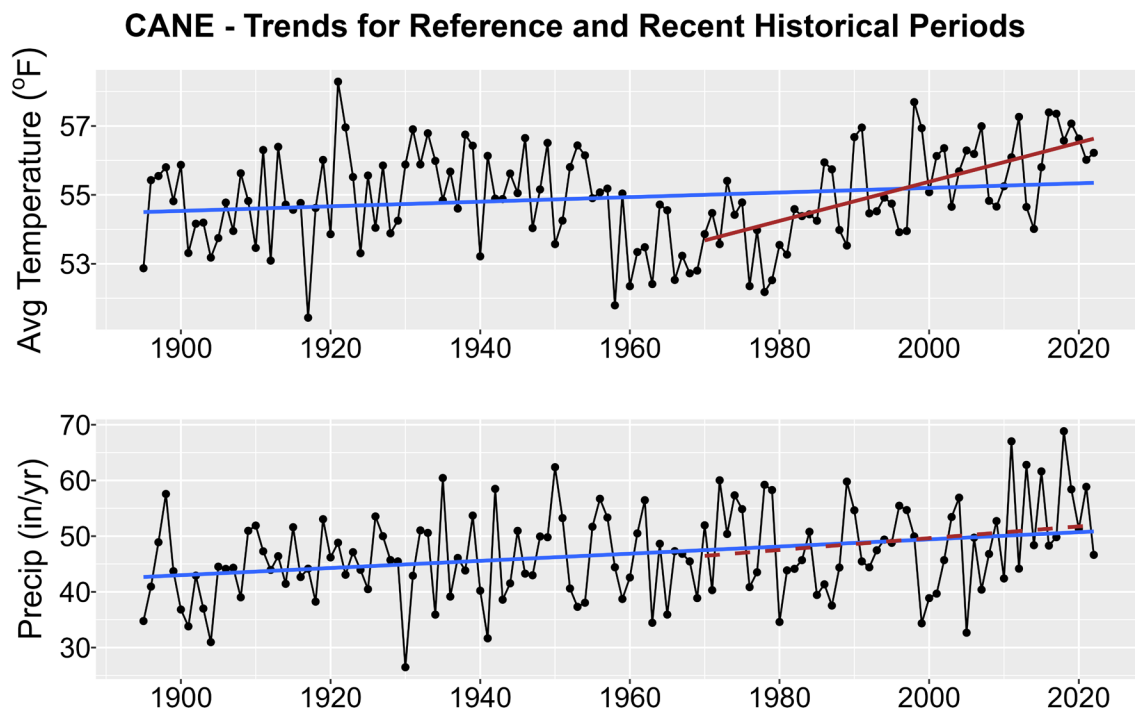
Figure 1. Historical trends in annual average temperature (upper plot) and annual total precipitation (lower plot) for CANE from 1895-2022. Black points show yearly values while blue lines are linear regressions for the entire period record and red lines for 1970-2022 trends. Solid lines are significant trends (i.e., p < 0.05 ); dashed lines are not statistically significant.
