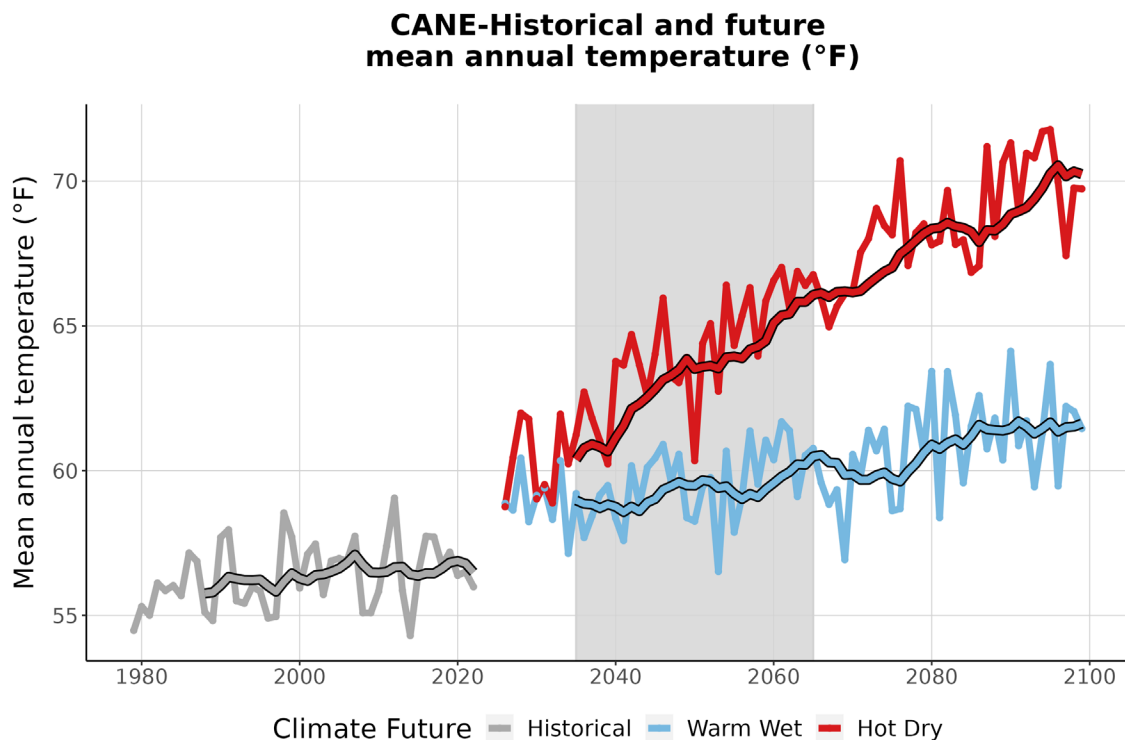
Figure 3. This graph compares observed average annual temperature at CANE (°F) (1979-2022) with projected average annual temperature for the two climate futures over the period 2023-2099. The historically observed data
