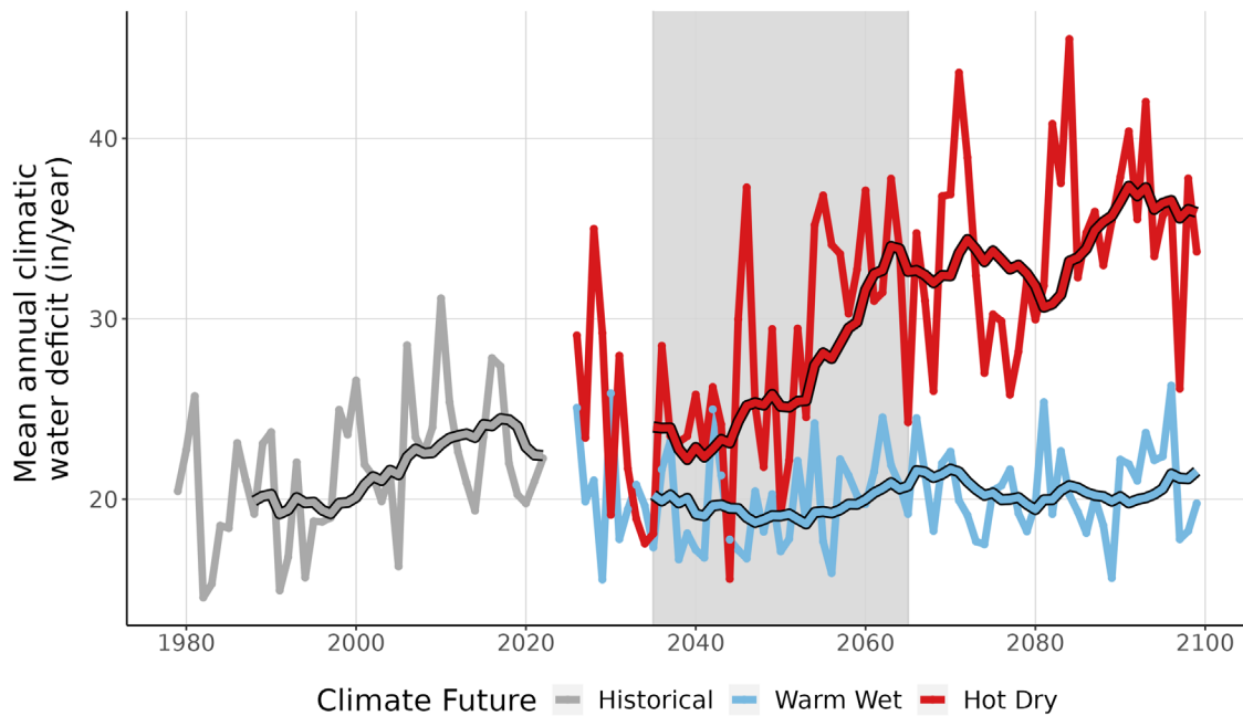
Figure 9. This line graph compares observed climatic water deficit at CANA (inches/year) (1979-2022) with projected climatic water deficit for the two climate futures over the period 2023-2099. The historical observation data is shown in gray, the Warm Wet climate future in blue, and the Hot Dry climate future in red. The smooth line running through each projection is the 10-year running average for historical observations and future projections. Gray-shaded area represents the time period that was averaged (2035-2065) to summarize future projections for the year 2050.
