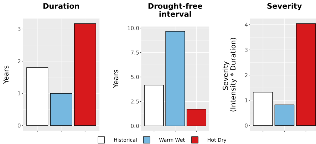
Figure 8. Drought metrics for CANA. (Left) Average drought duration (years) historically (1979-2012) and under each climate future. (Middle) Average drought return interval (years), indicating the expected amount of time between periods of drought, historically and under each climate future. (Right) Average drought severity, a measure of drought intensity multiplied by duration, historically and under each climate future.
