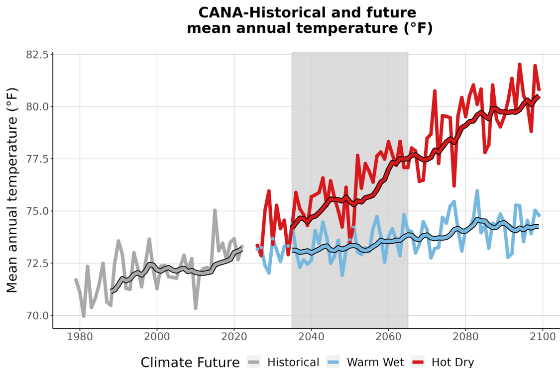
Figure 3. This graph compares observed average annual temperature at CANA (°F) (1979-2022) with projected average annual temperature for the two climate futures over the period 2023-2099. The historically observed data
