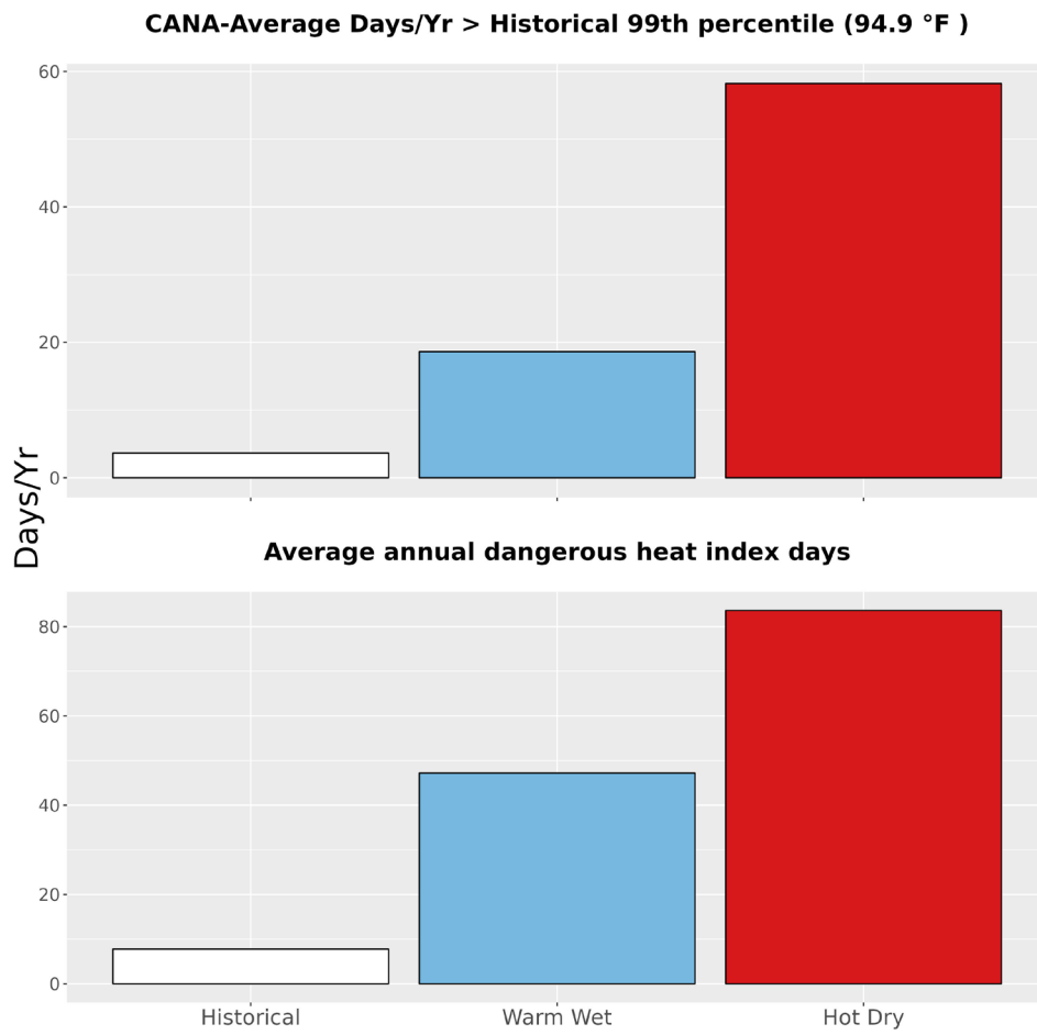
Figure 5. The upper bar graph represents the average number of days annually with temperatures greater than the historical 99th percentile (94.9 °F) historically (1979-2012) and for the two climate futures (2050). The bottom bar graph represents the average annual number of dangerous heat index days historically and for the two climate futures. Dangerous heat index days are days that exceed 105 °F.
