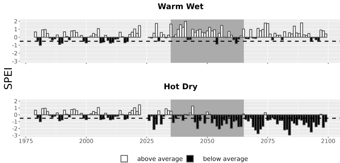
Figure 7. Drought metrics for CANA. Drought index (SPEI; units = standard deviations from historical) timeseries for each climate future. Below-average SPEI (black bars) indicates dry conditions. The dotted line (SPEI = -0.5) indicates drought conditions.
