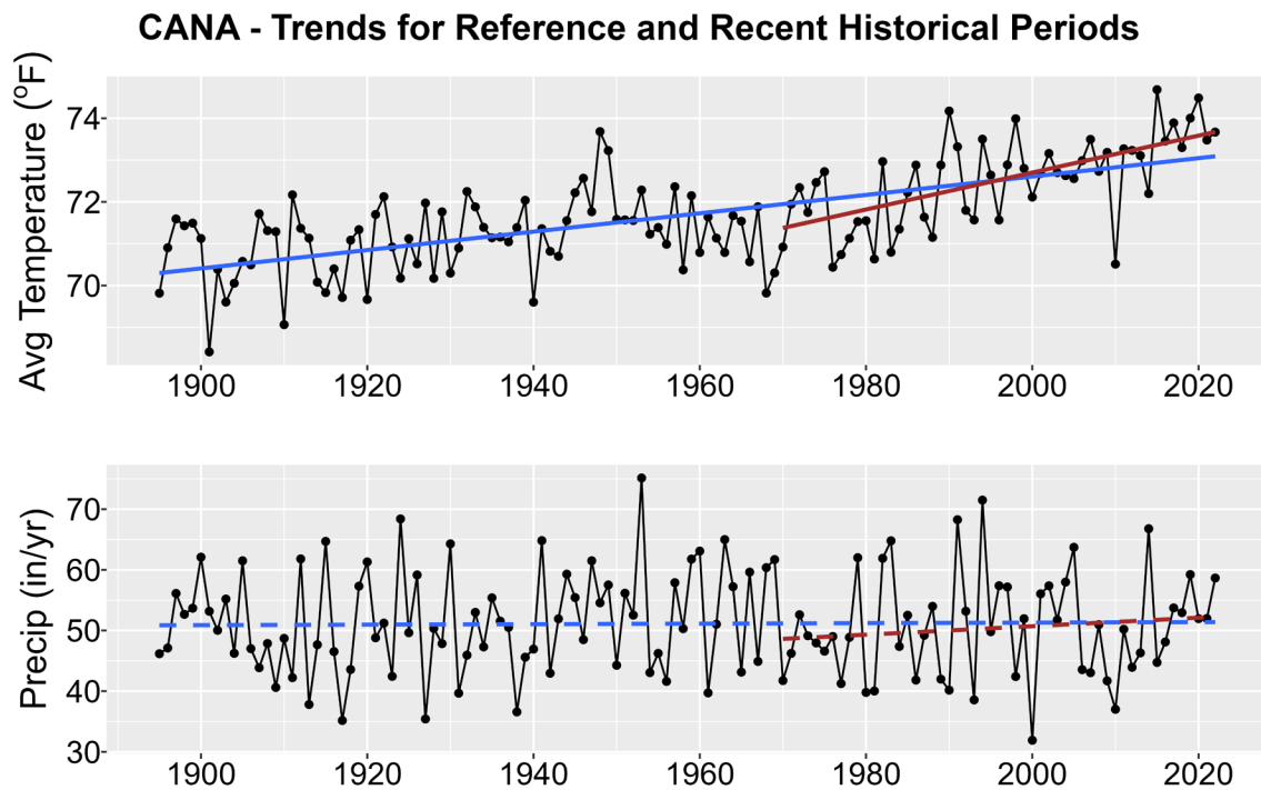
Figure 1. Historical trends in annual average temperature (upper plot) and annual total precipitation (lower plot) for CANA from 1895-2022. Black points show yearly values while blue lines are linear regressions for the entire period record and red lines for 1970-2022 trends. Solid lines are significant trends (i.e., p < 0.05 ); dashed lines are not statistically significant.
