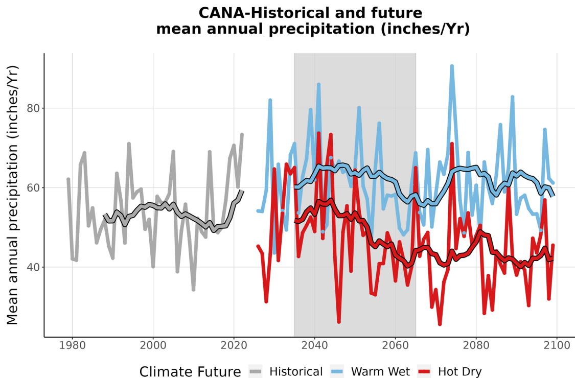
Figure 4. This graph compares observed average annual precipitation at CANA (inches/year) (1979-2022) with projected average annual precipitation for the two climate futures over the period 2023-2099. The historically observed data is shown in gray, the Warm Wet climate future in blue, and the Hot Dry climate future in red. The smooth line running through each projection is the 10-year running average for historical observations and future projections. The gray-shaded area represents the time period that was averaged (2035-2065) to summarize future projections for the year 2050 (Appendix 1).
