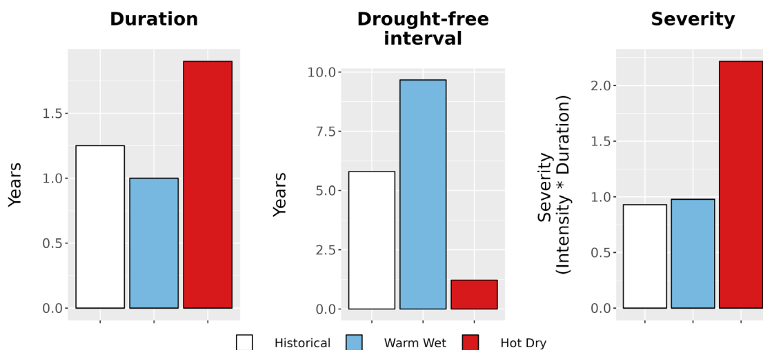
Figure 8. Drought metrics for CALO. (Left) Average drought duration (years) historically (1979-2012) and under each climate future. (Middle) Average drought return interval (years), indicating the expected amount of time between periods of drought, historically and under each climate future. (Right) Average drought severity, a measure of drought intensity multiplied by duration, historically and under each climate future.
