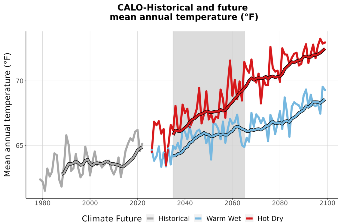
Figure 3. This graph compares observed average annual temperature at CALO (°F) (1979-2022) with projected average annual temperature for the two climate futures over the period 2023-2099. The historically observed data
