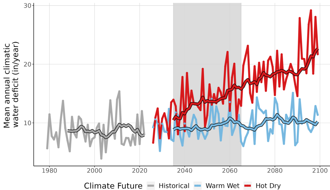
Figure 9. This line graph compares observed climatic water deficit at CALO (inches/year) (1979-2022) with projected climatic water deficit for the two climate futures over the period 2023-2099. The historical observation data is shown in gray, the Warm Wet climate future in blue, and the Hot Dry climate future in red. The smooth line running through each projection is the 10-year running average for historical observations and future projections. Gray-shaded area represents the time period that was averaged (2035-2065) to summarize future projections for the year 2050.
