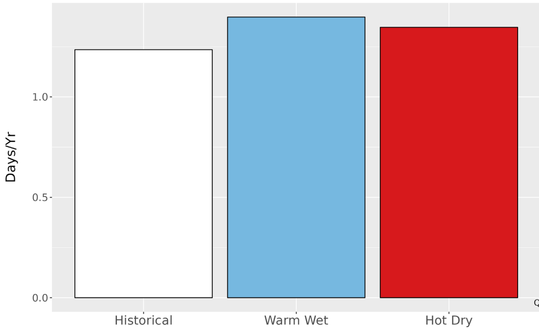
Figure 6. Average number of days annually with precipitation exceeding the 99th percentile (2.6 in.) of precipitation from the historical period 1979-2012 and for each climate future.
