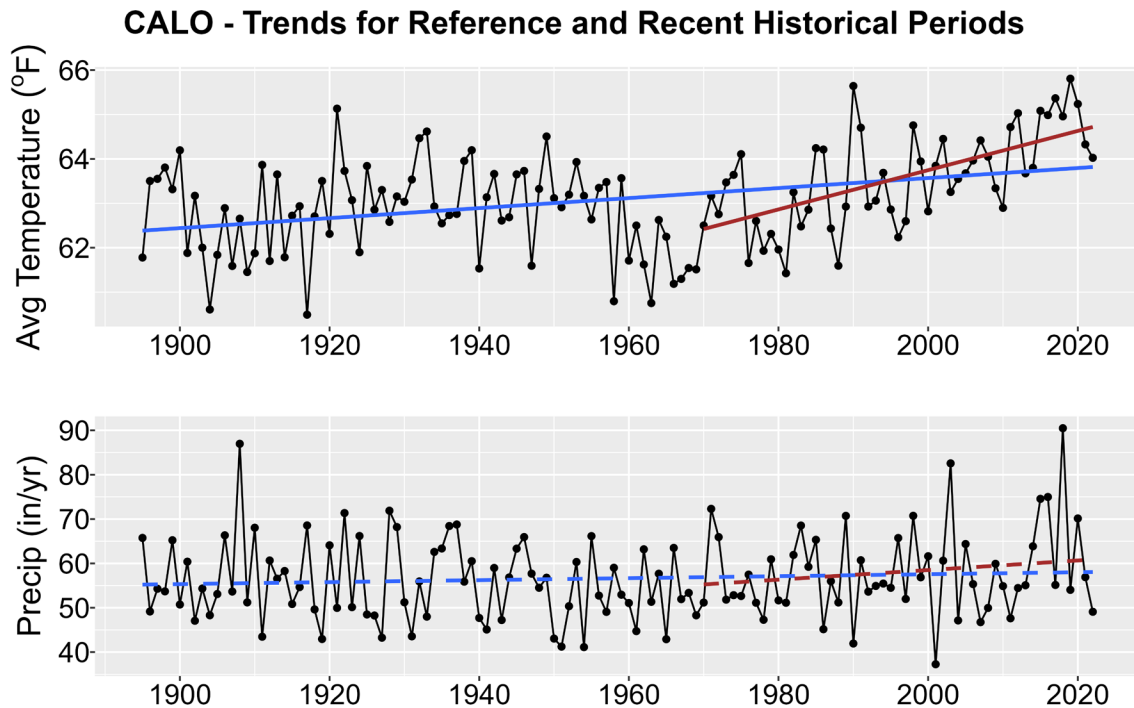
Figure 1. Historical trends in annual average temperature (upper plot) and annual total precipitation (lower plot) for CALO from 1895-2022. Black points show yearly values while blue lines are linear regressions for the entire period record and red lines for 1970-2022 trends. Solid lines are significant trends (i.e., p < 0.05 ); dashed lines are not statistically significant.
