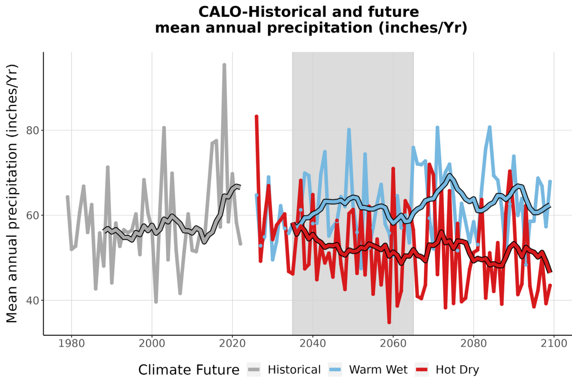
Figure 4. This graph compares observed average annual precipitation at CALO (inches/year) (1979-2022) with projected average annual precipitation for the two climate futures over the period 2023-2099. The historically observed data is shown in gray, the Warm Wet climate future in blue, and the Hot Dry climate future in red. The smooth line running through each projection is the 10-year running average for historical observations and future projections. The gray-shaded area represents the time period that was averaged (2035-2065) to summarize future projections for the year 2050 (Appendix 1).
