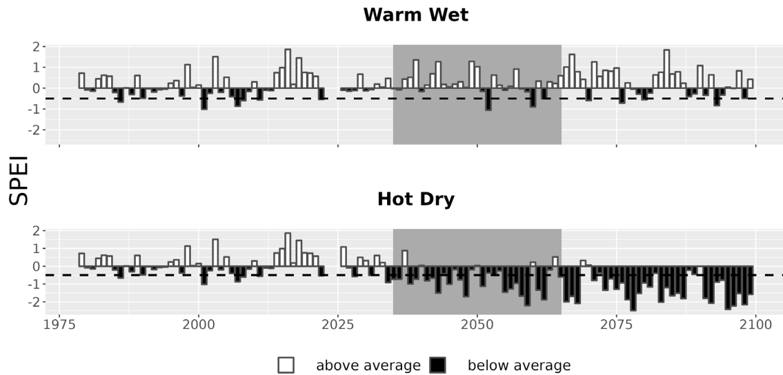
Figure 7. Drought metrics for CALO. Drought index (SPEI; units = standard deviations from historical) timeseries for each climate future. Below-average SPEI (black bars) indicates dry conditions. The dotted line (SPEI = -0.5) indicates drought conditions.
