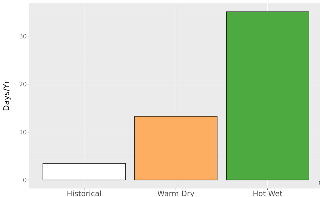
Figure 5. Metrics of extreme temperature at CACO. The bar graph represents the average number of days annually with temperatures greater than the historical 99th percentile (83.7 °F) historically (1979-2012) and for the two climate futures (2050).
