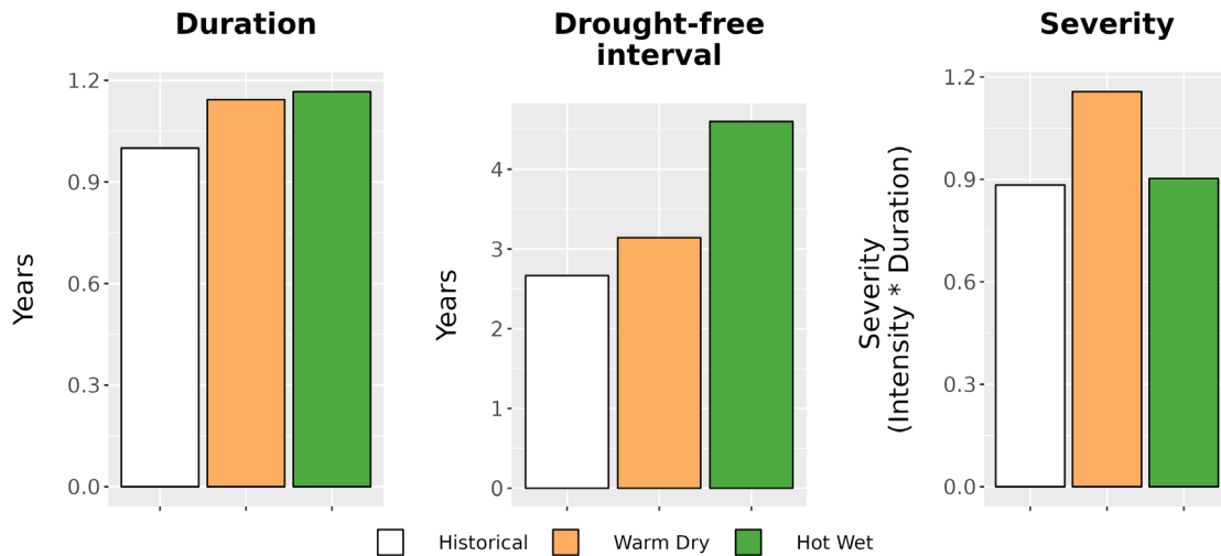
Figure 8. Drought metrics for CACO. (Left) Average drought duration (years) historically (1979-2012) and under each climate future. (Middle) Average drought return interval (years), indicating the expected amount of time between periods of drought, historically and under each climate future. (Right) Average drought severity, a measure of drought intensity multiplied by duration, historically and under each climate future.
