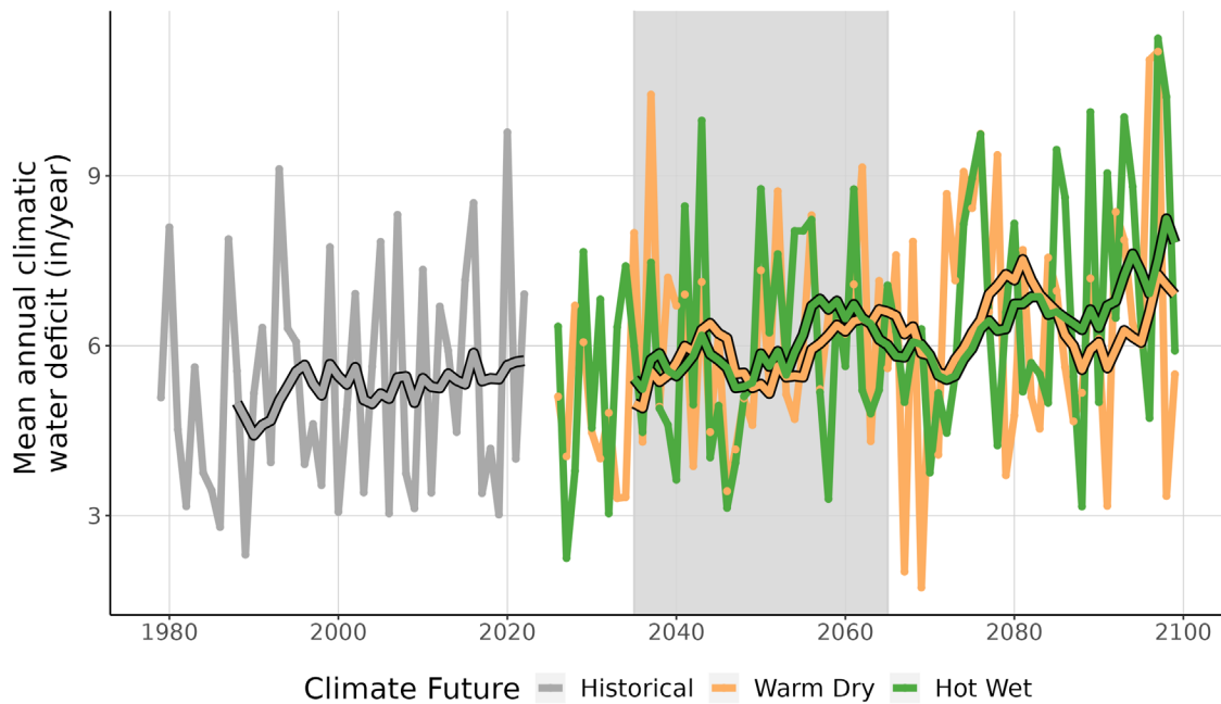
Figure 9. This line graph compares observed climatic water deficit at CACO (inches/year) (1979-2022) with projected climatic water deficit for the two climate futures over the period 2023-2099. The historical observation data is shown in gray, the Warm Dry climate future in orange, and the Hot Wet climate future in green. The smooth line running through each projection is the 10-year running average for historical observations and future projections. Gray-shaded area represents the time period that was averaged (2035-2065) to summarize future projections for the year 2050.
