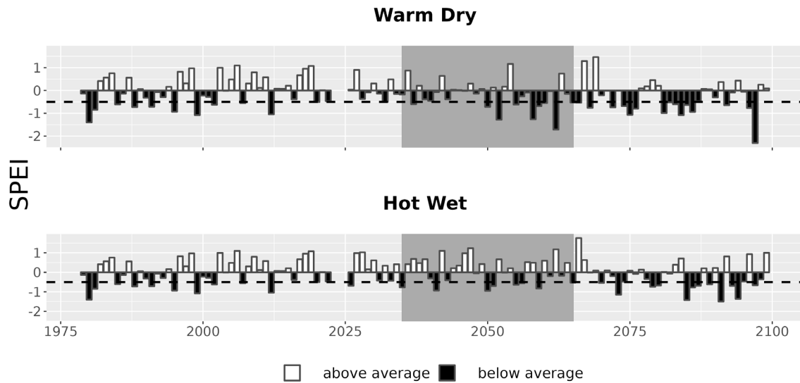
Figure 7. Drought metrics for CACO. Drought index (SPEI; units = standard deviations from historical) timeseries for each climate future. Below-average SPEI (black bars) indicates dry conditions. The dotted line (SPEI = -0.5) indicates drought conditions.
