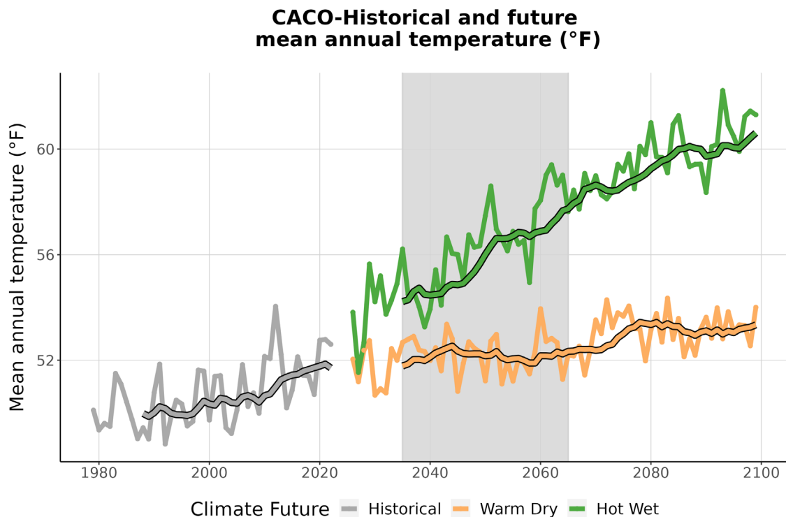
Figure 3. This graph compares observed average annual temperature at CACO (°F) (1979-2022) with projected average annual temperature for the two climate futures over the period 2023-2099. The historically observed data
