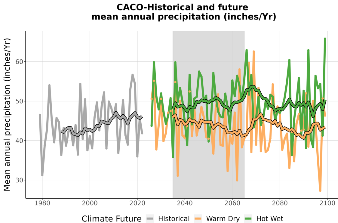
Figure 4. This graph compares observed average annual precipitation at CACO (inches/year) (1979-2022) with projected average annual precipitation for the two climate futures over the period 2023-2099. The historically observed data is shown in gray, the Warm Dry climate future in orange, and the Hot Wet climate future in green. The smooth line running through each projection is the 10-year running average for historical observations and future projections. The gray-shaded area represents the time period that was averaged (2035-2065) to summarize future projections for the year 2050 (Appendix 1).
