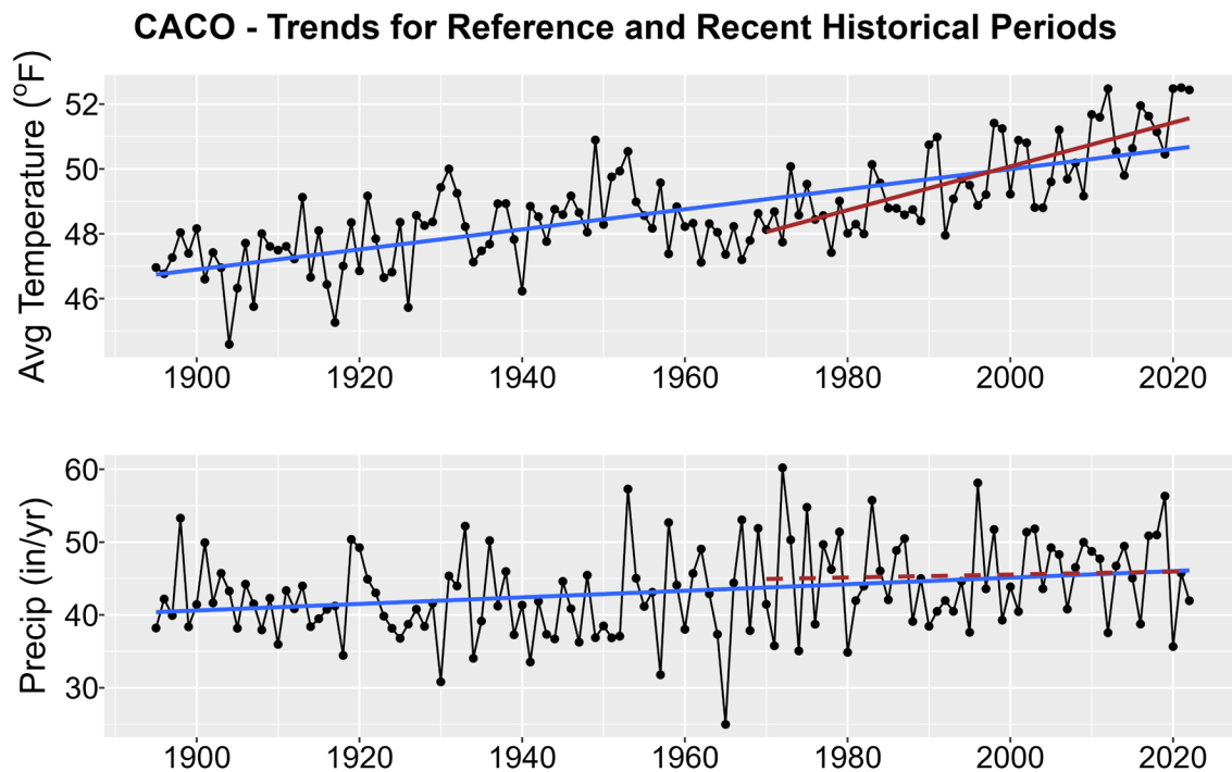
Figure 1. Historical trends in annual average temperature (upper plot) and annual total precipitation (lower plot) for CACO from 1895-2022. Black points show yearly values while blue lines are linear regressions for the entire period record and red lines for 1970-2022 trends. Solid lines are significant trends (i.e., p < 0.05 ); dashed lines are not statistically significant.
