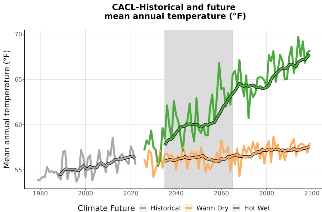
Figure 3. This graph compares observed average annual temperature at CACL (°F) (1979-2022) with projected average annual temperature for the two climate futures over the period 2023-2099. The historically observed data is shown in gray, the Warm Dry climate future in orange, and the Hot Wet climate future in green. The smooth line
