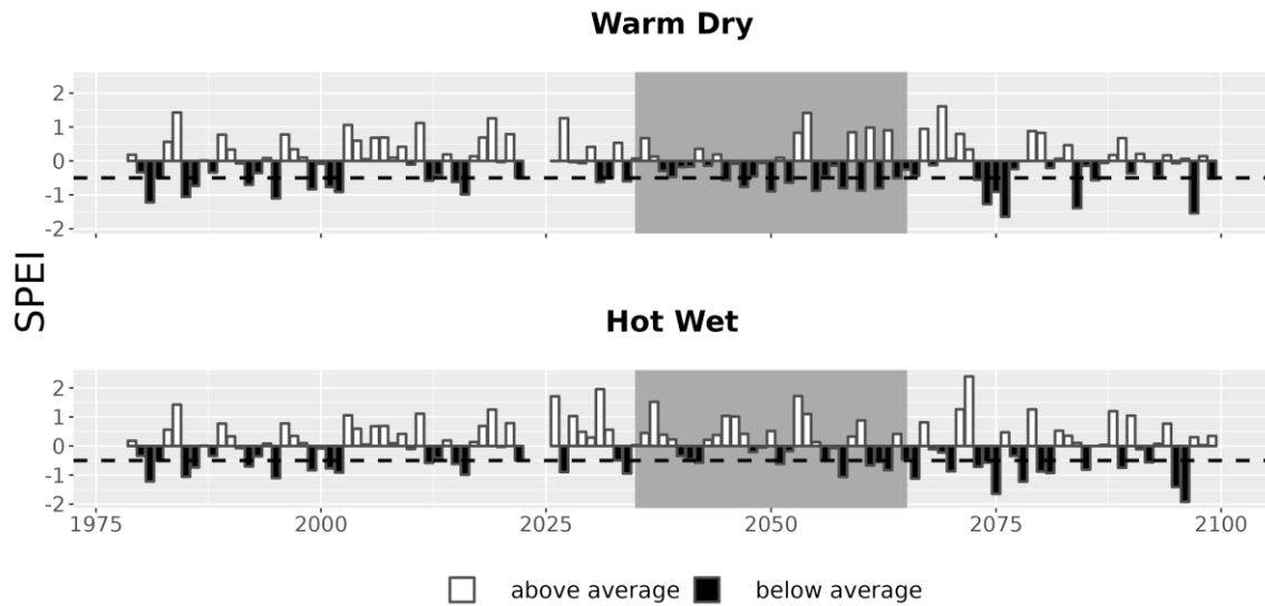
Figure 7. Drought metrics for CACL. Drought index (SPEI; units = standard deviations from historical) timeseries for each climate future. Below-average SPEI (black bars) indicates dry conditions. The dotted line (SPEI = -0.5) indicates drought conditions.
