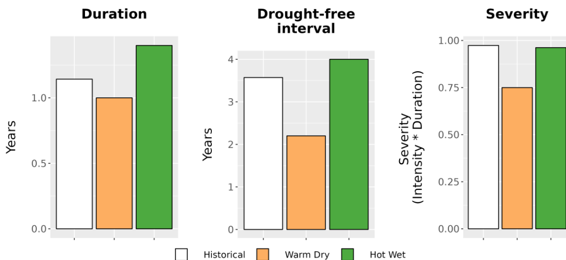
Figure 8. Drought metrics for CACL. (Left) Average drought duration (years) historically (1979-2012) and under each climate future. (Middle) Average drought return interval (years), indicating the expected amount of time between periods of drought, historically and under each climate future. (Right) Average drought severity, a measure of drought intensity multiplied by duration, historically and under each climate future.
