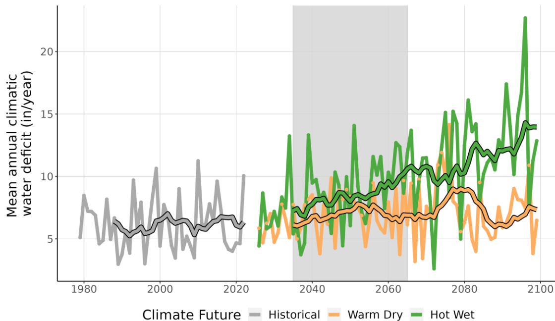
Figure 9. This line graph compares observed climatic water deficit at CACL (inches/year) (1979-2022) with projected climatic water deficit for the two climate futures over the period 2023-2099. The historical observation data is shown in gray, the Warm Dry climate future in orange, and the Hot Wet climate future in green. The smooth line running through each projection is the 10-year running average for historical observations and future projections. Gray-shaded area represents the time period that was averaged (2035-2065) to summarize future projections for the year 2050.
