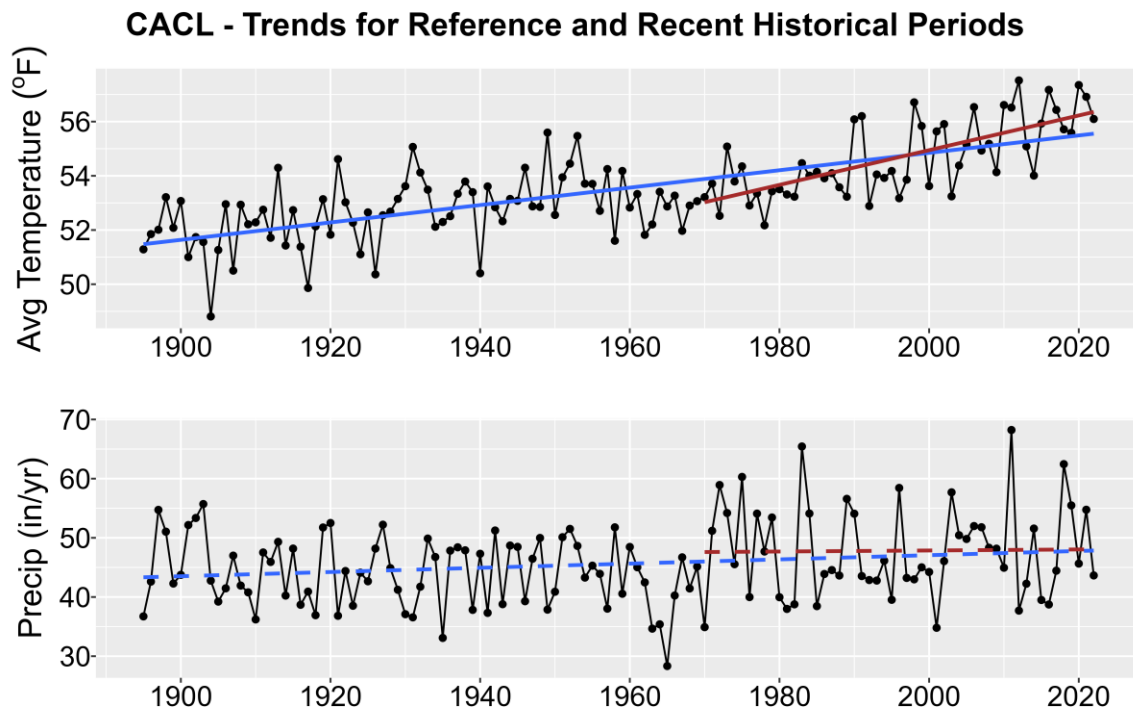
Figure 1. Historical trends in annual average temperature (upper plot) and annual total precipitation (lower plot) for CACL from 1895-2022. Black points show yearly values while blue lines are linear regressions for the entire period record and red lines for 1970-2022 trends. Solid lines are significant trends (i.e., p < 0.05 ); dashed lines are not statistically significant.
