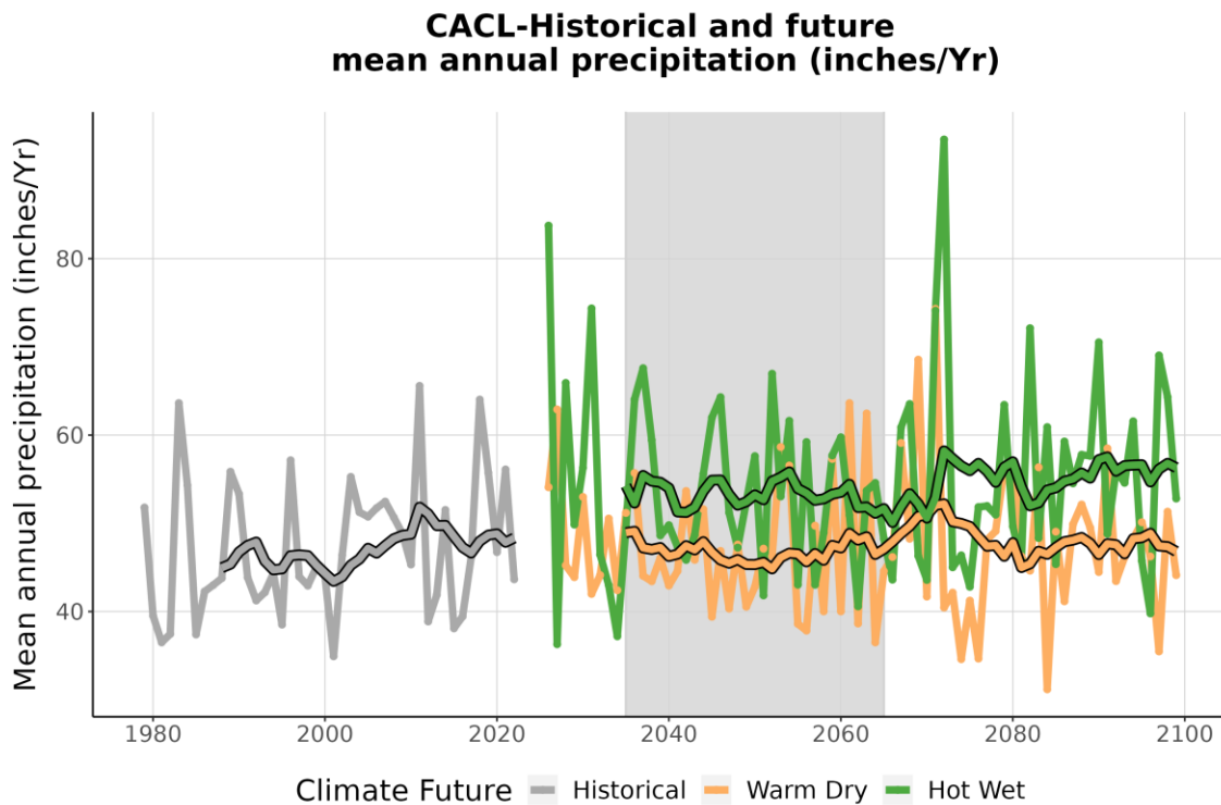
Figure 4. This graph compares observed average annual precipitation at CACL (inches/year) (1979-2022) with projected average annual precipitation for the two climate futures over the period 2023-2099. The historically observed data is shown in gray, the Warm Dry climate future in orange, and the Hot Wet climate future in green. The smooth line running through each projection is the 10-year running average for historical observations and future projections. The gray-shaded area represents the time period that was averaged (2035-2065) to summarize future projections for the year 2050 (Appendix 1).
