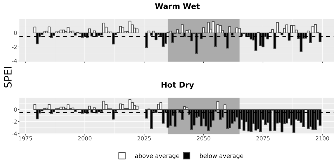
Figure 7. Drought metrics for BUFF. Drought index (SPEI; units = standard deviations from historical) timeseries for each climate future. Below-average SPEI (black bars) indicates dry conditions. The dotted line (SPEI = -0.5) indicates drought conditions.
