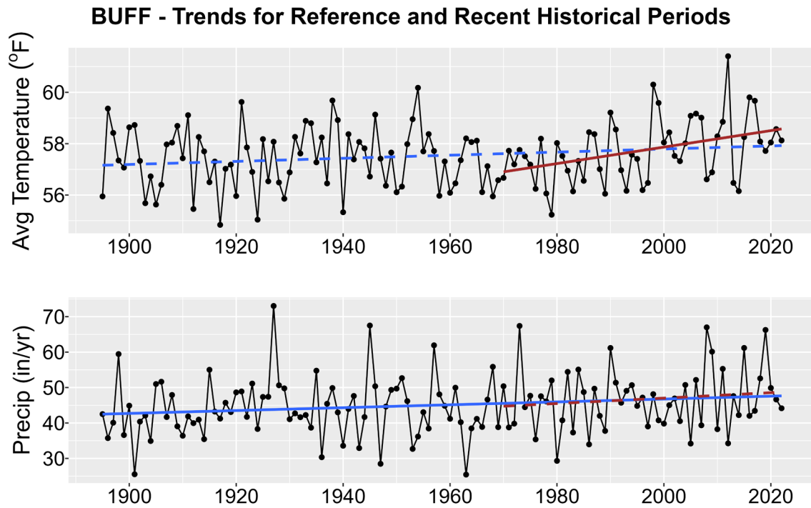
Figure 1. Historical trends in annual average temperature (upper plot) and annual total precipitation (lower plot) for BUFF from 1895-2022. Black points show yearly values while blue lines are linear regressions for the entire period record and red lines for 1970-2022 trends. Solid lines are significant trends (i.e., p < 0.05 ); dashed lines are not statistically significant.
