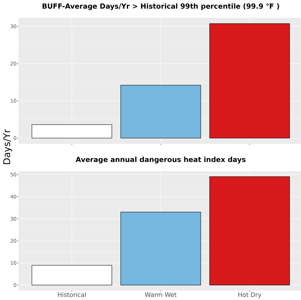
Figure 5. The upper bar graph represents the average number of days annually with temperatures greater than the historical 99th percentile (99.9 °F) historically (1979-2012) and for the two climate futures (2050). The bottom bar graph represents the average annual number of dangerous heat index days historically and for the two climate futures. Dangerous heat index days are days that exceed 105 °F.
