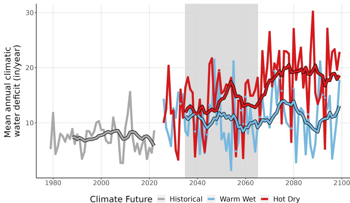
Figure 9. This line graph compares observed climatic water deficit at BUFF (inches/year) (1979-2022) with projected climatic water deficit for the two climate futures over the period 2023-2099. The historical observation data is shown in gray, the Warm Wet climate future in blue, and the Hot Dry climate future in red. The smooth line running through each projection is the 10-year running average for historical observations and future projections. Gray-shaded area represents the time period that was averaged (2035-2065) to summarize future projections for the year 2050.
