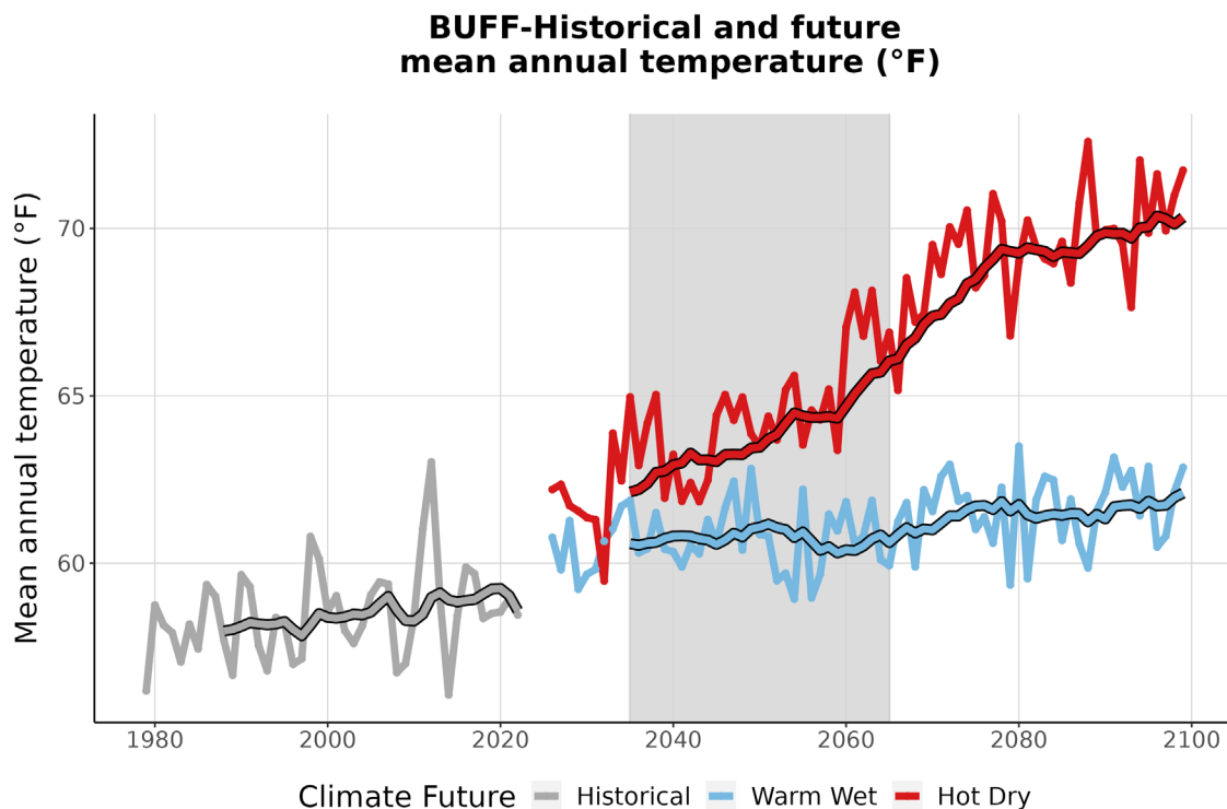
Figure 3. This graph compares observed average annual temperature at BUFF (°F) (1979-2022) with projected average annual temperature for the two climate futures over the period 2023-2099. The historically observed data
