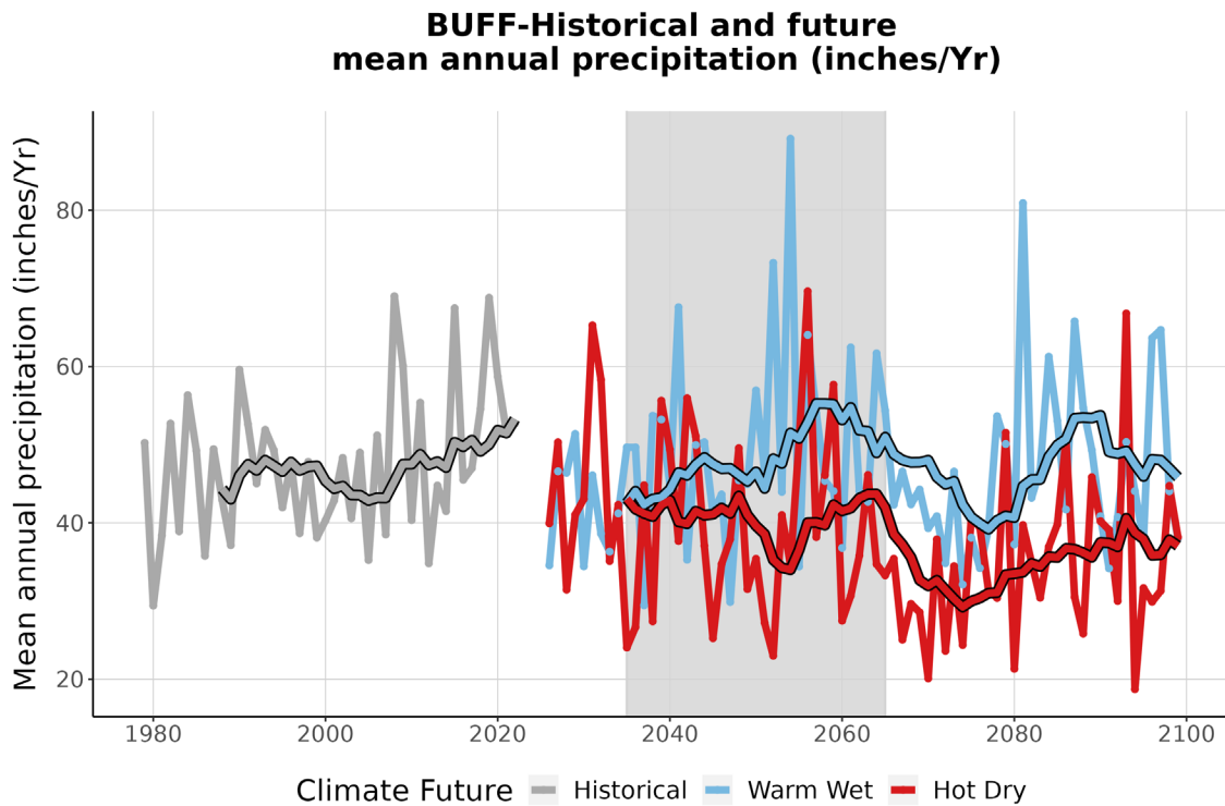
Figure 4. This graph compares observed average annual precipitation at BUFF (inches/year) (1979-2022) with projected average annual precipitation for the two climate futures over the period 2023-2099. The historically observed data is shown in gray, the Warm Wet climate future in blue, and the Hot Dry climate future in red. The smooth line running through each projection is the 10-year running average for historical observations and future projections. The gray-shaded area represents the time period that was averaged (2035-2065) to summarize future projections for the year 2050 (Appendix 1).
