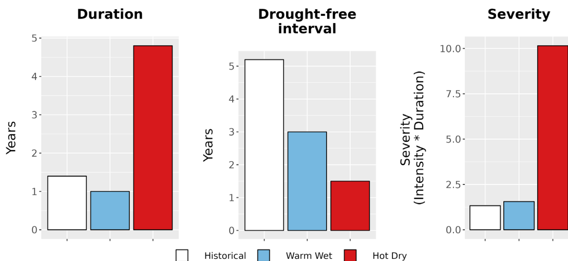
Figure 8. Drought metrics for BUFF. (Left) Average drought duration (years) historically (1979-2012) and under each climate future. (Middle) Average drought return interval (years), indicating the expected amount of time between periods of drought, historically and under each climate future. (Right) Average drought severity, a measure of drought intensity multiplied by duration, historically and under each climate future.
