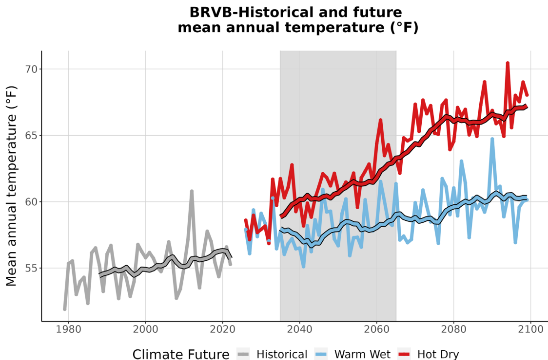
Figure 3. This graph compares observed average annual temperature at BRVB (°F) (1979-2022) with projected average annual temperature for the two climate futures over the period 2023-2099. The historically observed data
