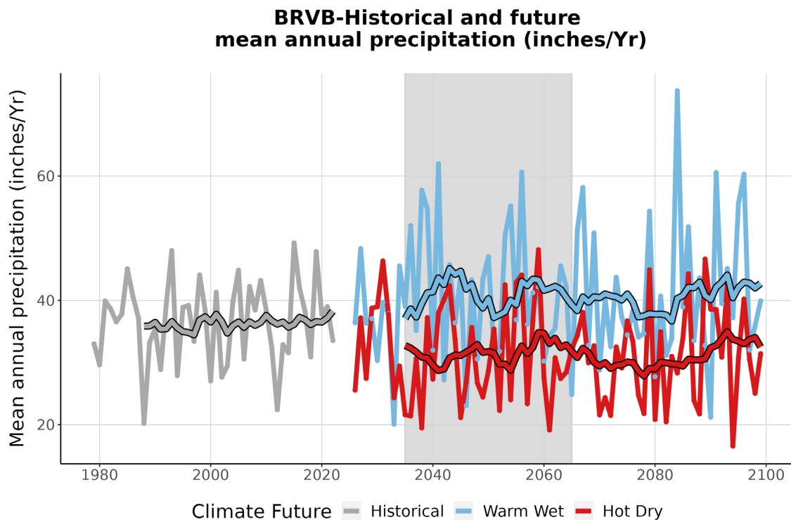
Figure 4. This graph compares observed average annual precipitation at BRVB (inches/year) (1979-2022) with projected average annual precipitation for the two climate futures over the period 2023-2099. The historically observed data is shown in gray, the Warm Wet climate future in blue, and the Hot Dry climate future in red. The smooth line running through each projection is the 10-year running average for historical observations and future projections. The gray-shaded area represents the time period that was averaged (2035-2065) to summarize future projections for the year 2050 (Appendix 1).
