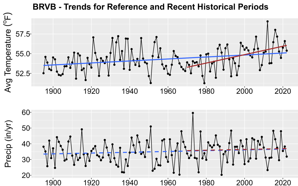
Figure 1. Historical trends in annual average temperature (upper plot) and annual total precipitation (lower plot) for BRVB from 1895-2022. Black points show yearly values while blue lines are linear regressions for the entire period record and red lines for 1970-2022 trends. Solid lines are significant trends (i.e., p < 0.05 ); dashed lines are not statistically significant.
