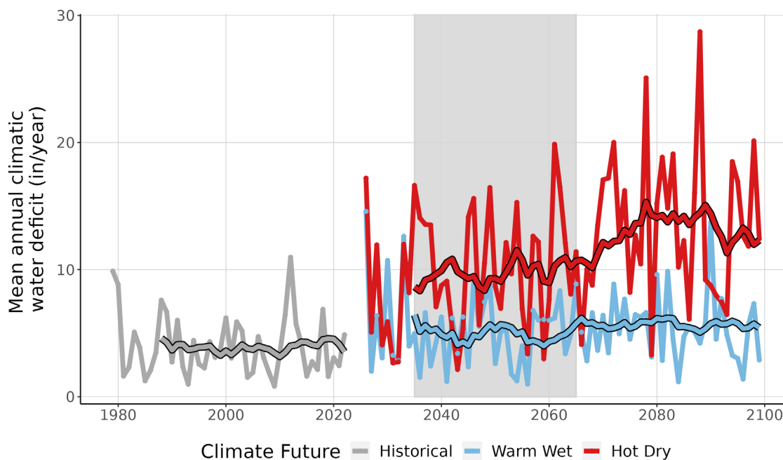
Figure 9. This line graph compares observed climatic water deficit at BRVB (inches/year) (1979-2022) with projected climatic water deficit for the two climate futures over the period 2023-2099. The historical observation data is shown in gray, the Warm Wet climate future in blue, and the Hot Dry climate future in red. The smooth line running through each projection is the 10-year running average for historical observations and future projections. Gray-shaded area represents the time period that was averaged (2035-2065) to summarize future projections for the year 2050.
