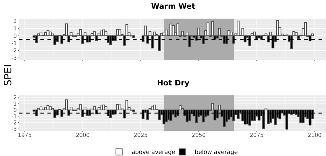
Figure 7. Drought metrics for BRVB. Drought index (SPEI; units = standard deviations from historical) timeseries for each climate future. Below-average SPEI (black bars) indicates dry conditions. The dotted line (SPEI = -0.5) indicates drought conditions.
