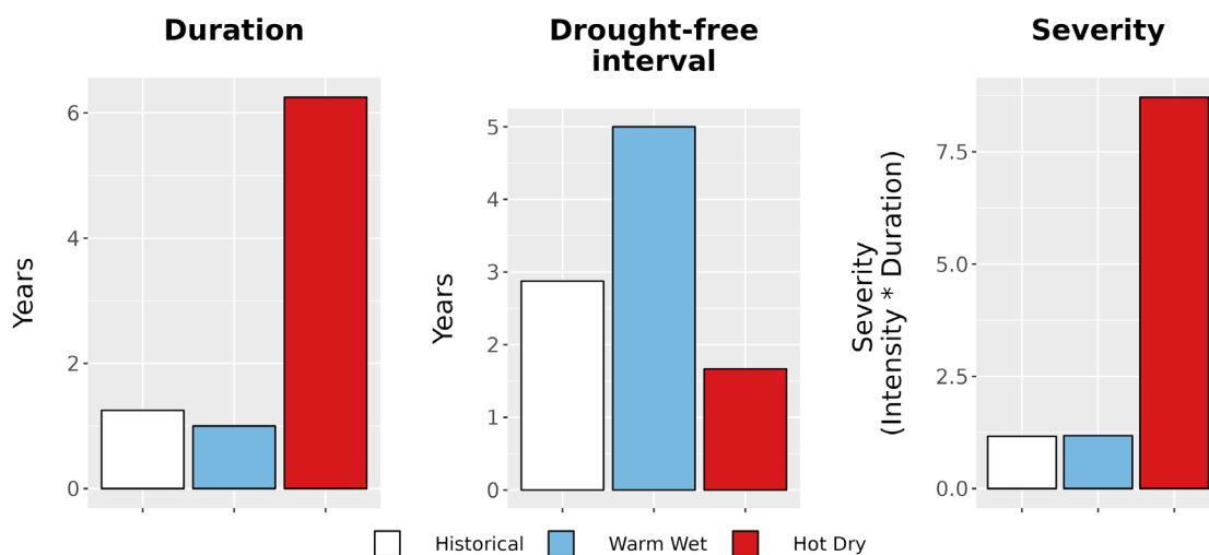
Figure 8. Drought metrics for BRVB. (Left) Average drought duration (years) historically (1979-2012) and under each climate future. (Middle) Average drought return interval (years), indicating the expected amount of time between periods of drought, historically and under each climate future. (Right) Average drought severity, a measure of drought intensity multiplied by duration, historically and under each climate future.
