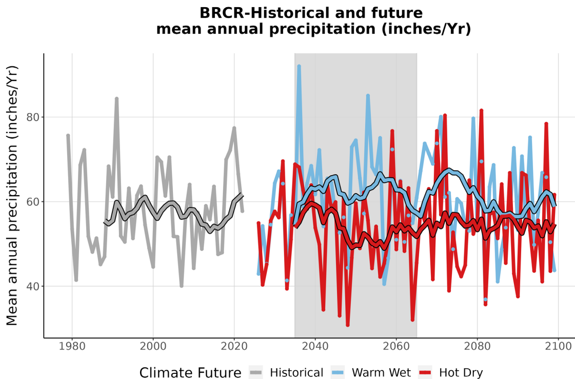
Figure 4. This graph compares observed average annual precipitation at BRCR (inches/year) (1979-2022) with projected average annual precipitation for the two climate futures over the period 2023-2099. The historically observed data is shown in gray, the Warm Wet climate future in blue, and the Hot Dry climate future in red. The smooth line running through each projection is the 10-year running average for historical observations and future projections. The gray-shaded area represents the time period that was averaged (2035-2065) to summarize future projections for the year 2050 (Appendix 1).
