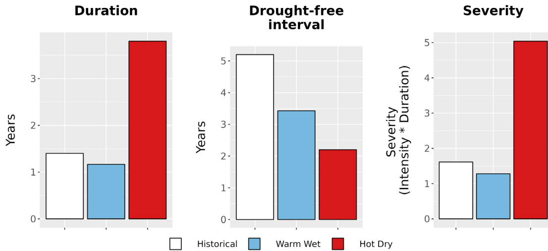
Figure 8. Drought metrics for BRCR. (Left) Average drought duration (years) historically (1979-2012) and under each climate future. (Middle) Average drought return interval (years), indicating the expected amount of time between periods of drought, historically and under each climate future. (Right) Average drought severity, a measure of drought intensity multiplied by duration, historically and under each climate future.
