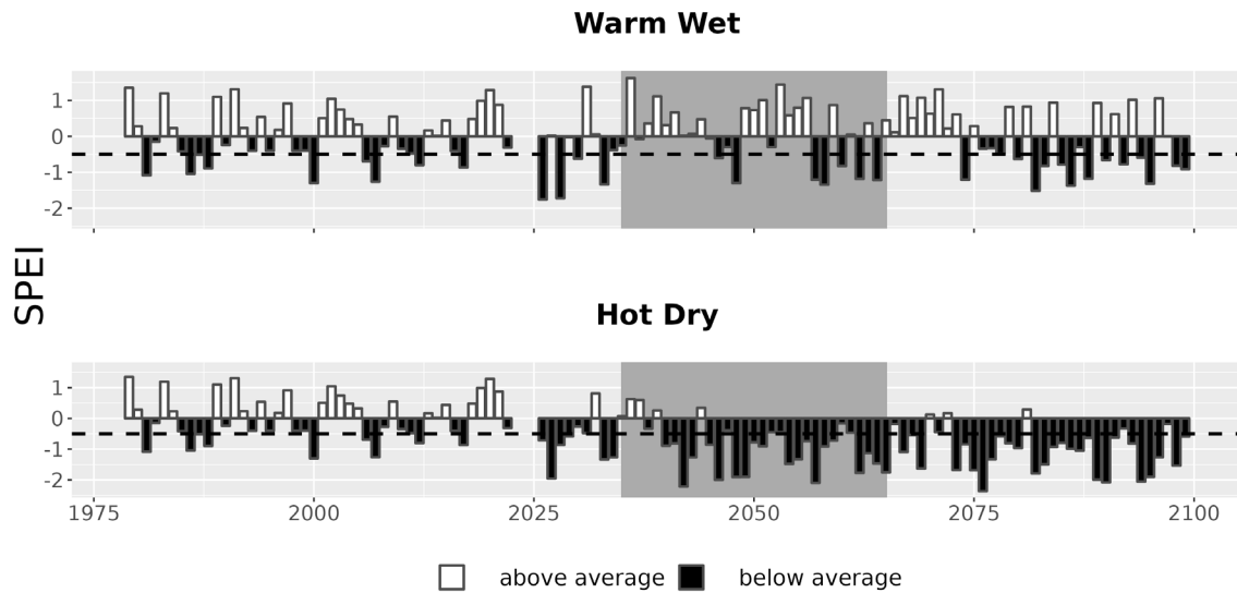
Figure 7. Drought metrics for BRCR. Drought index (SPEI; units = standard deviations from historical) timeseries for each climate future. Below-average SPEI (black bars) indicates dry conditions. The dotted line (SPEI = -0.5) indicates drought conditions.
