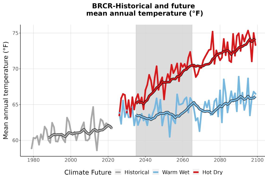
Figure 3. This graph compares observed average annual temperature at BRCR (°F) (1979-2022) with projected average annual temperature for the two climate futures over the period 2023-2099. The historically observed data
