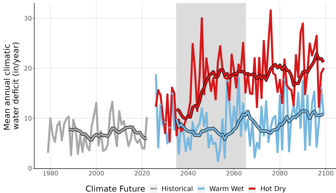
Figure 9. This line graph compares observed climatic water deficit at BRCR (inches/year) (1979-2022) with projected climatic water deficit for the two climate futures over the period 2023-2099. The historical observation data is shown in gray, the Warm Wet climate future in blue, and the Hot Dry climate future in red. The smooth line running through each projection is the 10-year running average for historical observations and future projections. Gray-shaded area represents the time period that was averaged (2035-2065) to summarize future projections for the year 2050.
