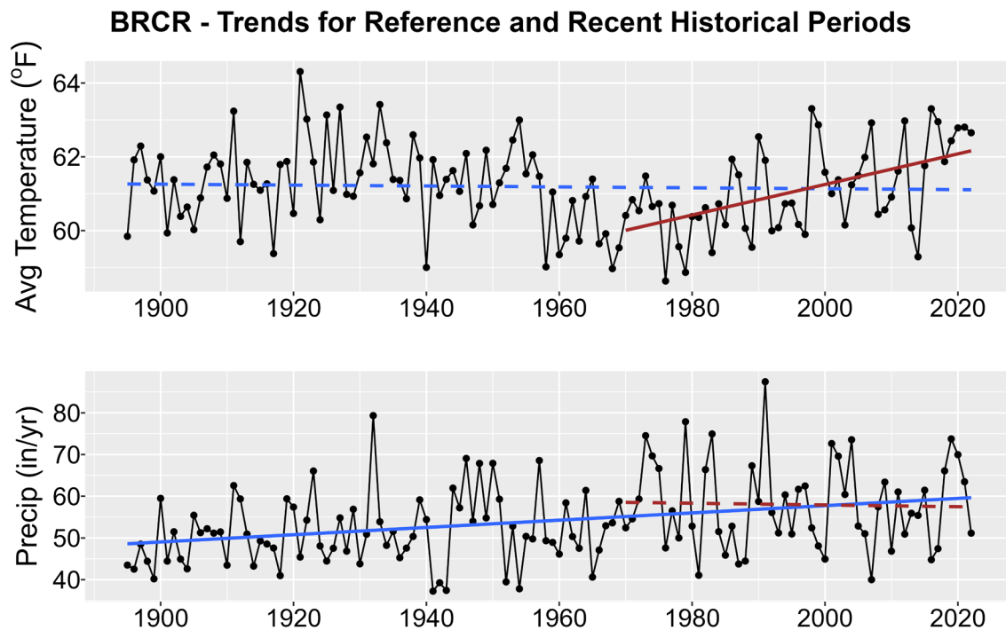
Figure 1. Historical trends in annual average temperature (upper plot) and annual total precipitation (lower plot) for BRCR from 1895-2022. Black points show yearly values while blue lines are linear regressions for the entire period record and red lines for 1970-2022 trends. Solid lines are significant trends (i.e., p < 0.05 ); dashed lines are not statistically significant.
