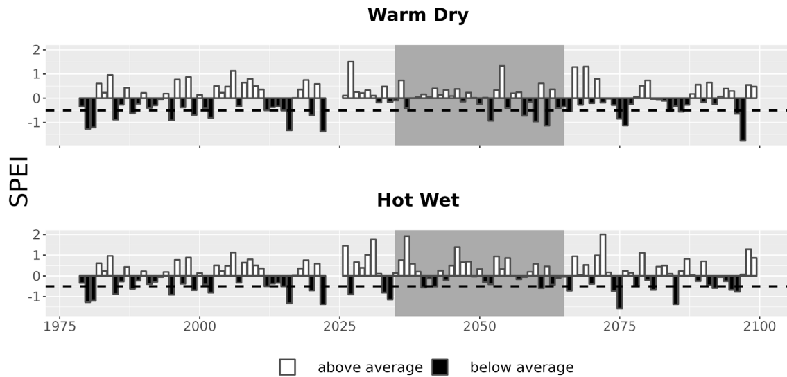
Figure 7. Drought metrics for BOST. Drought index (SPEI; units = standard deviations from historical) timeseries for each climate future. Below-average SPEI (black bars) indicates dry conditions. The dotted line (SPEI = -0.5) indicates drought conditions.
