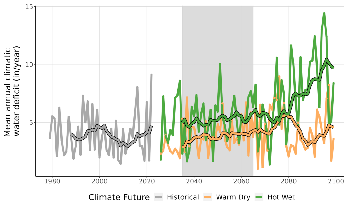
Figure 9. This line graph compares observed climatic water deficit at BOST (inches/year) (1979-2022) with projected climatic water deficit for the two climate futures over the period 2023-2099. The historical observation data is shown in gray, the Warm Dry climate future in orange, and the Hot Wet climate future in green. The smooth line running through each projection is the 10-year running average for historical observations and future projections. Gray-shaded area represents the time period that was averaged (2035-2065) to summarize future projections for the year 2050.
