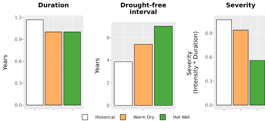
Figure 8. Drought metrics for BOST. (Left) Average drought duration (years) historically (1979-2012) and under each climate future. (Middle) Average drought return interval (years), indicating the expected amount of time between periods of drought, historically and under each climate future. (Right) Average drought severity, a measure of drought intensity multiplied by duration, historically and under each climate future.
