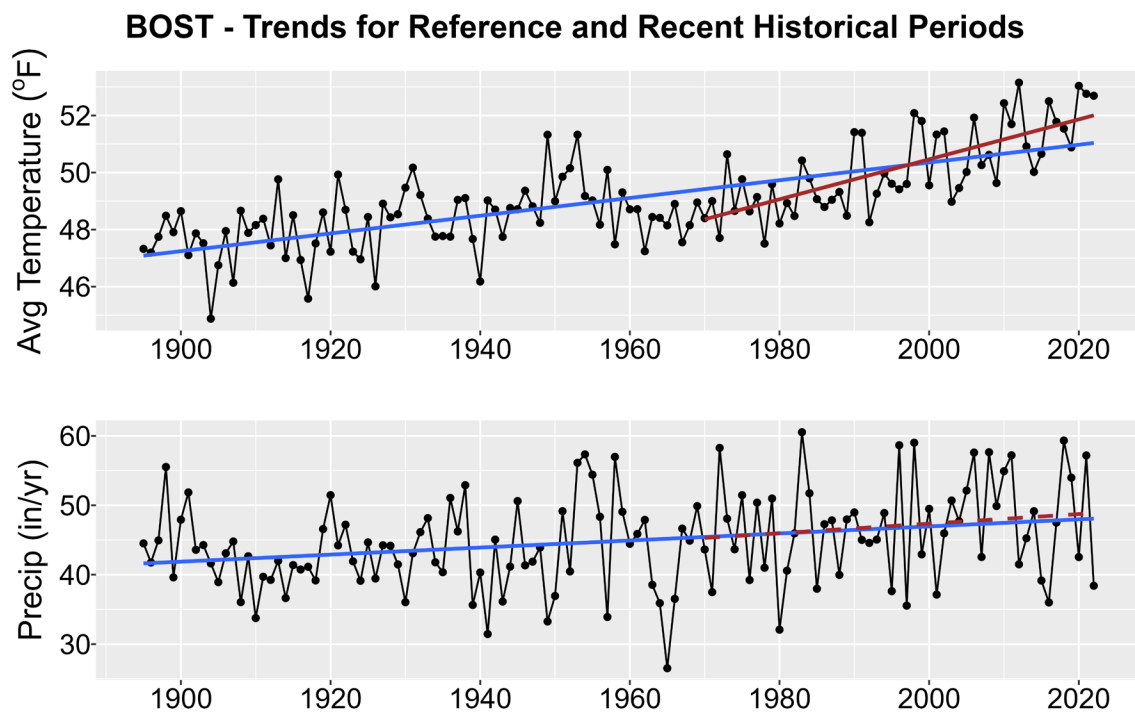
Figure 1. Historical trends in annual average temperature (upper plot) and annual total precipitation (lower plot) for BOST from 1895-2022. Black points show yearly values while blue lines are linear regressions for the entire period record and red lines for 1970-2022 trends. Solid lines are significant trends (i.e., p < 0.05 ); dashed lines are not statistically significant.
