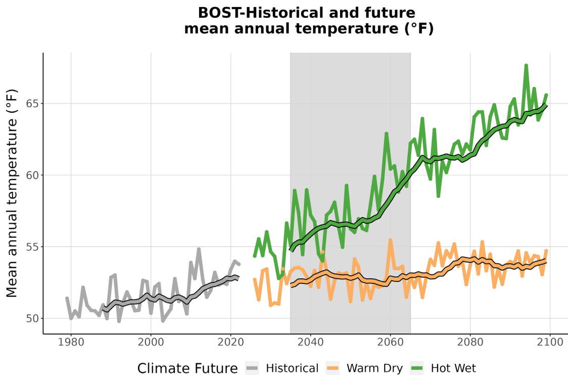
Figure 3. This graph compares observed average annual temperature at BOST (°F) (1979-2022) with projected average annual temperature for the two climate futures over the period 2023-2099. The historically observed data is shown in gray, the Warm Dry climate future in orange, and the Hot Wet climate future in green. The smooth line
