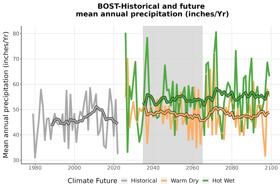
Figure 4. This graph compares observed average annual precipitation at BOST (inches/year) (1979-2022) with projected average annual precipitation for the two climate futures over the period 2023-2099. The historically observed data is shown in gray, the Warm Dry climate future in orange, and the Hot Wet climate future in green. The smooth line running through each projection is the 10-year running average for historical observations and future projections. The gray-shaded area represents the time period that was averaged (2035-2065) to summarize future projections for the year 2050 (Appendix 1).
