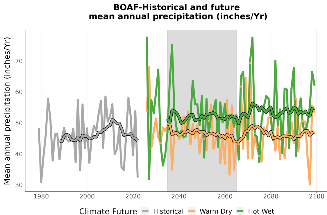
Figure 4. This graph compares observed average annual precipitation at BOAF (inches/year) (1979-2022) with projected average annual precipitation for the two climate futures over the period 2023-2099. The historically observed data is shown in gray, the Warm Dry climate future in orange, and the Hot Wet climate future in green. The smooth line running through each projection is the 10-year running average for historical observations and future projections. The gray-shaded area represents the time period that was averaged (2035-2065) to summarize future projections for the year 2050 (Appendix 1).
