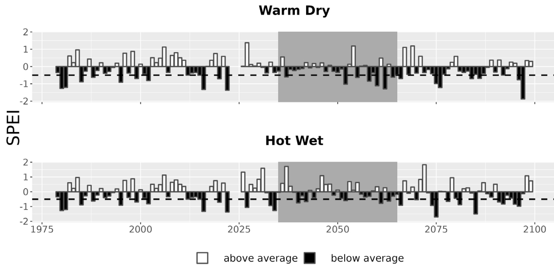
Figure 7. Drought metrics for BOAF. Drought index (SPEI; units = standard deviations from historical) timeseries for each climate future. Below-average SPEI (black bars) indicates dry conditions. The dotted line (SPEI = -0.5) indicates drought conditions.
