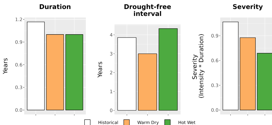
Figure 8. Drought metrics for BOAF. (Left) Average drought duration (years) historically (1979-2012) and under each climate future. (Middle) Average drought return interval (years), indicating the expected amount of time between periods of drought, historically and under each climate future. (Right) Average drought severity, a measure of drought intensity multiplied by duration, historically and under each climate future.
