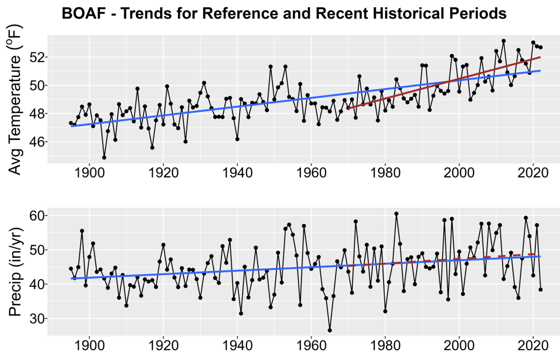
Figure 1. Historical trends in annual average temperature (upper plot) and annual total precipitation (lower plot) for BOAF from 1895-2022. Black points show yearly values while blue lines are linear regressions for the entire period record and red lines for 1970-2022 trends. Solid lines are significant trends (i.e., p < 0.05 ); dashed lines are not statistically significant.
