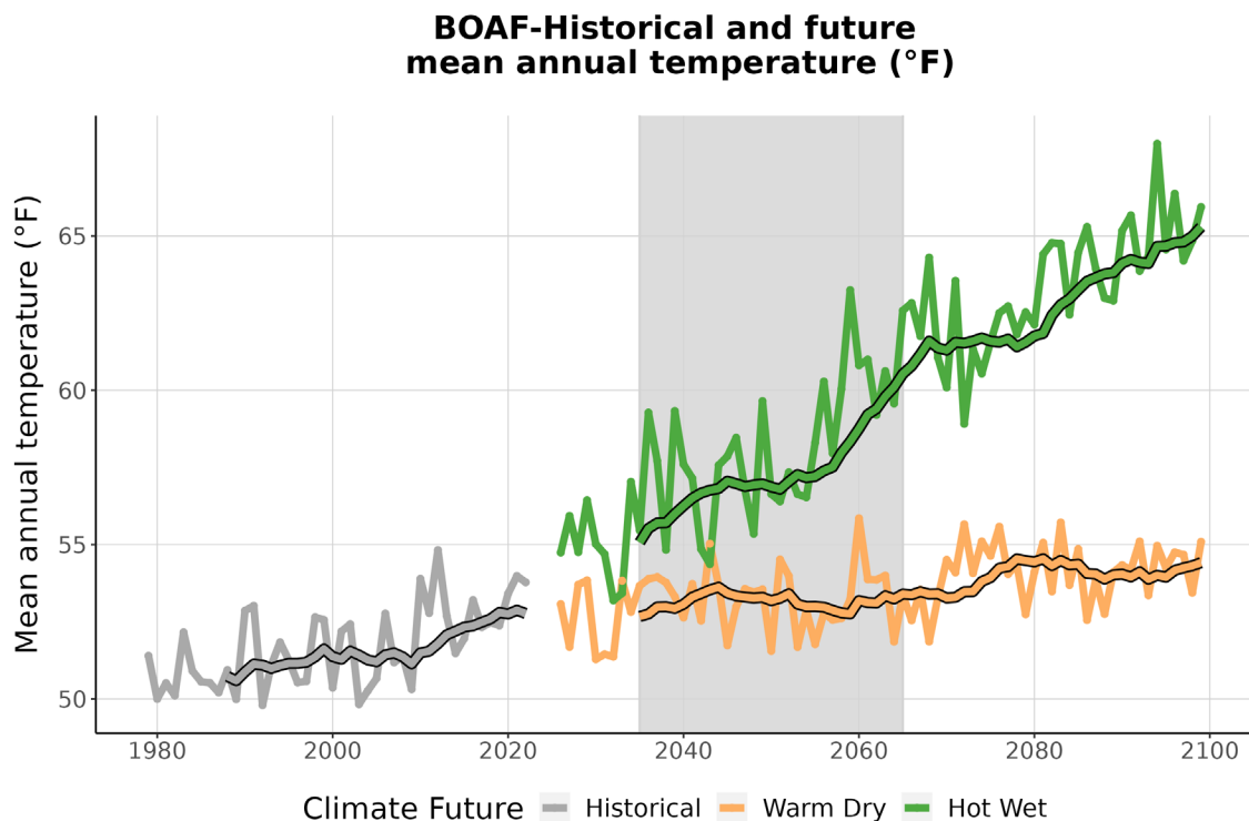
Figure 3. This graph compares observed average annual temperature at BOAF (°F) (1979-2022) with projected average annual temperature for the two climate futures over the period 2023-2099. The historically observed data
