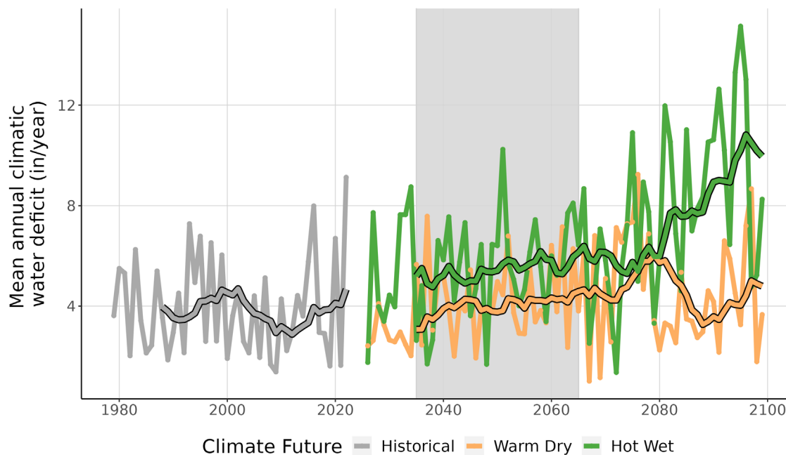
Figure 9. This line graph compares observed climatic water deficit at BOAF (inches/year) (1979-2022) with projected climatic water deficit for the two climate futures over the period 2023-2099. The historical observation data is shown in gray, the Warm Dry climate future in orange, and the Hot Wet climate future in green. The smooth line running through each projection is the 10-year running average for historical observations and future projections. Gray-shaded area represents the time period that was averaged (2035-2065) to summarize future projections for the year 2050.
