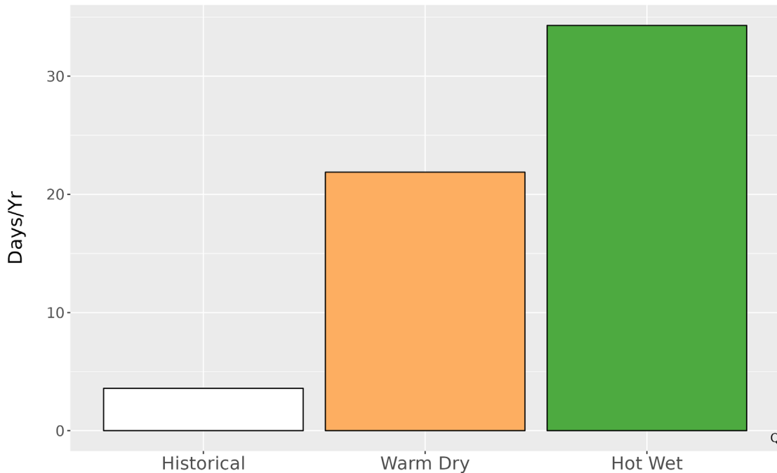
Figure 5. Metrics of extreme temperature at BLUE. The bar graph represents the average number of days annually with temperatures greater than the historical 99th percentile (89.3 °F) historically (1979-2012) and for the two climate futures (2050).
