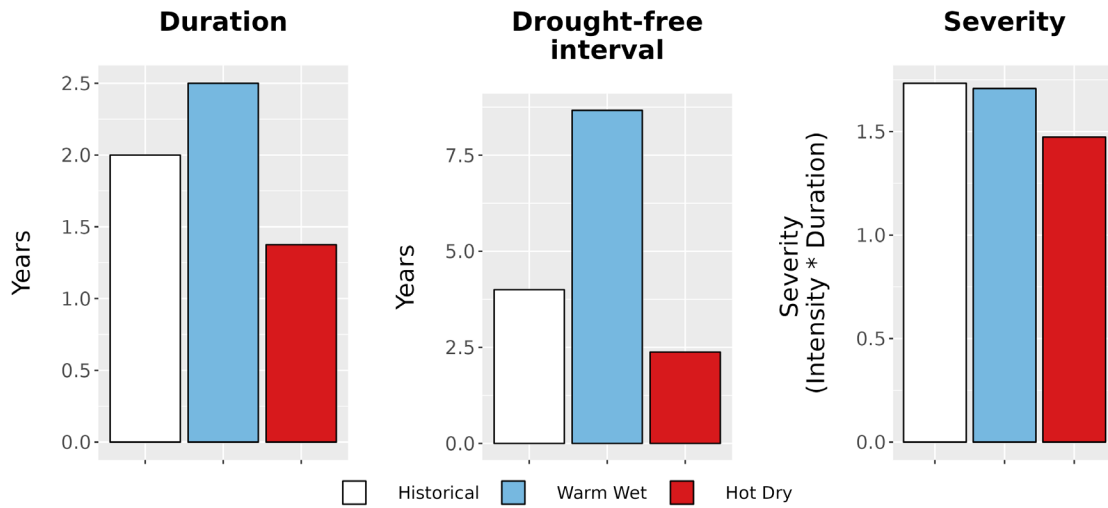
Figure 8. Drought metrics for BLRI. (Left) Average drought duration (years) historically (1979-2012) and under each climate future. (Middle) Average drought return interval (years), indicating the expected amount of time between periods of drought, historically and under each climate future. (Right) Average drought severity, a measure of drought intensity multiplied by duration, historically and under each climate future.
