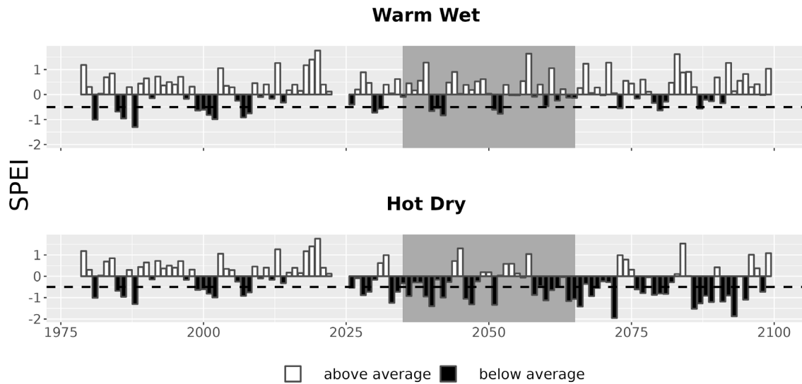
Figure 7. Drought metrics for BLRI. Drought index (SPEI; units = standard deviations from historical) timeseries for each climate future. Below-average SPEI (black bars) indicates dry conditions. The dotted line (SPEI = -0.5) indicates drought conditions.
