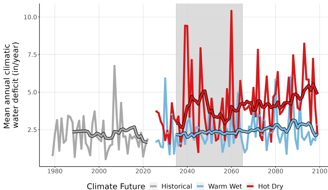
Figure 9. This line graph compares observed climatic water deficit at BLRI (inches/year) (1979-2022) with projected climatic water deficit for the two climate futures over the period 2023-2099. The historical observation data is shown in gray, the Warm Wet climate future in blue, and the Hot Dry climate future in red. The smooth line running through each projection is the 10-year running average for historical observations and future projections. Gray-shaded area represents the time period that was averaged (2035-2065) to summarize future projections for the year 2050.
