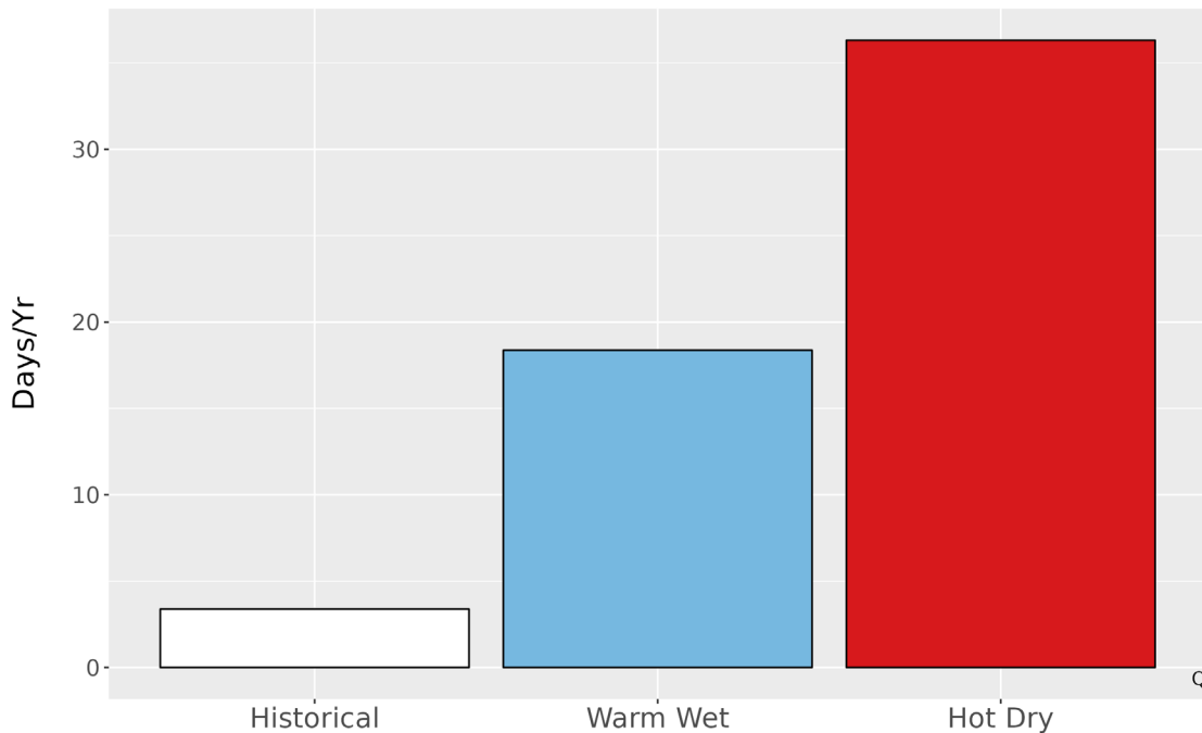
Figure 5. Metrics of extreme temperature at BLRI. The bar graph represents the average number of days annually with temperatures greater than the historical 99th percentile (85.9 °F) historically (1979-2012) and for the two climate futures (2050).
