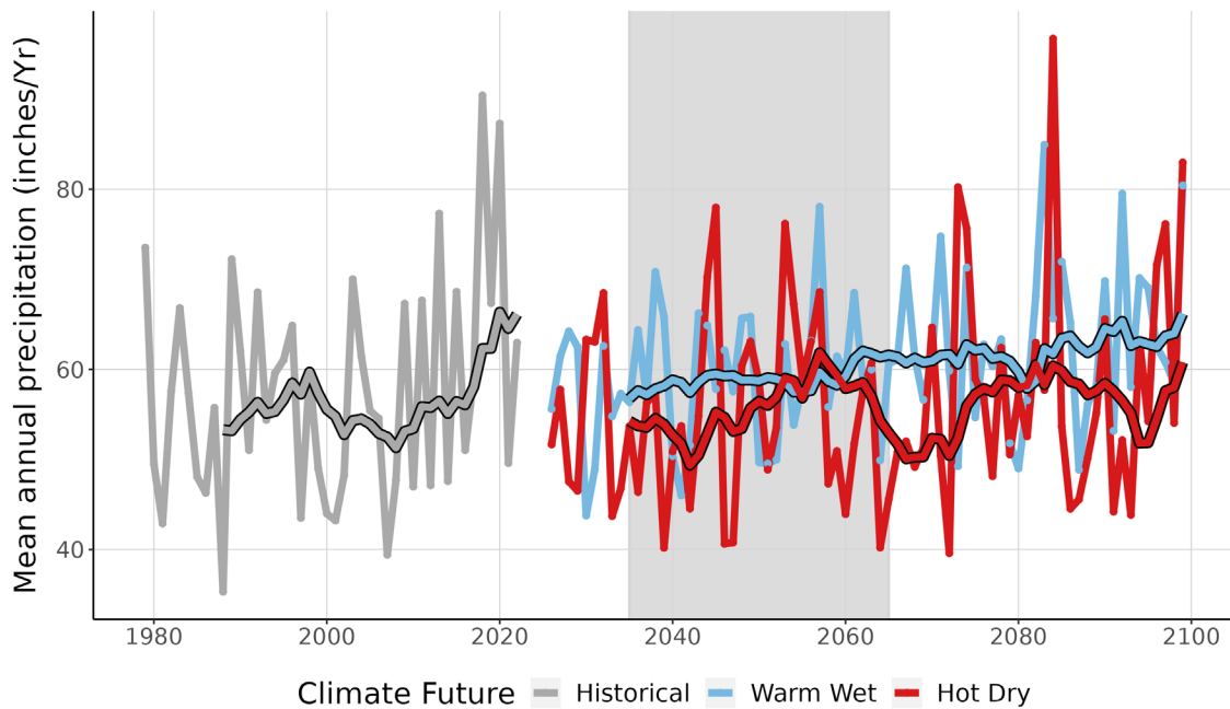
Figure 4. This graph compares observed average annual precipitation at BLRI (inches/year) (1979-2022) with projected average annual precipitation for the two climate futures over the period 2023-2099. The historically observed data is shown in gray, the Warm Wet climate future in blue, and the Hot Dry climate future in red. The smooth line running through each projection is the 10-year running average for historical observations and future projections. The gray-shaded area represents the time period that was averaged (2035-2065) to summarize future projections for the year 2050 (Appendix 1).
