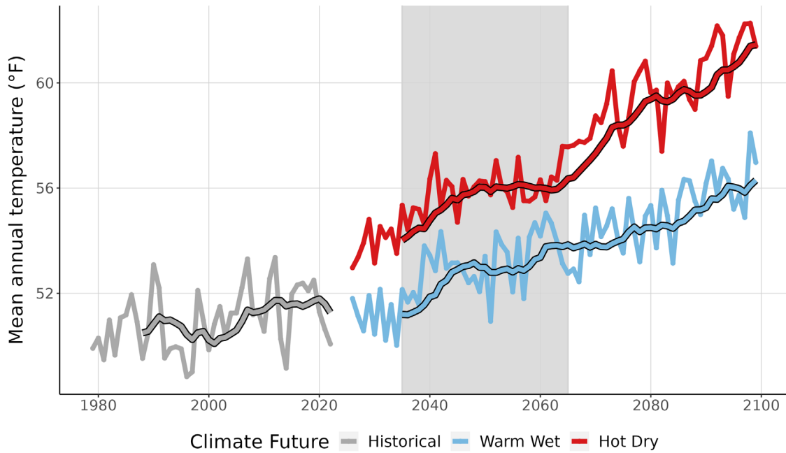
Figure 3. This graph compares observed average annual temperature at BLRI (°F) (1979-2022) with projected average annual temperature for the two climate futures over the period 2023-2099. The historically observed data is shown in gray, the Warm Wet climate future in blue, and the Hot Dry climate future in red. The smooth line running through each projection is the 10-year running average for historical observations and future projections. Gray-shaded area represents the time period that was averaged (2035-2065) to summarize future projections for the year 2050 (Appendix 1).
