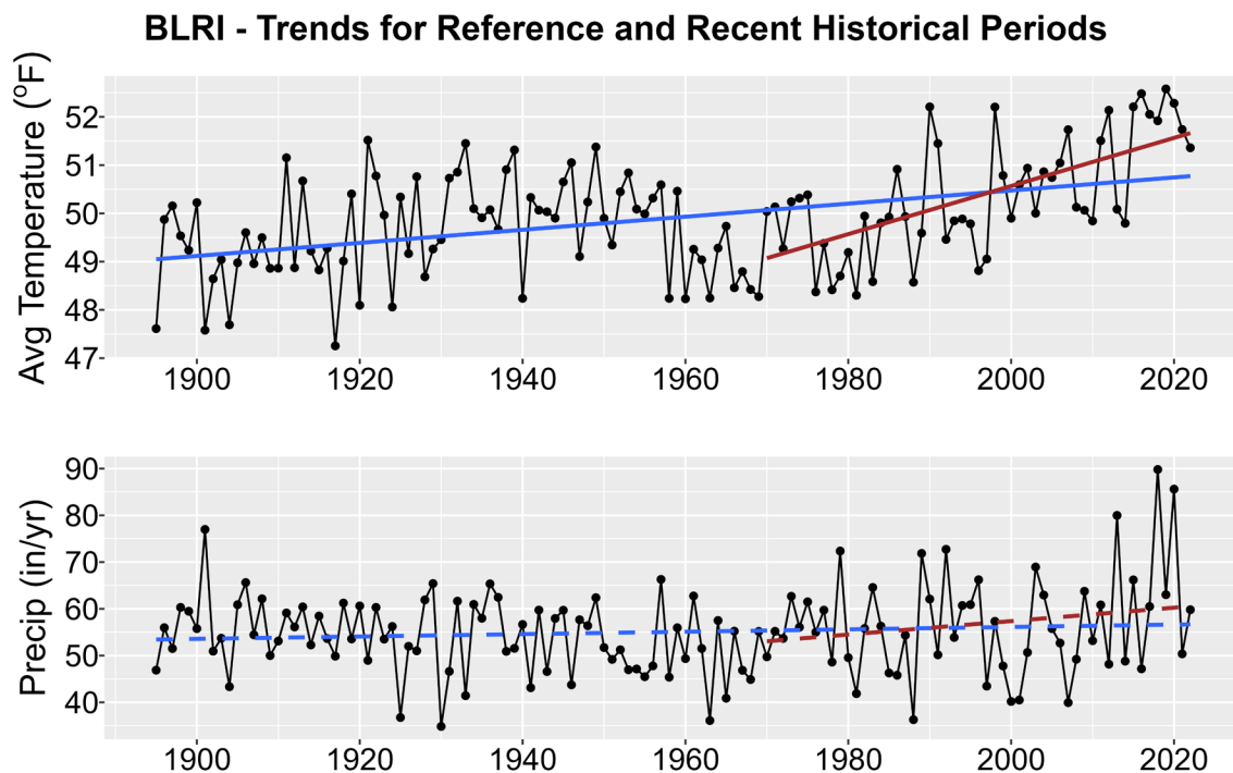
Figure 1. Historical trends in annual average temperature (upper plot) and annual total precipitation (lower plot) for BLRI from 1895-2022. Black points show yearly values while blue lines are linear regressions for the entire
