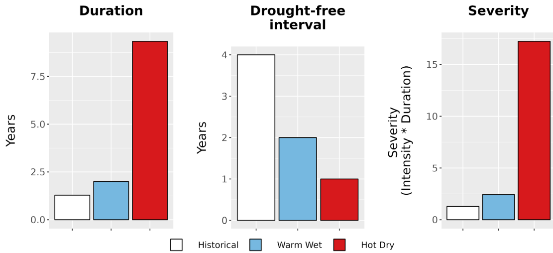
Figure 8. Drought metrics for BLCA. (Left) Average drought duration (years) historically (1979-2012) and under each climate future. (Middle) Average drought return interval (years), indicating the expected amount of time between periods of drought, historically and under each climate future. (Right) Average drought severity, a measure of drought intensity multiplied by duration, historically and under each climate future.
