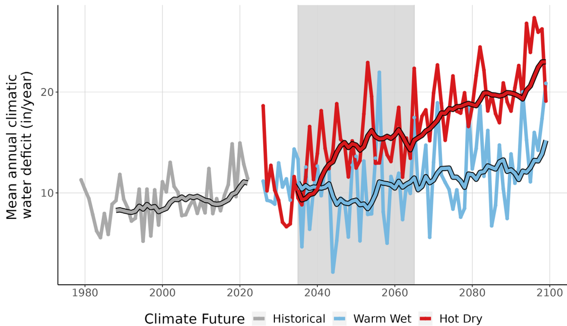
Figure 9. This line graph compares observed climatic water deficit at BLCA (inches/year) (1979-2022) with projected climatic water deficit for the two climate futures over the period 2023-2099. The historical observation data is shown in gray, the Warm Wet climate future in blue, and the Hot Dry climate future in red. The smooth line running through each projection is the 10-year running average for historical observations and future projections. Gray-shaded area represents the time period that was averaged (2035-2065) to summarize future projections for the year 2050.
