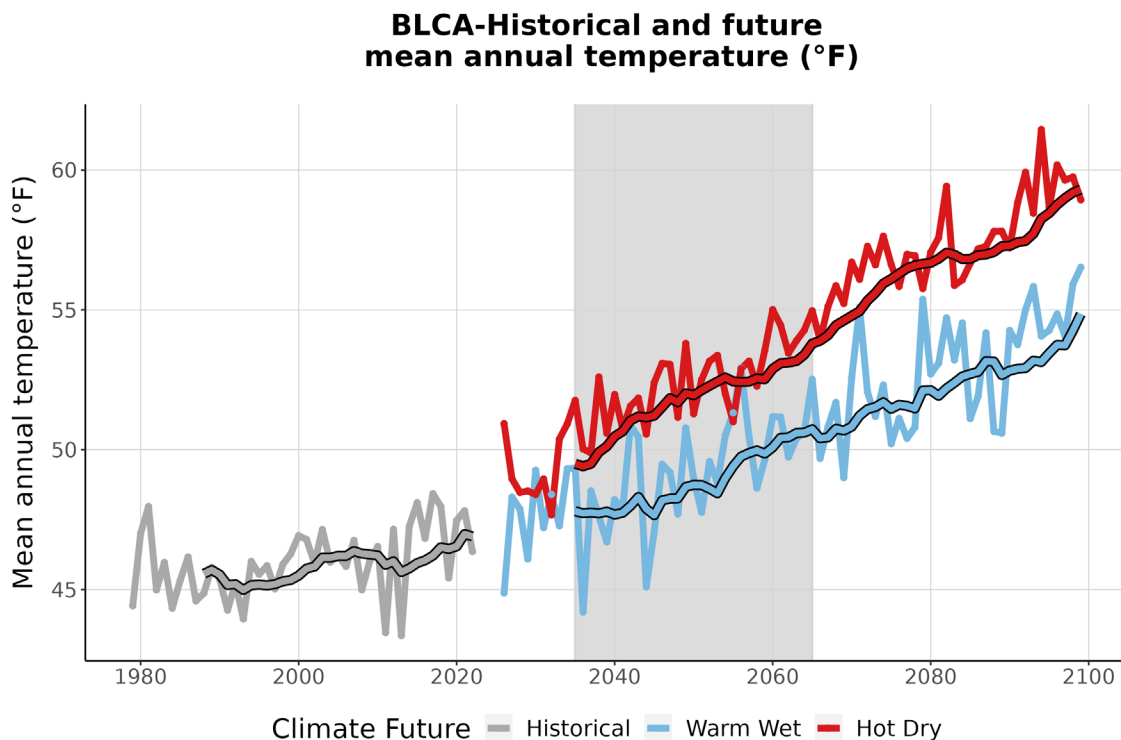
Figure 3. This graph compares observed average annual temperature at BLCA (°F) (1979-2022) with projected average annual temperature for the two climate futures over the period 2023-2099. The historically observed data
