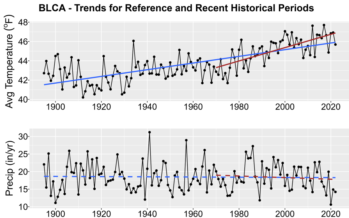
Figure 1. Historical trends in annual average temperature (upper plot) and annual total precipitation (lower plot) for BLCA from 1895-2022. Black points show yearly values while blue lines are linear regressions for the entire period record and red lines for 1970-2022 trends. Solid lines are significant trends (i.e., p < 0.05 ); dashed lines are not statistically significant.
