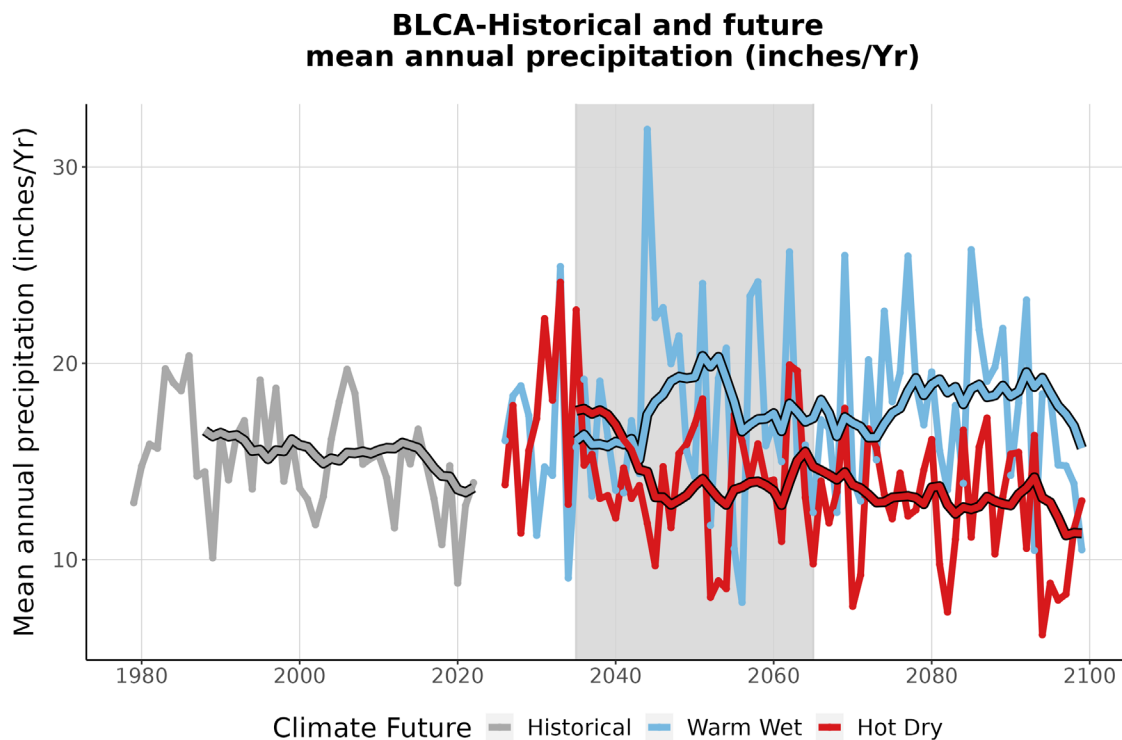
Figure 4. This graph compares observed average annual precipitation at BLCA (inches/year) (1979-2022) with projected average annual precipitation for the two climate futures over the period 2023-2099. The historically observed data is shown in gray, the Warm Wet climate future in blue, and the Hot Dry climate future in red. The smooth line running through each projection is the 10-year running average for historical observations and future projections. The gray-shaded area represents the time period that was averaged (2035-2065) to summarize future projections for the year 2050 (Appendix 1).
