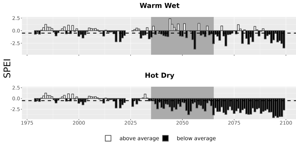
Figure 7. Drought metrics for BLCA. Drought index (SPEI; units = standard deviations from historical) timeseries for each climate future. Below-average SPEI (black bars) indicates dry conditions. The dotted line (SPEI = -0.5) indicates drought conditions.
