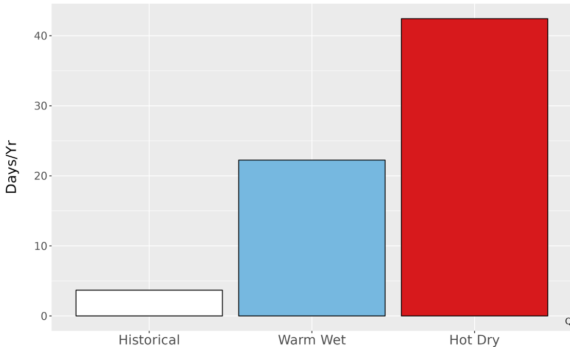
Figure 5. Metrics of extreme temperature at BLCA. The bar graph represents the average number of days annually with temperatures greater than the historical 99th percentile (89.5 °F) historically (1979-2012) and for the two climate futures (2050).
