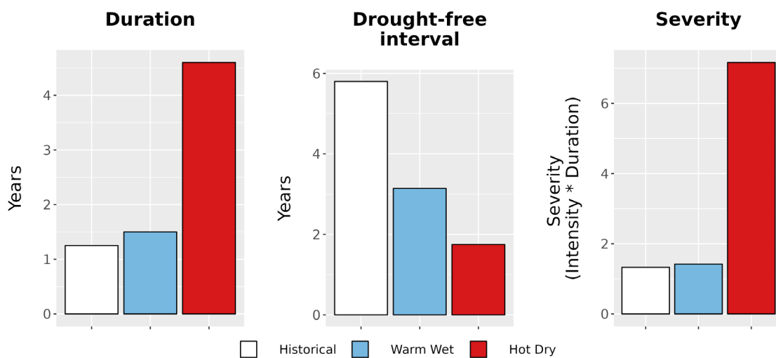
Figure 8. Drought metrics for BITH. (Left) Average drought duration (years) historically (1979-2012) and under each climate future. (Middle) Average drought return interval (years), indicating the expected amount of time between periods of drought, historically and under each climate future. (Right) Average drought severity, a measure of drought intensity multiplied by duration, historically and under each climate future.
