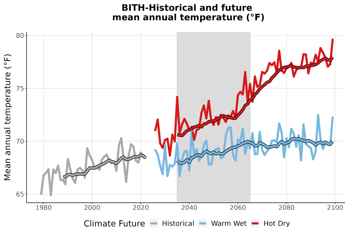
Figure 3. This graph compares observed average annual temperature at BITH (°F) (1979-2022) with projected average annual temperature for the two climate futures over the period 2023-2099. The historically observed data
