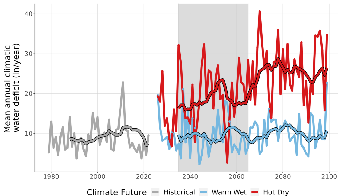
Figure 9. This line graph compares observed climatic water deficit at BITH (inches/year) (1979-2022) with projected climatic water deficit for the two climate futures over the period 2023-2099. The historical observation data is shown in gray, the Warm Wet climate future in blue, and the Hot Dry climate future in red. The smooth line running through each projection is the 10-year running average for historical observations and future projections. Gray-shaded area represents the time period that was averaged (2035-2065) to summarize future projections for the year 2050.
