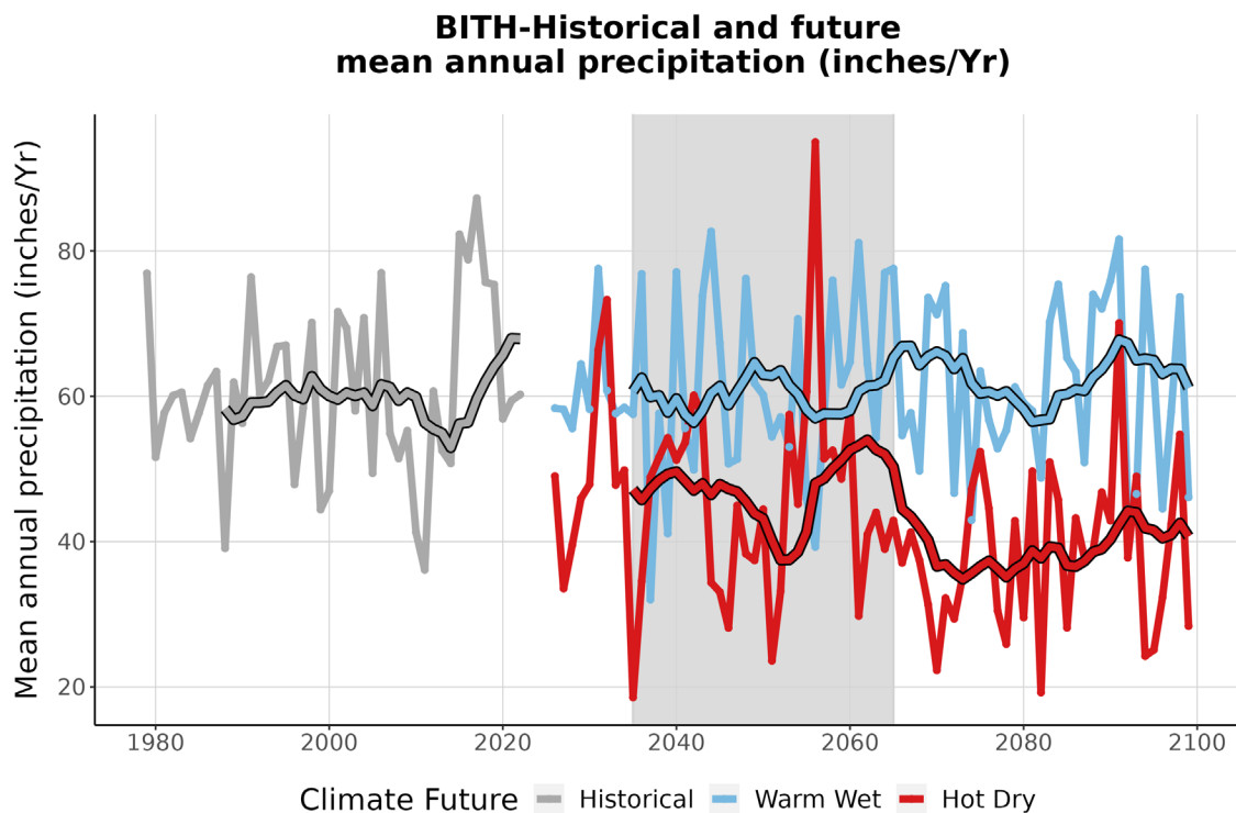
Figure 4. This graph compares observed average annual precipitation at BITH (inches/year) (1979-2022) with projected average annual precipitation for the two climate futures over the period 2023-2099. The historically observed data is shown in gray, the Warm Wet climate future in blue, and the Hot Dry climate future in red. The smooth line running through each projection is the 10-year running average for historical observations and future projections. The gray-shaded area represents the time period that was averaged (2035-2065) to summarize future projections for the year 2050 (Appendix 1).
