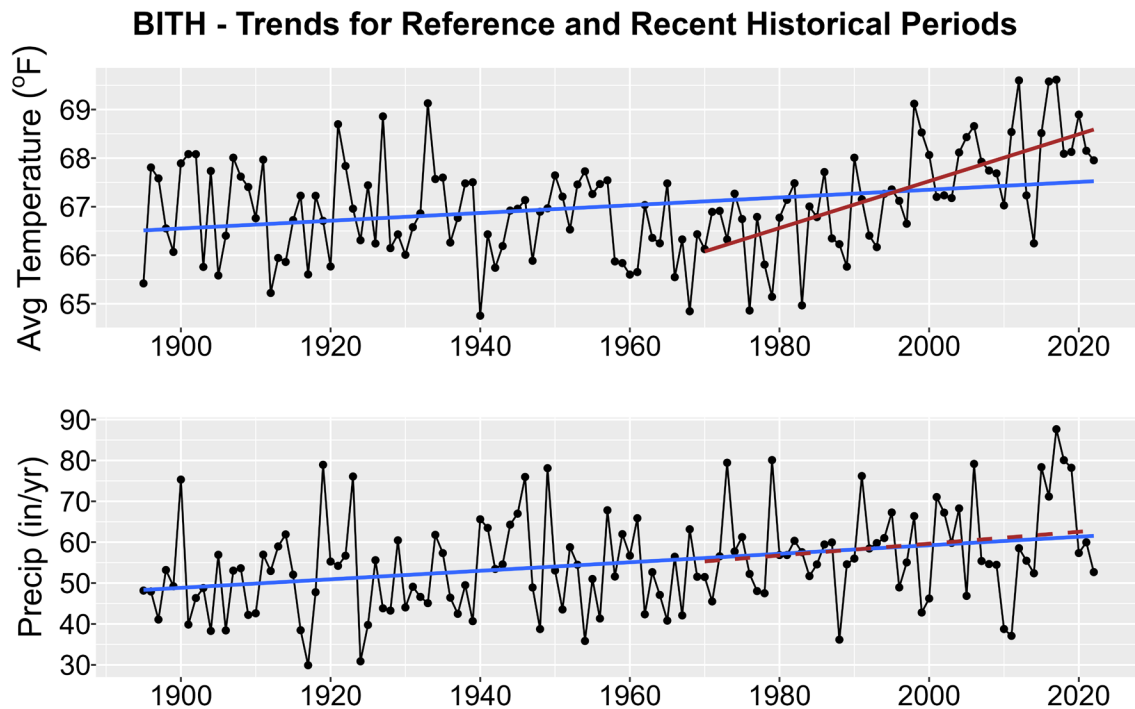
Figure 1. Historical trends in annual average temperature (upper plot) and annual total precipitation (lower plot) for BITH from 1895-2022. Black points show yearly values while blue lines are linear regressions for the entire period record and red lines for 1970-2022 trends. Solid lines are significant trends (i.e., p < 0.05 ); dashed lines are not statistically significant.
