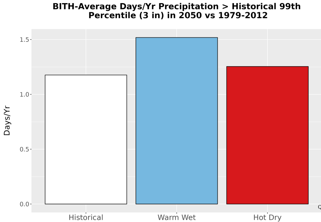
Figure 6. Average number of days annually with precipitation exceeding the 99th percentile (3 in.) of precipitation from the historical period 1979-2012 and for each climate future.
