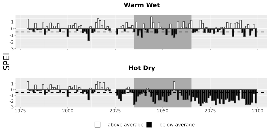
Figure 7. Drought metrics for BITH. Drought index (SPEI; units = standard deviations from historical) timeseries for each climate future. Below-average SPEI (black bars) indicates dry conditions. The dotted line (SPEI = -0.5) indicates drought conditions.
