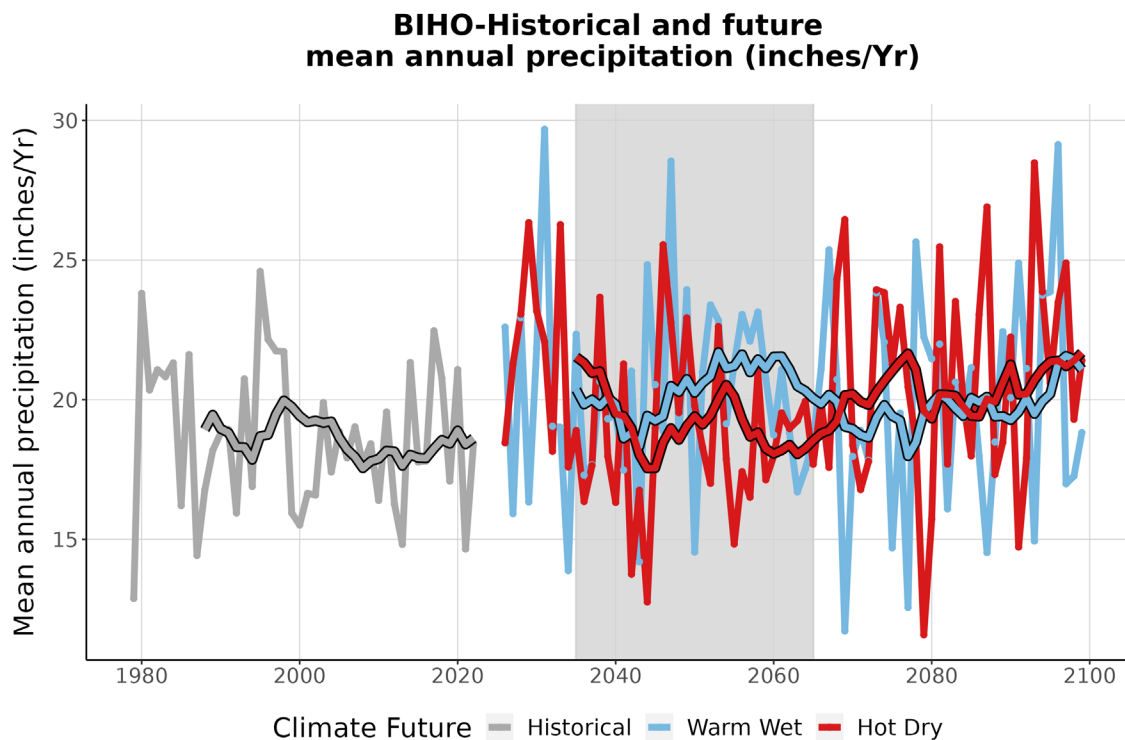
Figure 4. This graph compares observed average annual precipitation at BIHO (inches/year) (1979-2022) with projected average annual precipitation for the two climate futures over the period 2023-2099. The historically observed data is shown in gray, the Warm Wet climate future in blue, and the Hot Dry climate future in red. The smooth line running through each projection is the 10-year running average for historical observations and future projections. The gray-shaded area represents the time period that was averaged (2035-2065) to summarize future projections for the year 2050 (Appendix 1).
