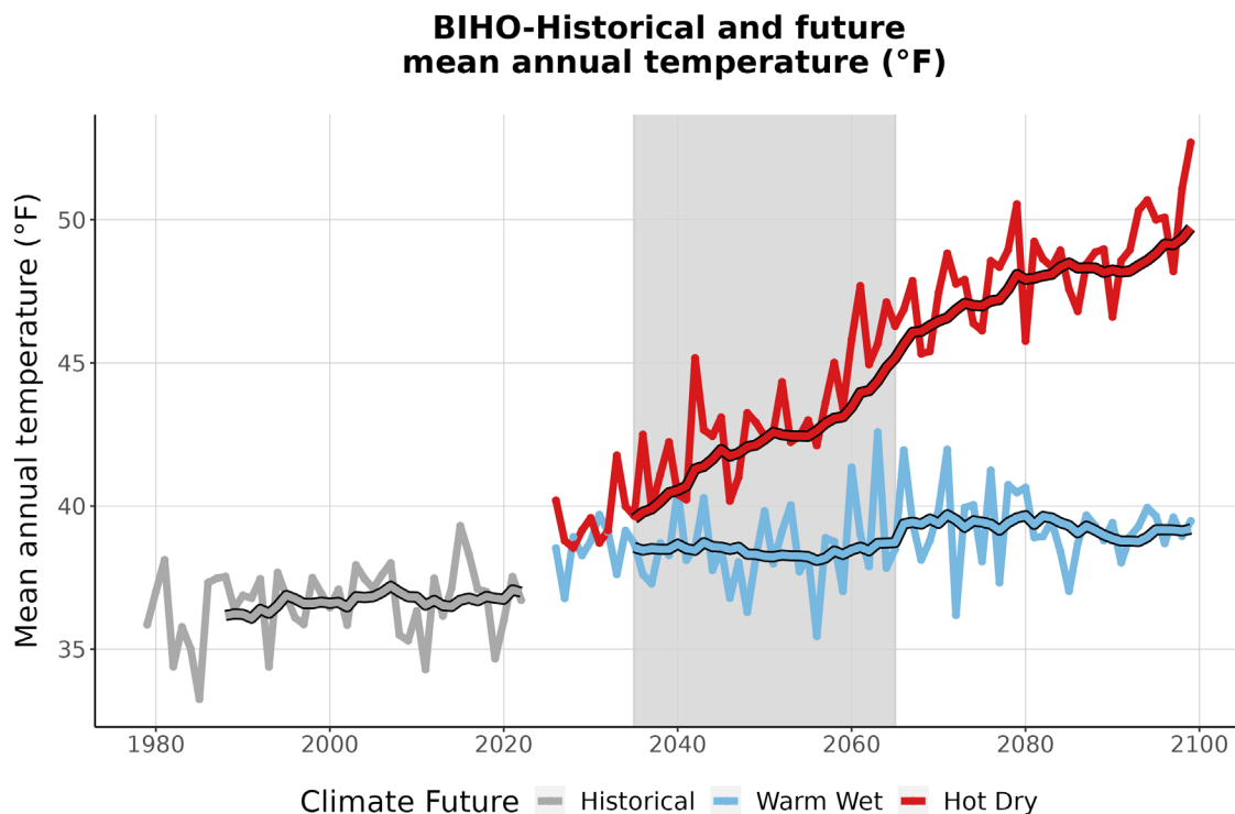
Figure 3. This graph compares observed average annual temperature at BIHO (°F) (1979-2022) with projected average annual temperature for the two climate futures over the period 2023-2099. The historically observed data
