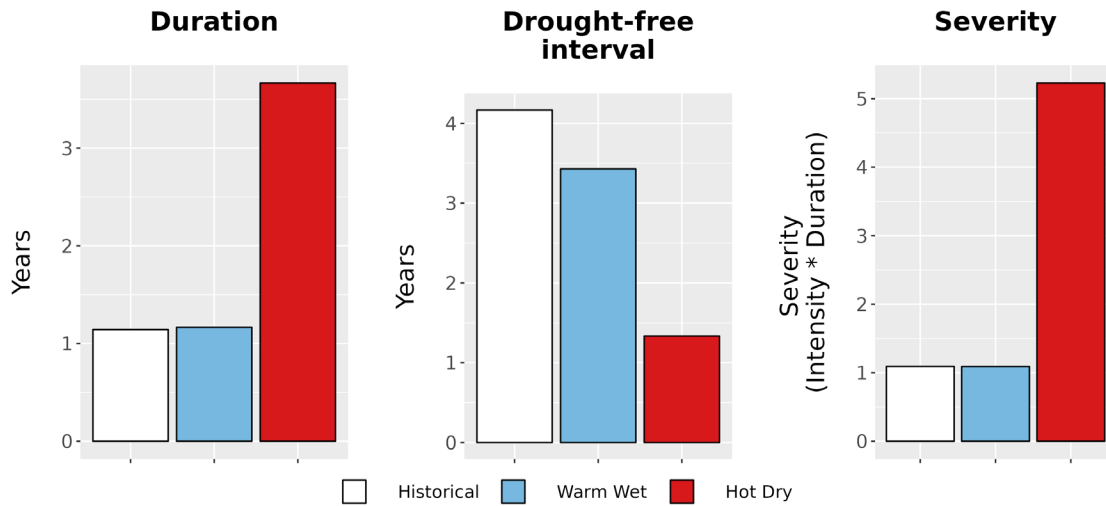
Figure 8. Drought metrics for BIHO. (Left) Average drought duration (years) historically (1979-2012) and under each climate future. (Middle) Average drought return interval (years), indicating the expected amount of time between periods of drought, historically and under each climate future. (Right) Average drought severity, a measure of drought intensity multiplied by duration, historically and under each climate future.
