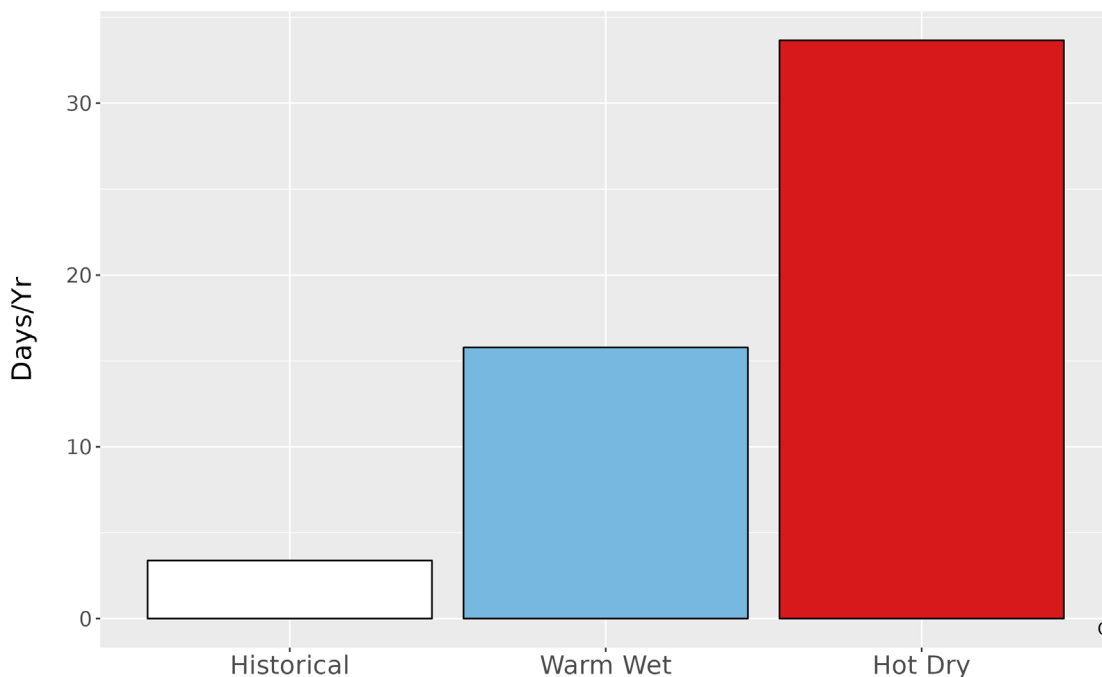
Figure 5. Metrics of extreme temperature at BIHO. The bar graph represents the average number of days annually with temperatures greater than the historical 99th percentile (86.1 °F) historically (1979-2012) and for the two climate futures (2050).
