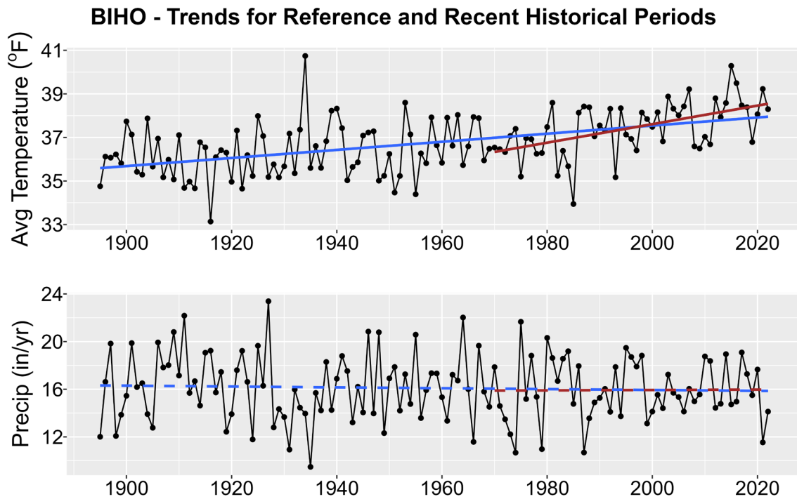
Figure 1. Historical trends in annual average temperature (upper plot) and annual total precipitation (lower plot) for BIHO from 1895-2022. Black points show yearly values while blue lines are linear regressions for the entire period record and red lines for 1970-2022 trends. Solid lines are significant trends (i.e., p < 0.05 ); dashed lines are not statistically significant.
