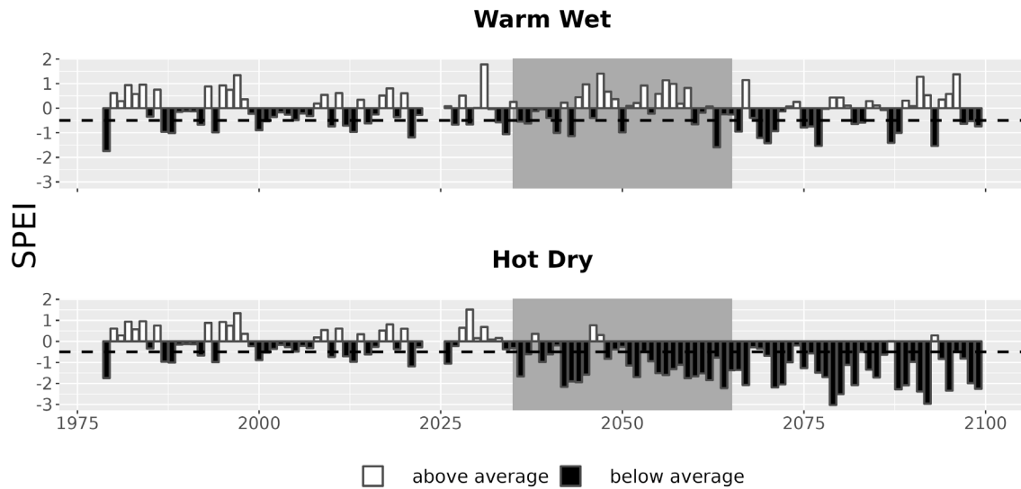
Figure 7. Drought metrics for BIHO. Drought index (SPEI; units = standard deviations from historical) timeseries for each climate future. Below-average SPEI (black bars) indicates dry conditions. The dotted line (SPEI = -0.5) indicates drought conditions.
