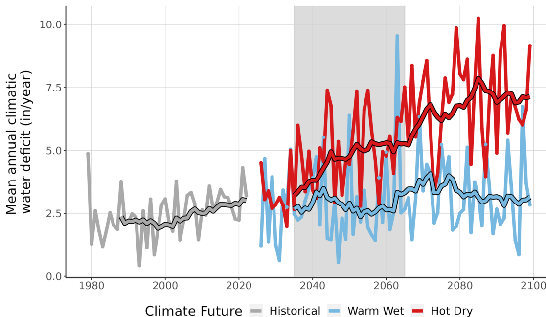
Figure 9. This line graph compares observed climatic water deficit at BIHO (inches/year) (1979-2022) with projected climatic water deficit for the two climate futures over the period 2023-2099. The historical observation data is shown in gray, the Warm Wet climate future in blue, and the Hot Dry climate future in red. The smooth line running through each projection is the 10-year running average for historical observations and future projections. Gray-shaded area represents the time period that was averaged (2035-2065) to summarize future projections for the year 2050.
