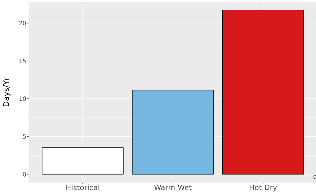
Figure 5. Metrics of extreme temperature at BICA. The bar graph represents the average number of days annually with temperatures greater than the historical 99th percentile (97.8 °F) historically (1979-2012) and for the two climate futures (2050).
