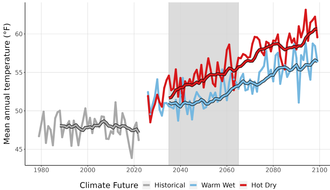
Figure 3. This graph compares observed average annual temperature at BICA (°F) (1979-2022) with projected average annual temperature for the two climate futures over the period 2023-2099. The historically observed data is shown in gray, the Warm Wet climate future in blue, and the Hot Dry climate future in red. The smooth line running through each projection is the 10-year running average for historical observations and future projections. Gray-shaded area represents the time period that was averaged (2035-2065) to summarize future projections for the year 2050 (Appendix 1).
