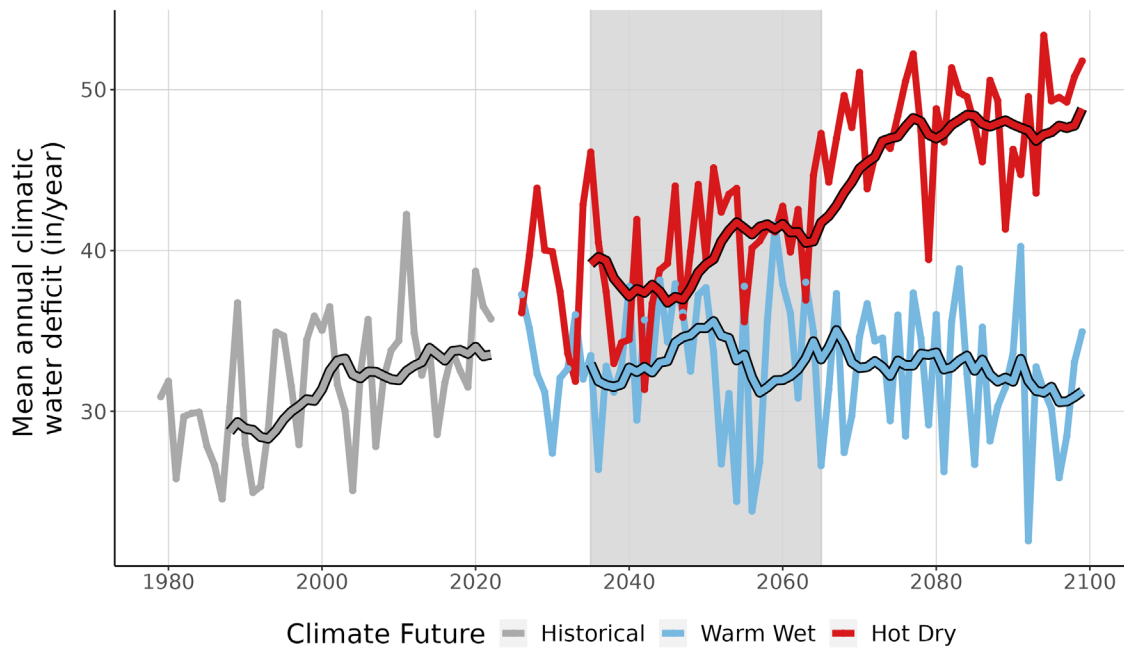
Figure 9. This line graph compares observed climatic water deficit at BIBE (inches/year) (1979-2022) with projected climatic water deficit for the two climate futures over the period 2023-2099. The historical observation data is shown in gray, the Warm Wet climate future in blue, and the Hot Dry climate future in red. The smooth line running through each projection is the 10-year running average for historical observations and future projections. Gray-shaded area represents the time period that was averaged (2035-2065) to summarize future projections for the year 2050.
