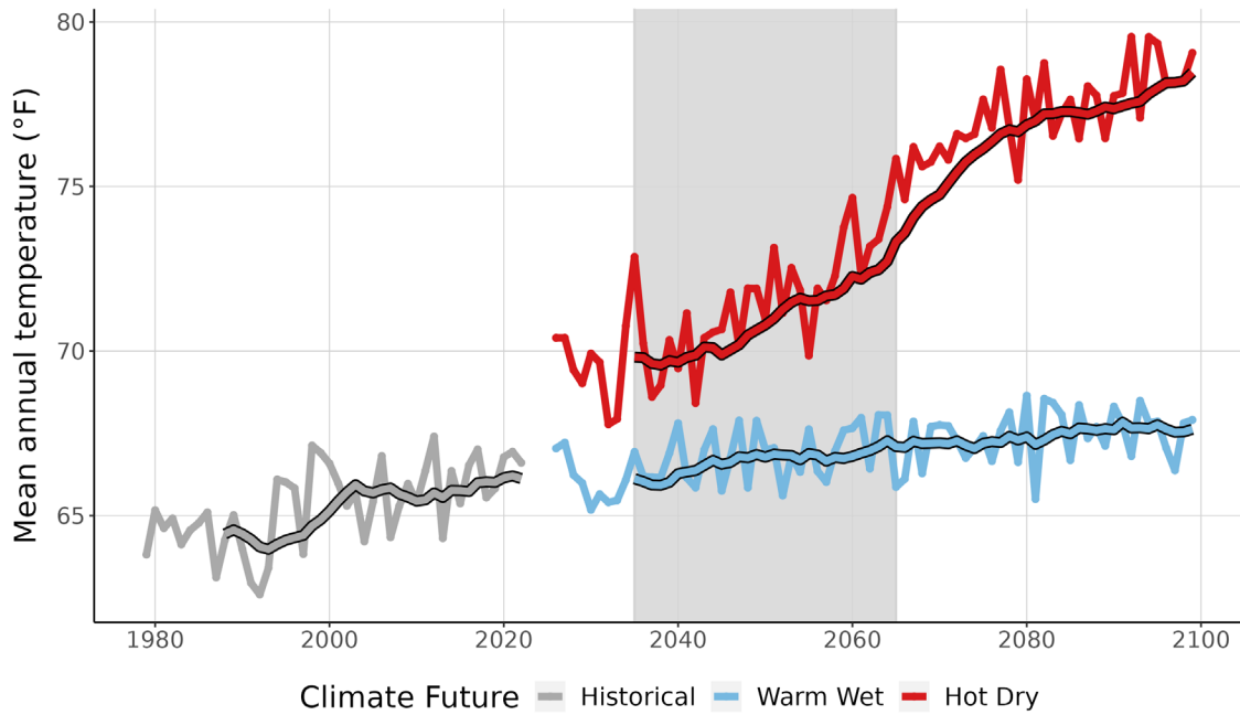
Figure 3. This graph compares observed average annual temperature at BIBE (°F) (1979-2022) with projected average annual temperature for the two climate futures over the period 2023-2099. The historically observed data is shown in gray, the Warm Wet climate future in blue, and the Hot Dry climate future in red. The smooth line running through each projection is the 10-year running average for historical observations and future projections. Gray-shaded area represents the time period that was averaged (2035-2065) to summarize future projections for the year 2050 (Appendix 1).
