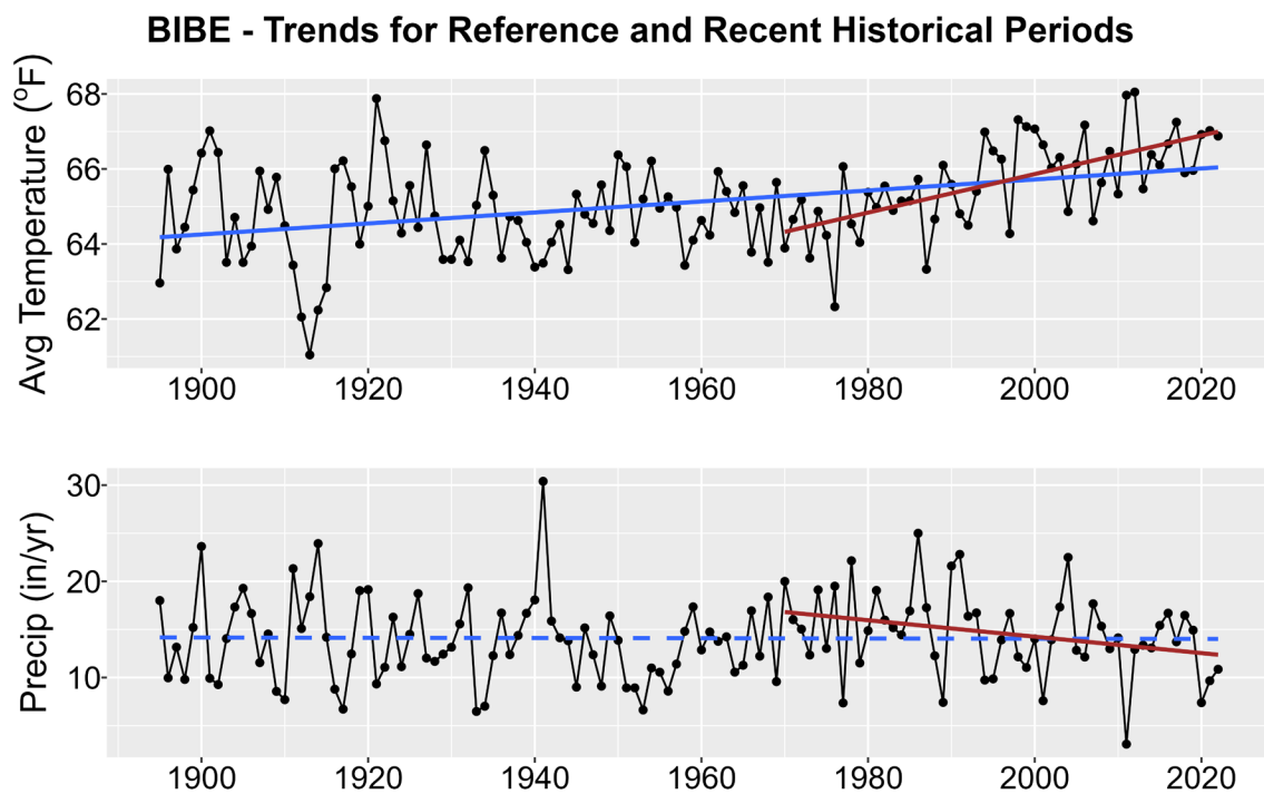
Figure 1. Historical trends in annual average temperature (upper plot) and annual total precipitation (lower plot) for BIBE from 1895-2022. Black points show yearly values while blue lines are linear regressions for the entire period record and red lines for 1970-2022 trends. Solid lines are significant trends (i.e., p < 0.05 ); dashed lines are not statistically significant.
