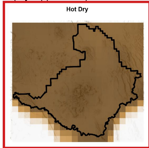
Figure A3. (Top) Map showing average annual climatic water deficit for the historical period (inches/year) and (bottom) change in average annual climatic water deficit for the two climate futures. Legends are located below each set of maps as a continuous color gradient. Gridded data is extracted from Hegewisch, K.C. and J.T. Abatzoglou, 'Climate Mapper' web tool. Climate Toolbox ( https://climatetoolbox.org/ ) accessed on 6/3/2024.
