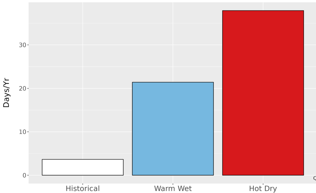
Figure 5. Metrics of extreme temperature at BIBE. The bar graph represents the average number of days annually with temperatures greater than the historical 99th percentile (98.5 °F) historically (1979-2012) and for the two climate futures (2050).
