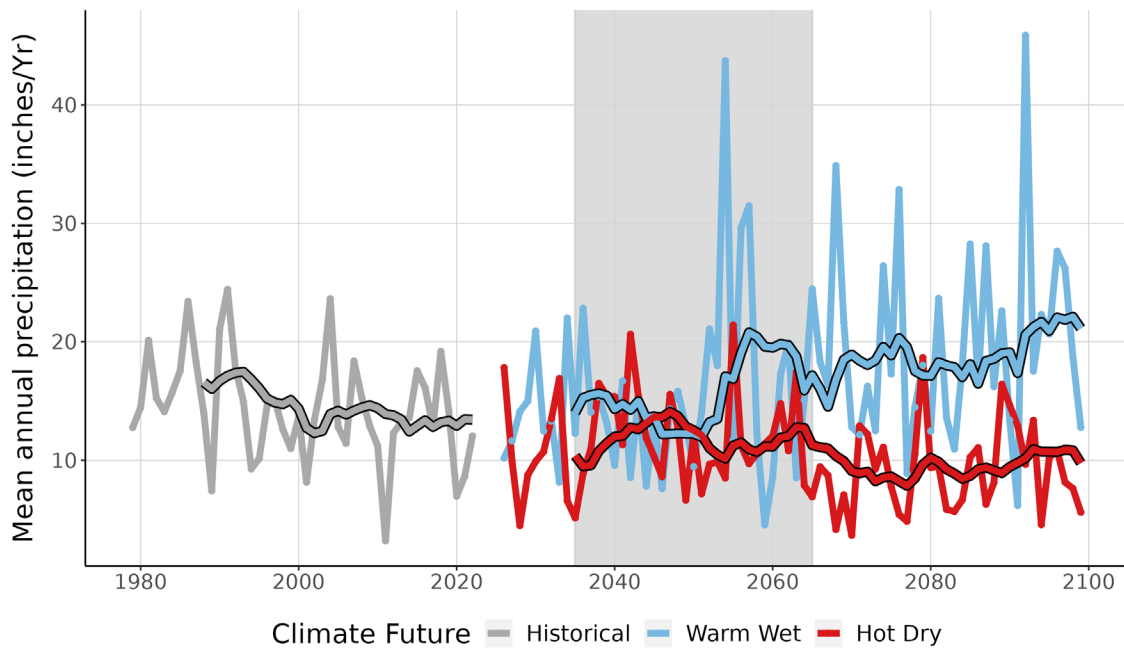
Figure 4. This graph compares observed average annual precipitation at BIBE (inches/year) (1979-2022) with projected average annual precipitation for the two climate futures over the period 2023-2099. The historically observed data is shown in gray, the Warm Wet climate future in blue, and the Hot Dry climate future in red. The smooth line running through each projection is the 10-year running average for historical observations and future projections. The gray-shaded area represents the time period that was averaged (2035-2065) to summarize future projections for the year 2050 (Appendix 1).
