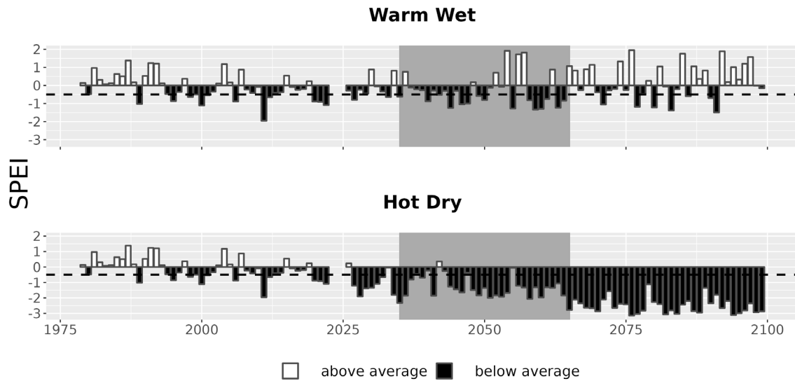
Figure 7. Drought metrics for BIBE. Drought index (SPEI; units = standard deviations from historical) timeseries for each climate future. Below-average SPEI (black bars) indicates dry conditions. The dotted line (SPEI = -0.5) indicates drought conditions.
