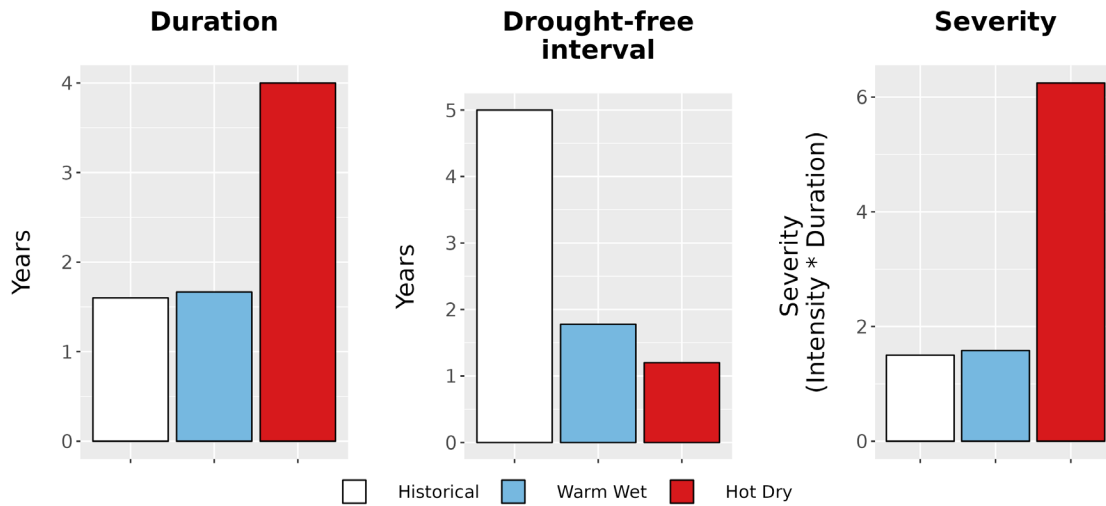
Figure 8. Drought metrics for BIBE. (Left) Average drought duration (years) historically (1979-2012) and under each climate future. (Middle) Average drought return interval (years), indicating the expected amount of time between periods of drought, historically and under each climate future. (Right) Average drought severity, a measure of drought intensity multiplied by duration, historically and under each climate future.
