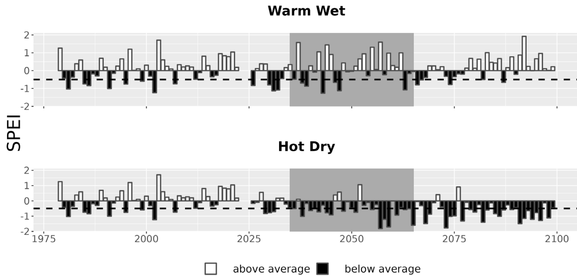
Figure 7. Drought metrics for BEPA. Drought index (SPEI; units = standard deviations from historical) timeseries for each climate future. Below-average SPEI (black bars) indicates dry conditions. The dotted line (SPEI = -0.5) indicates drought conditions.
