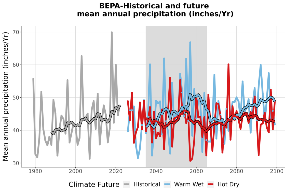
Figure 4. This graph compares observed average annual precipitation at BEPA (inches/year) (1979-2022) with projected average annual precipitation for the two climate futures over the period 2023-2099. The historically observed data is shown in gray, the Warm Wet climate future in blue, and the Hot Dry climate future in red. The smooth line running through each projection is the 10-year running average for historical observations and future projections. The gray-shaded area represents the time period that was averaged (2035-2065) to summarize future projections for the year 2050 (Appendix 1).
