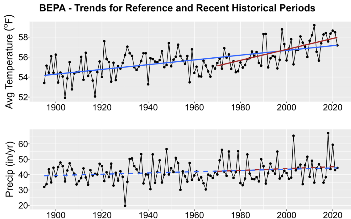
Figure 1. Historical trends in annual average temperature (upper plot) and annual total precipitation (lower plot) for BEPA from 1895-2022. Black points show yearly values while blue lines are linear regressions for the entire period record and red lines for 1970-2022 trends. Solid lines are significant trends (i.e., p < 0.05 ); dashed lines are not statistically significant.
