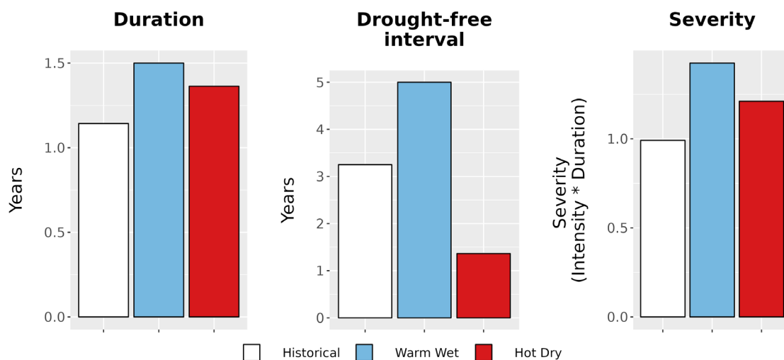
Figure 8. Drought metrics for BEPA. (Left) Average drought duration (years) historically (1979-2012) and under each climate future. (Middle) Average drought return interval (years), indicating the expected amount of time between periods of drought, historically and under each climate future. (Right) Average drought severity, a measure of drought intensity multiplied by duration, historically and under each climate future.
