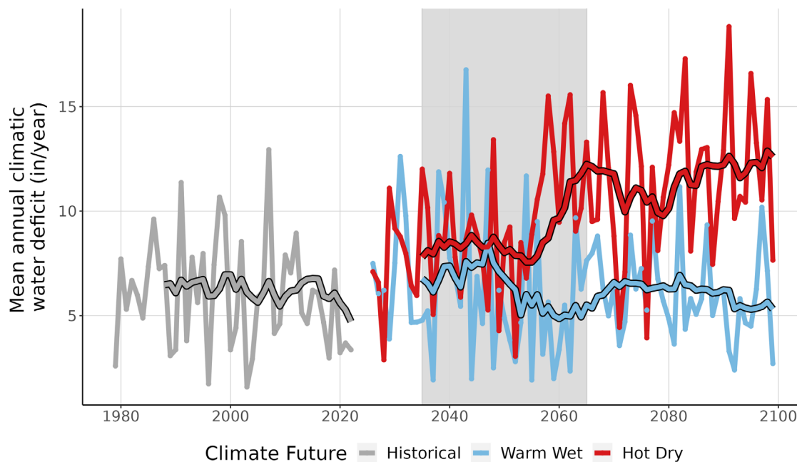
Figure 9. This line graph compares observed climatic water deficit at BEPA (inches/year) (1979-2022) with projected climatic water deficit for the two climate futures over the period 2023-2099. The historical observation data is shown in gray, the Warm Wet climate future in blue, and the Hot Dry climate future in red. The smooth line running through each projection is the 10-year running average for historical observations and future projections. Gray-shaded area represents the time period that was averaged (2035-2065) to summarize future projections for the year 2050.
