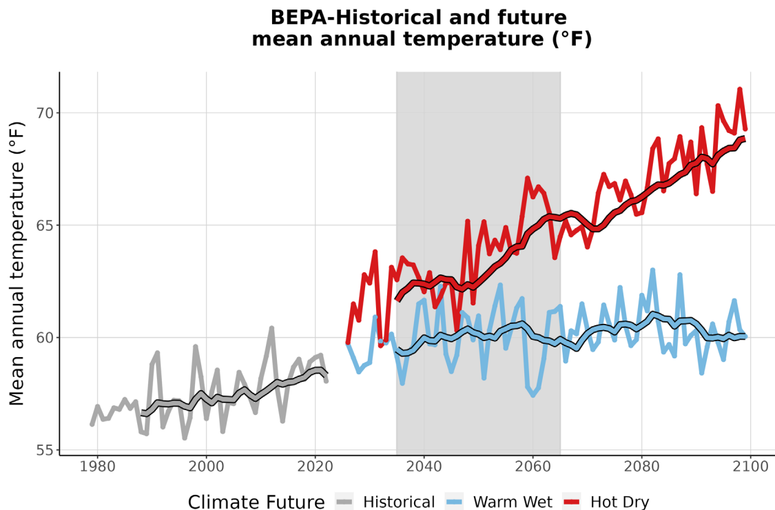
Figure 3. This graph compares observed average annual temperature at BEPA (°F) (1979-2022) with projected average annual temperature for the two climate futures over the period 2023-2099. The historically observed data
