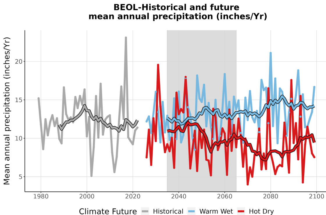
Figure 4. This graph compares observed average annual precipitation at BEOL (inches/year) (1979-2022) with projected average annual precipitation for the two climate futures over the period 2023-2099. The historically observed data is shown in gray, the Warm Wet climate future in blue, and the Hot Dry climate future in red. The smooth line running through each projection is the 10-year running average for historical observations and future projections. The gray-shaded area represents the time period that was averaged (2035-2065) to summarize future projections for the year 2050 (Appendix 1).
