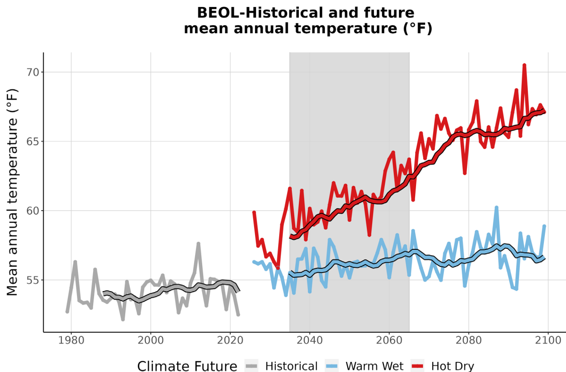
Figure 3. This graph compares observed average annual temperature at BEOL (°F) (1979-2022) with projected average annual temperature for the two climate futures over the period 2023-2099. The historically observed data
