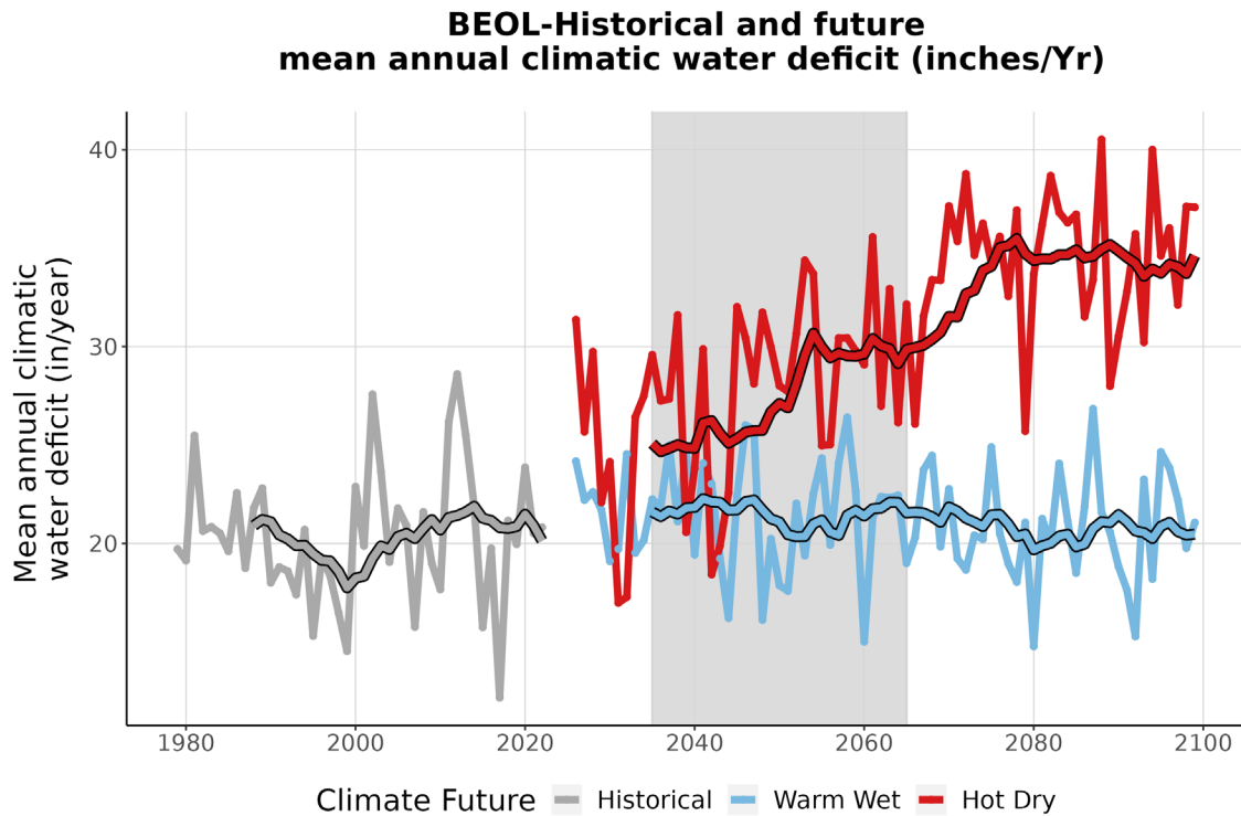
Figure 9. This line graph compares observed climatic water deficit at BEOL (inches/year) (1979-2022) with projected climatic water deficit for the two climate futures over the period 2023-2099. The historical observation data is shown in gray, the Warm Wet climate future in blue, and the Hot Dry climate future in red. The smooth line running through each projection is the 10-year running average for historical observations and future projections. Gray-shaded area represents the time period that was averaged (2035-2065) to summarize future projections for the year 2050.
