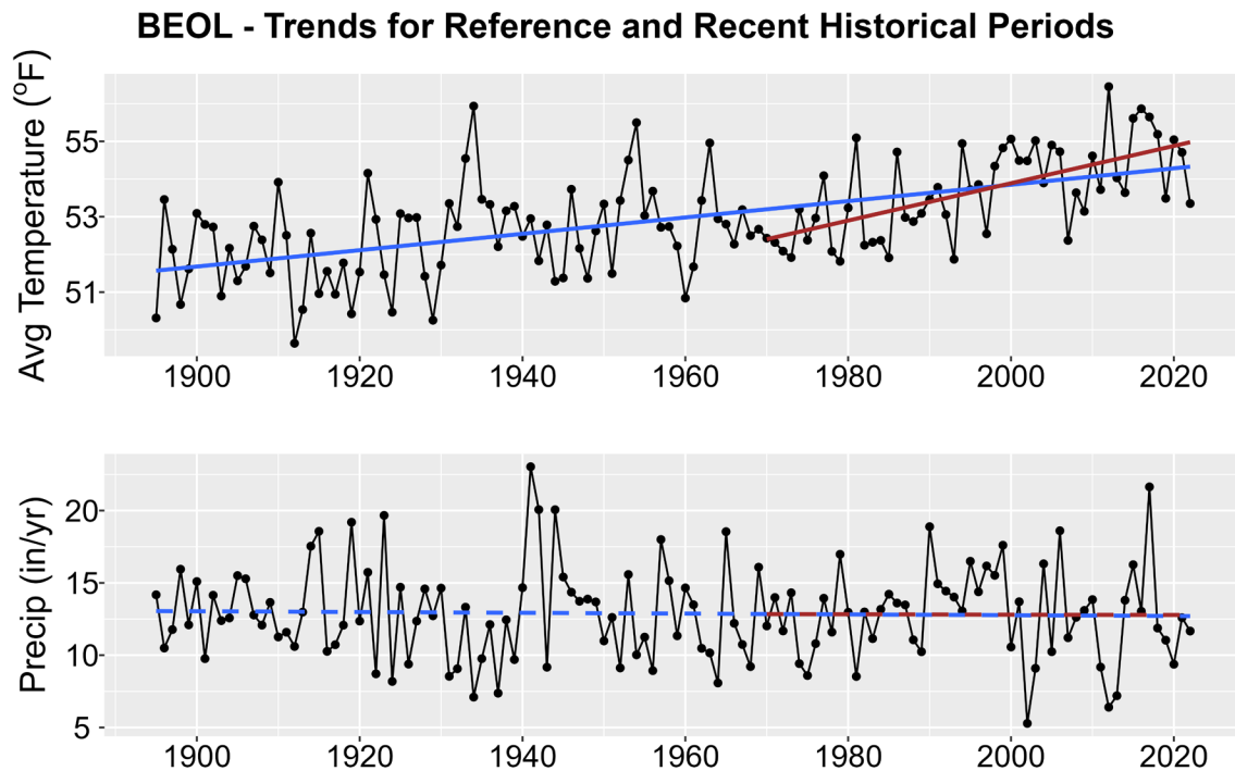
Figure 1. Historical trends in annual average temperature (upper plot) and annual total precipitation (lower plot) for BEOL from 1895-2022. Black points show yearly values while blue lines are linear regressions for the entire period record and red lines for 1970-2022 trends. Solid lines are significant trends (i.e., p < 0.05 ); dashed lines are not statistically significant.
