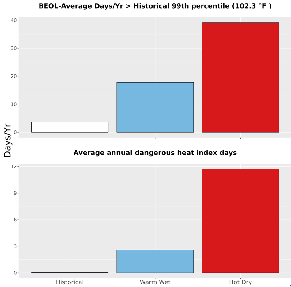
Figure 5. The upper bar graph represents the average number of days annually with temperatures greater than the historical 99th percentile (102.3 °F) historically (1979-2012) and for the two climate futures (2050). The bottom bar graph represents the average annual number of dangerous heat index days historically and for the two climate futures. Dangerous heat index days are days that exceed 105 °F.
