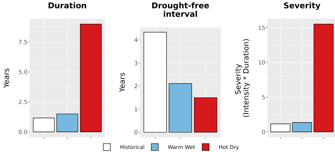
Figure 8. Drought metrics for BEOL. (Left) Average drought duration (years) historically (1979-2012) and under each climate future. (Middle) Average drought return interval (years), indicating the expected amount of time between periods of drought, historically and under each climate future. (Right) Average drought severity, a measure of drought intensity multiplied by duration, historically and under each climate future.
