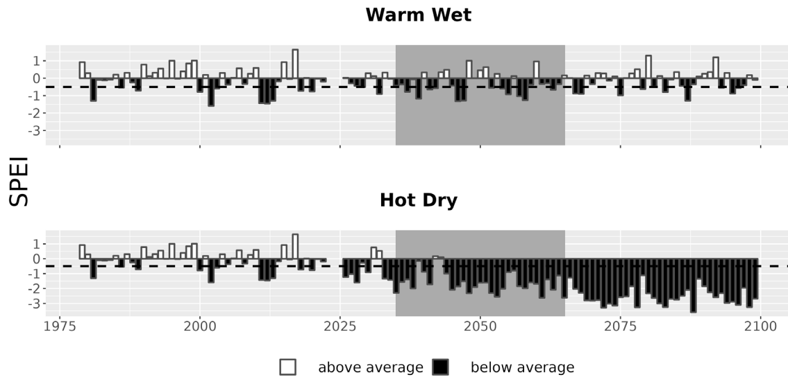
Figure 7. Drought metrics for BEOL. Drought index (SPEI; units = standard deviations from historical) timeseries for each climate future. Below-average SPEI (black bars) indicates dry conditions. The dotted line (SPEI = -0.5) indicates drought conditions.
