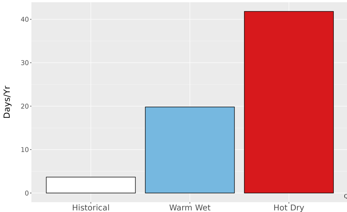
Figure 5. Metrics of extreme temperature at BAND. The bar graph represents the average number of days annually with temperatures greater than the historical 99th percentile (92.9 °F) historically (1979-2012) and for the two climate futures (2050).
