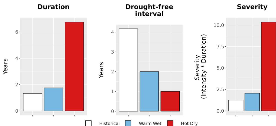
Figure 8. Drought metrics for BAND. (Left) Average drought duration (years) historically (1979-2012) and under each climate future. (Middle) Average drought return interval (years), indicating the expected amount of time between periods of drought, historically and under each climate future. (Right) Average drought severity, a measure of drought intensity multiplied by duration, historically and under each climate future.
