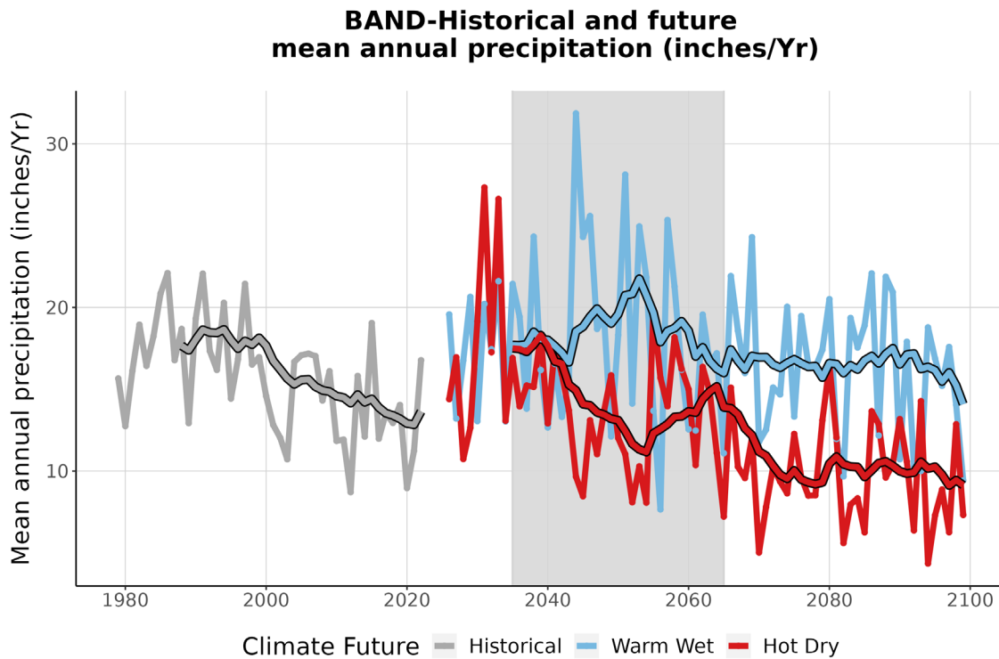
Figure 4. This graph compares observed average annual precipitation at BAND (inches/year) (1979-2022) with projected average annual precipitation for the two climate futures over the period 2023-2099. The historically observed data is shown in gray, the Warm Wet climate future in blue, and the Hot Dry climate future in red. The smooth line running through each projection is the 10-year running average for historical observations and future projections. The gray-shaded area represents the time period that was averaged (2035-2065) to summarize future projections for the year 2050 (Appendix 1).
