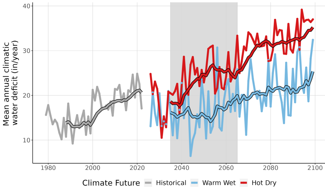
Figure 9. This line graph compares observed climatic water deficit at BAND (inches/year) (1979-2022) with projected climatic water deficit for the two climate futures over the period 2023-2099. The historical observation data is shown in gray, the Warm Wet climate future in blue, and the Hot Dry climate future in red. The smooth line running through each projection is the 10-year running average for historical observations and future projections. Gray-shaded area represents the time period that was averaged (2035-2065) to summarize future projections for the year 2050.
