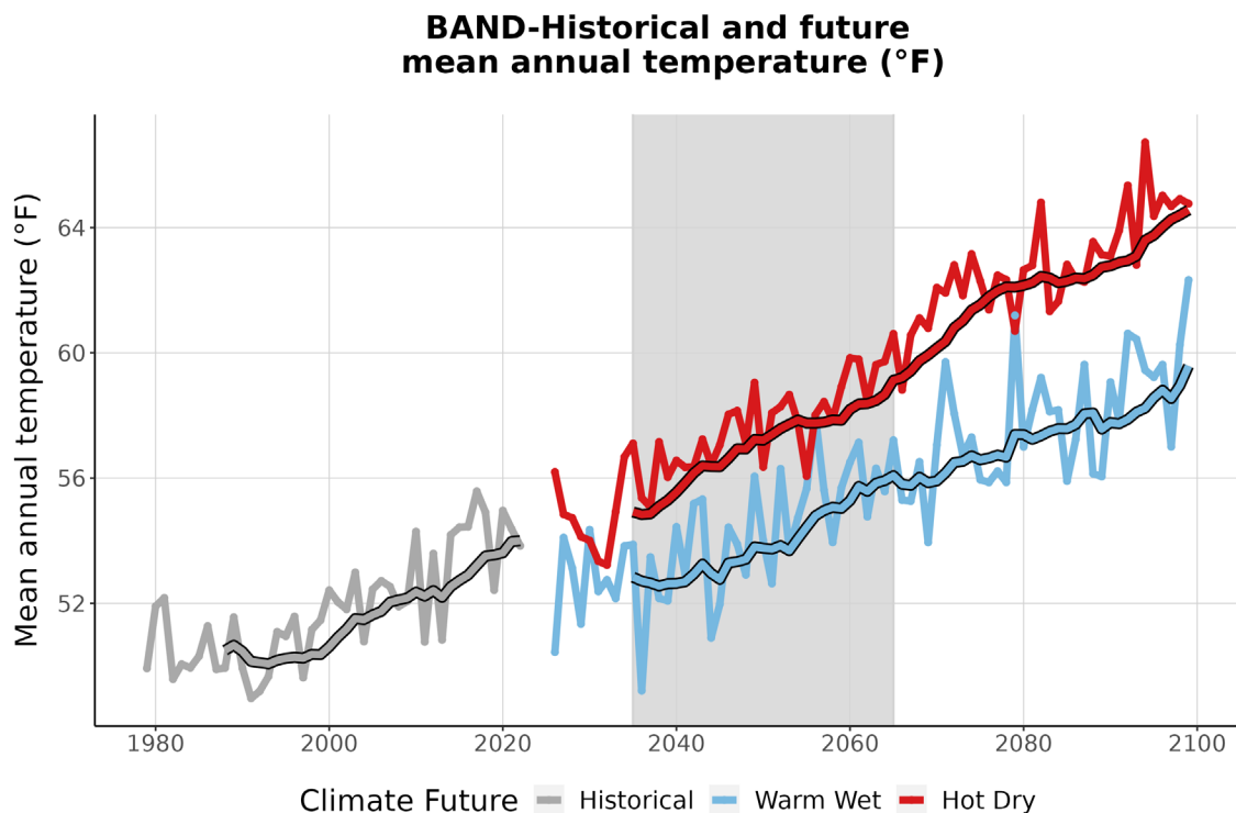
Figure 3. This graph compares observed average annual temperature at BAND (°F) (1979-2022) with projected average annual temperature for the two climate futures over the period 2023-2099. The historically observed data
