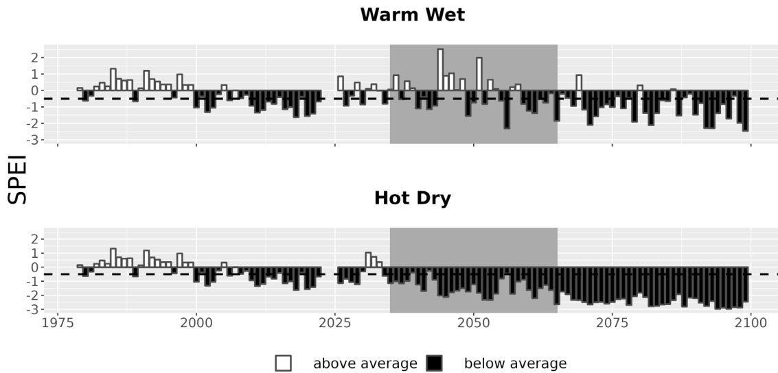
Figure 7. Drought metrics for BAND. Drought index (SPEI; units = standard deviations from historical) timeseries for each climate future. Below-average SPEI (black bars) indicates dry conditions. The dotted line (SPEI = -0.5) indicates drought conditions.
