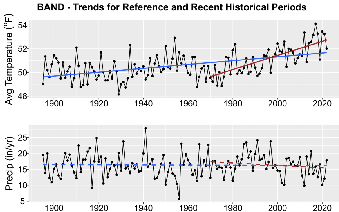
Figure 1. Historical trends in annual average temperature (upper plot) and annual total precipitation (lower plot) for BAND from 1895-2022. Black points show yearly values while blue lines are linear regressions for the entire period record and red lines for 1970-2022 trends. Solid lines are significant trends (i.e., p < 0.05 ); dashed lines are not statistically significant.
