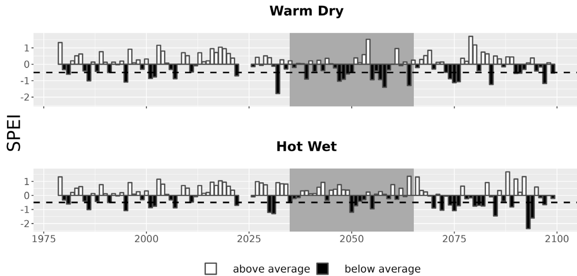
Figure 7. Drought metrics for ASIS. Drought index (SPEI; units = standard deviations from historical) timeseries for each climate future. Below-average SPEI (black bars) indicates dry conditions. The dotted line (SPEI = -0.5) indicates drought conditions.
