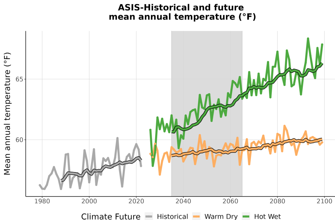
Figure 3. This graph compares observed average annual temperature at ASIS (°F) (1979-2022) with projected average annual temperature for the two climate futures over the period 2023-2099. The historically observed data
