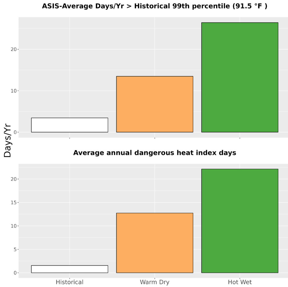
Figure 5. The upper bar graph represents the average number of days annually with temperatures greater than the historical 99th percentile (91.5 °F) historically (1979-2012) and for the two climate futures (2050). The bottom bar graph represents the average annual number of dangerous heat index days historically and for the two climate futures. Dangerous heat index days are days that exceed 105 °F.
