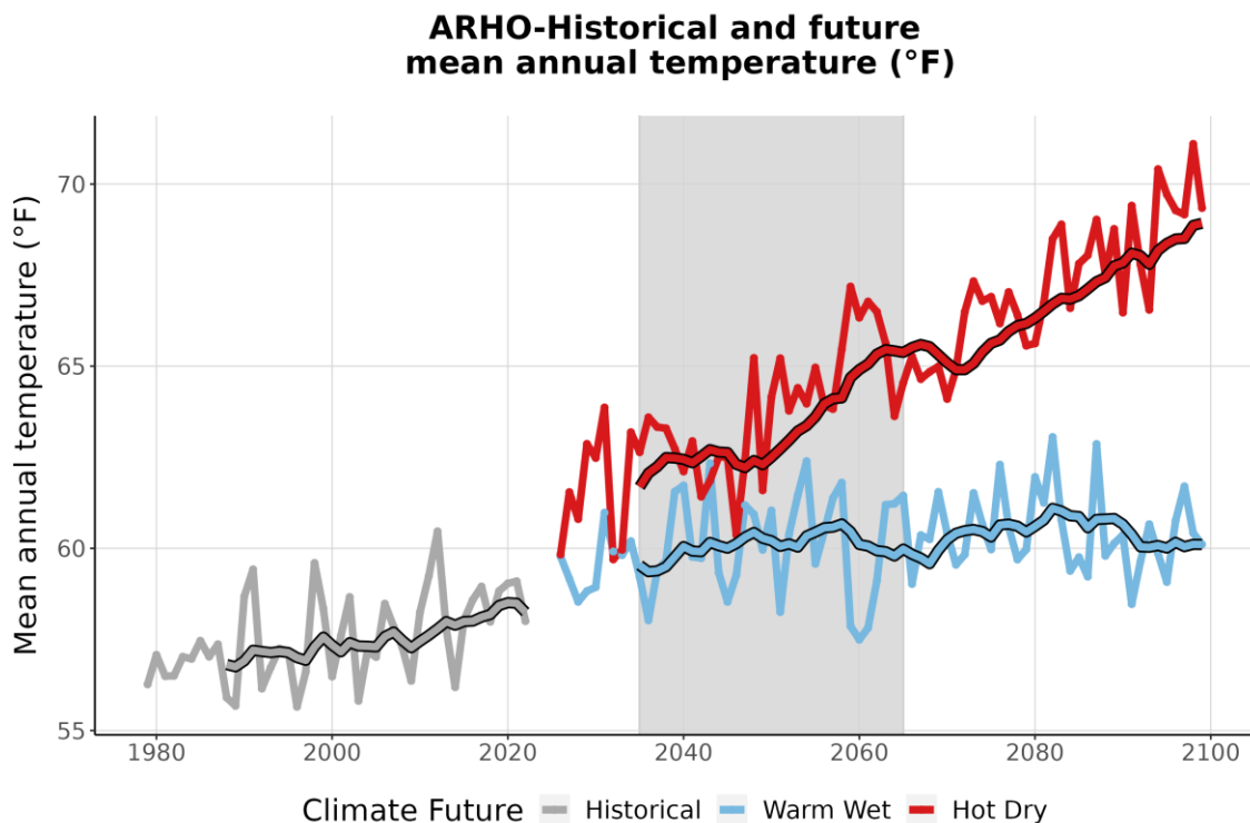
Figure 3. This graph compares observed average annual temperature at ARHO (°F) (1979-2022) with projected average annual temperature for the two climate futures over the period 2023-2099. The historically observed data
