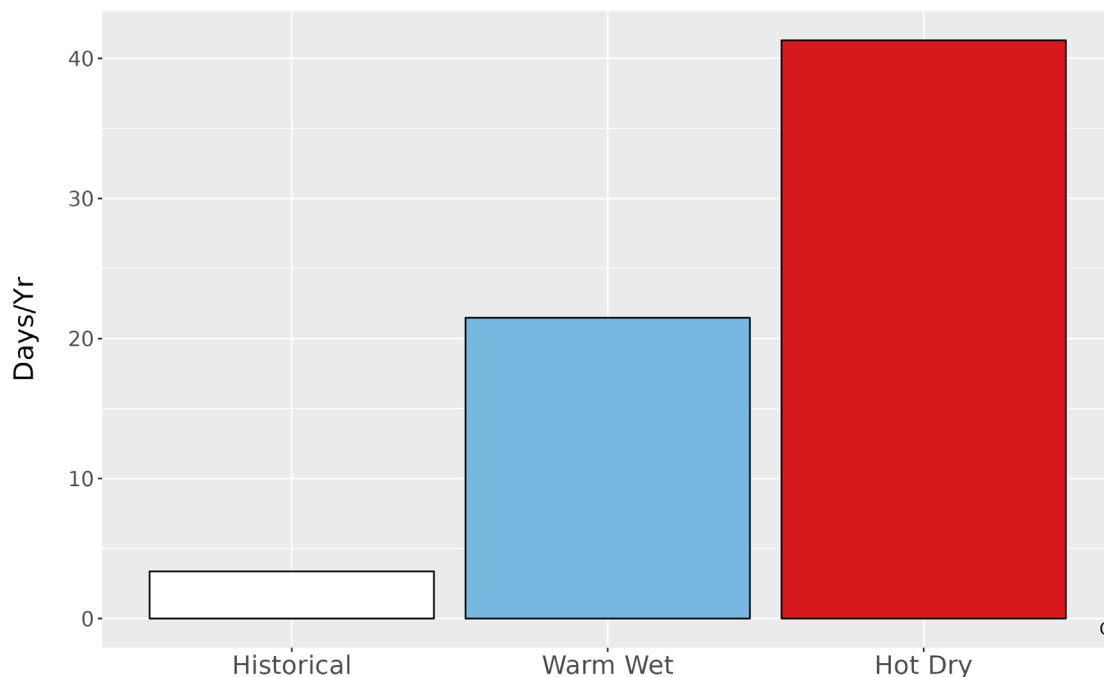
Figure 5. Metrics of extreme temperature at ARCH. The bar graph represents the average number of days annually with temperatures greater than the historical 99th percentile (101 °F) historically (1979-2012) and for the two climate futures (2050).
