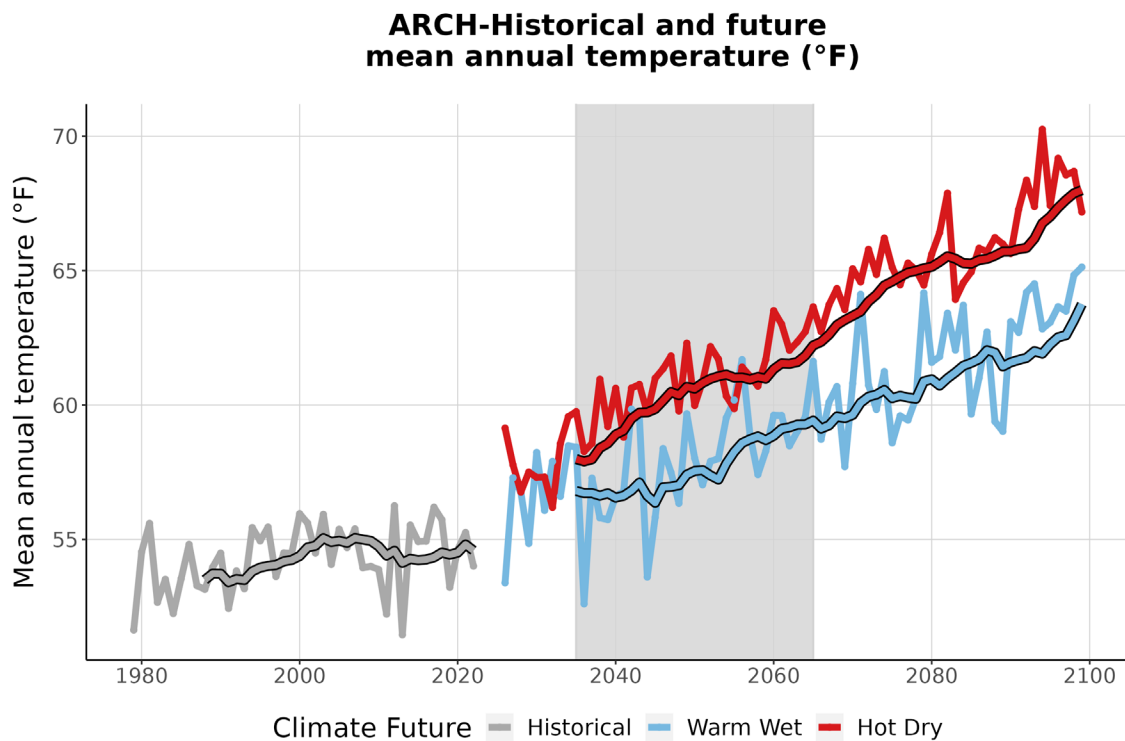
Figure 3. This graph compares observed average annual temperature at ARCH (°F) (1979-2022) with projected average annual temperature for the two climate futures over the period 2023-2099. The historically observed data is shown in gray, the Warm Wet climate future in blue, and the Hot Dry climate future in red. The smooth line
