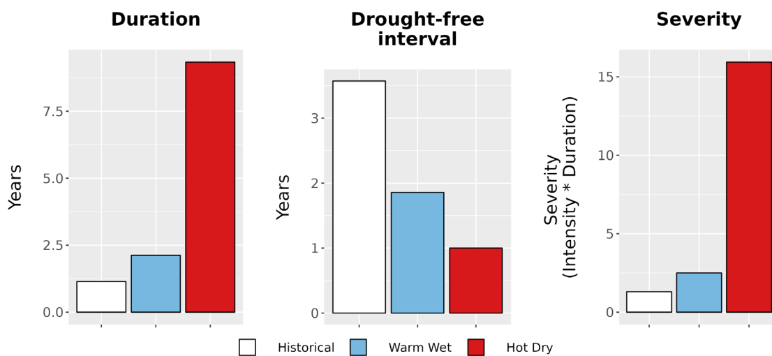
Figure 8. Drought metrics for ARCH. (Left) Average drought duration (years) historically (1979-2012) and under each climate future. (Middle) Average drought return interval (years), indicating the expected amount of time between periods of drought, historically and under each climate future. (Right) Average drought severity, a measure of drought intensity multiplied by duration, historically and under each climate future.
