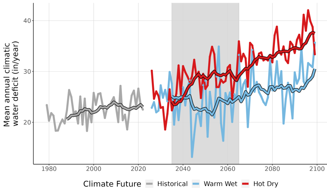
Figure 9. This line graph compares observed climatic water deficit at ARCH (inches/year) (1979-2022) with projected climatic water deficit for the two climate futures over the period 2023-2099. The historical observation data is shown in gray, the Warm Wet climate future in blue, and the Hot Dry climate future in red. The smooth line running through each projection is the 10-year running average for historical observations and future projections. Gray-shaded area represents the time period that was averaged (2035-2065) to summarize future projections for the year 2050.
