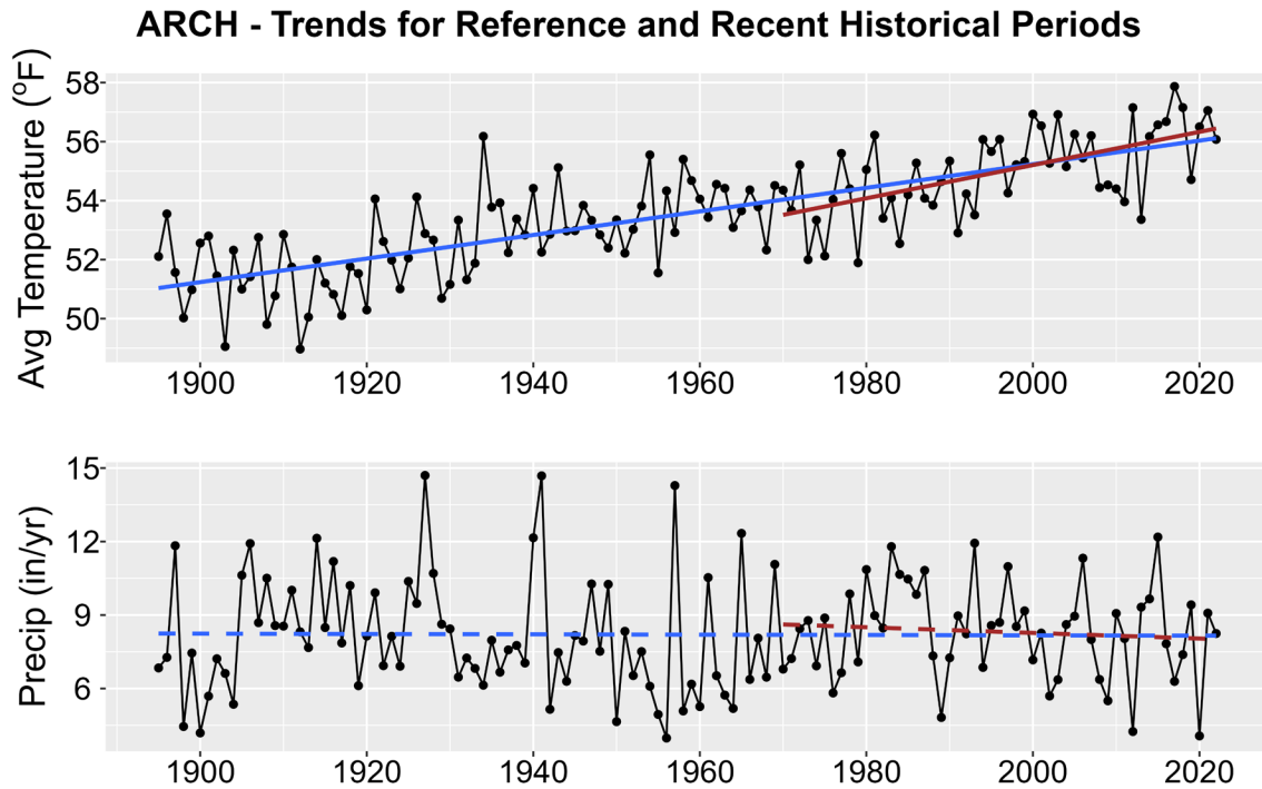
Figure 1. Historical trends in annual average temperature (upper plot) and annual total precipitation (lower plot) for ARCH from 1895-2022. Black points show yearly values while blue lines are linear regressions for the entire period record and red lines for 1970-2022 trends. Solid lines are significant trends (i.e., p < 0.05 ); dashed lines are not statistically significant.
