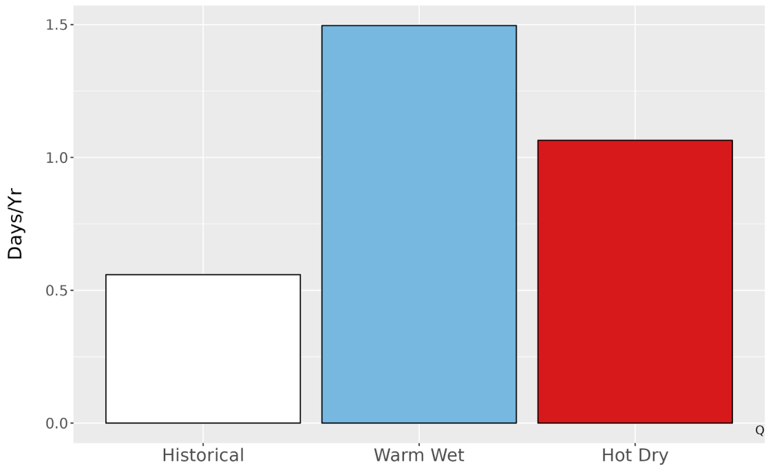
Figure 6. Average number of days annually with precipitation exceeding the 99th percentile (0.6 in.) of precipitation from the historical period 1979-2012 and for each climate future.
