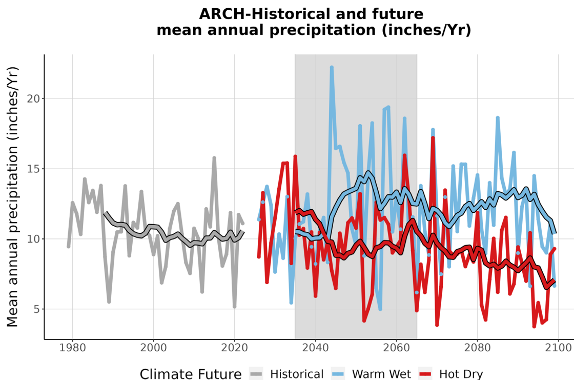
Figure 4. This graph compares observed average annual precipitation at ARCH (inches/year) (1979-2022) with projected average annual precipitation for the two climate futures over the period 2023-2099. The historically observed data is shown in gray, the Warm Wet climate future in blue, and the Hot Dry climate future in red. The smooth line running through each projection is the 10-year running average for historical observations and future projections. The gray-shaded area represents the time period that was averaged (2035-2065) to summarize future projections for the year 2050 (Appendix 1).
