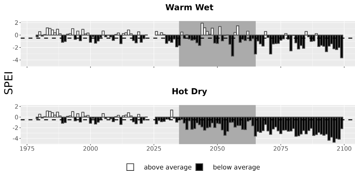
Figure 7. Drought metrics for ARCH. Drought index (SPEI; units = standard deviations from historical) timeseries for each climate future. Below-average SPEI (black bars) indicates dry conditions. The dotted line (SPEI = -0.5) indicates drought conditions.
