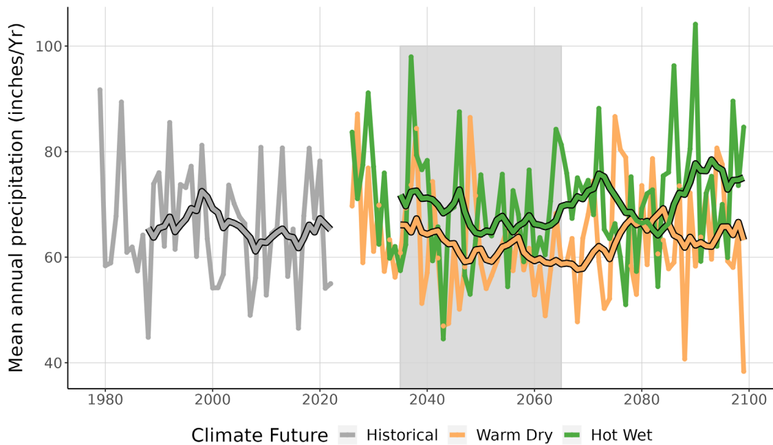
Figure 4. This graph compares observed average annual precipitation at APPA (inches/year) (1979-2022) with projected average annual precipitation for the two climate futures over the period 2023-2099. The historically observed data is shown in gray, the Warm Dry climate future in orange, and the Hot Wet climate future in green. The smooth line running through each projection is the 10-year running average for historical observations and future projections. The gray-shaded area represents the time period that was averaged (2035-2065) to summarize future projections for the year 2050 (Appendix 1).
