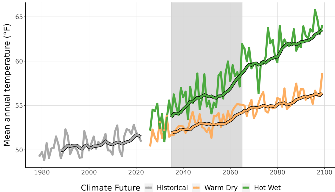
Figure 3. This graph compares observed average annual temperature at APPA (°F) (1979-2022) with projected average annual temperature for the two climate futures over the period 2023-2099. The historically observed data is shown in gray, the Warm Dry climate future in orange, and the Hot Wet climate future in green. The smooth line running through each projection is the 10-year running average for historical observations and future projections. Gray-shaded area represents the time period that was averaged (2035-2065) to summarize future projections for the year 2050 (Appendix 1).
