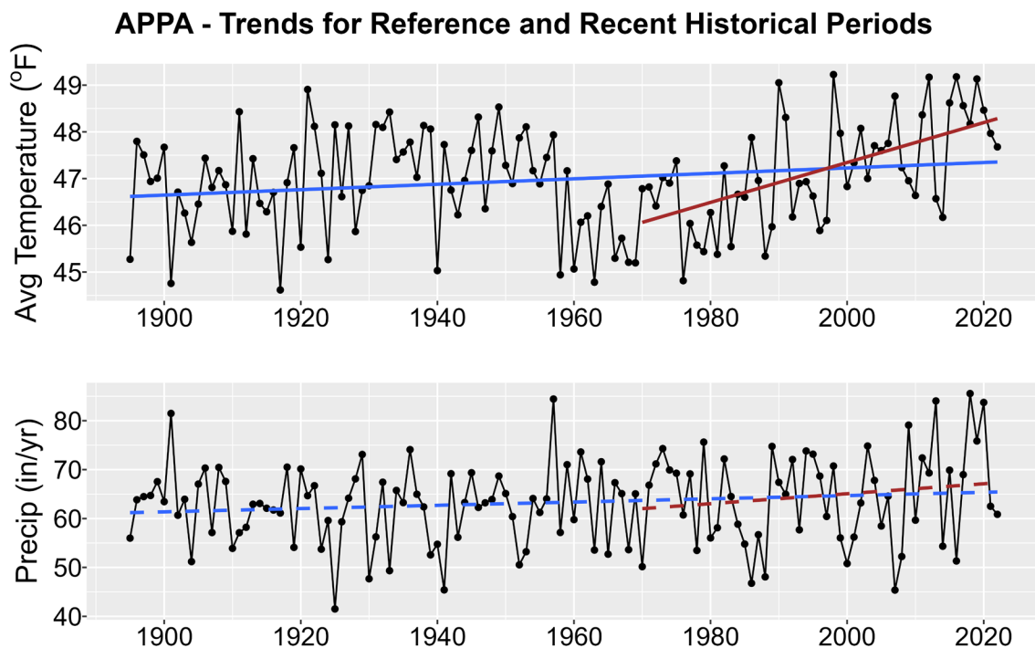
Figure 1. Historical trends in annual average temperature (upper plot) and annual total precipitation (lower plot) for APPA from 1895-2022. Black points show yearly values while blue lines are linear regressions for the entire
