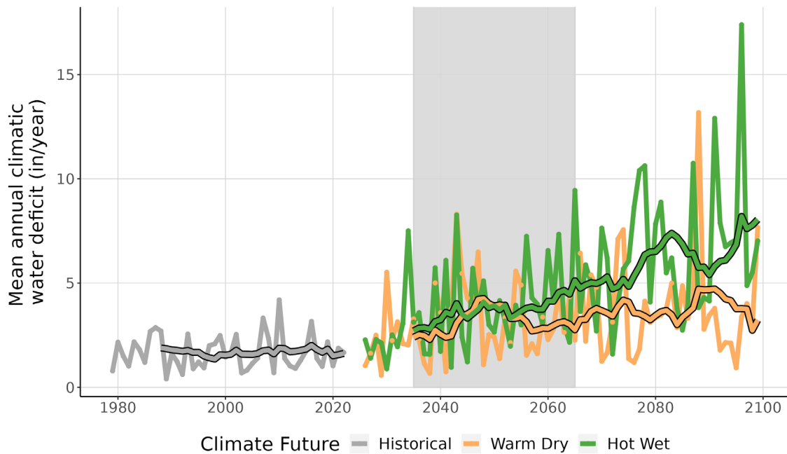
Figure 9. This line graph compares observed climatic water deficit at APPA (inches/year) (1979-2022) with projected climatic water deficit for the two climate futures over the period 2023-2099. The historical observation data is shown in gray, the Warm Dry climate future in orange, and the Hot Wet climate future in green. The smooth line running through each projection is the 10-year running average for historical observations and future projections. Gray-shaded area represents the time period that was averaged (2035-2065) to summarize future projections for the year 2050.
