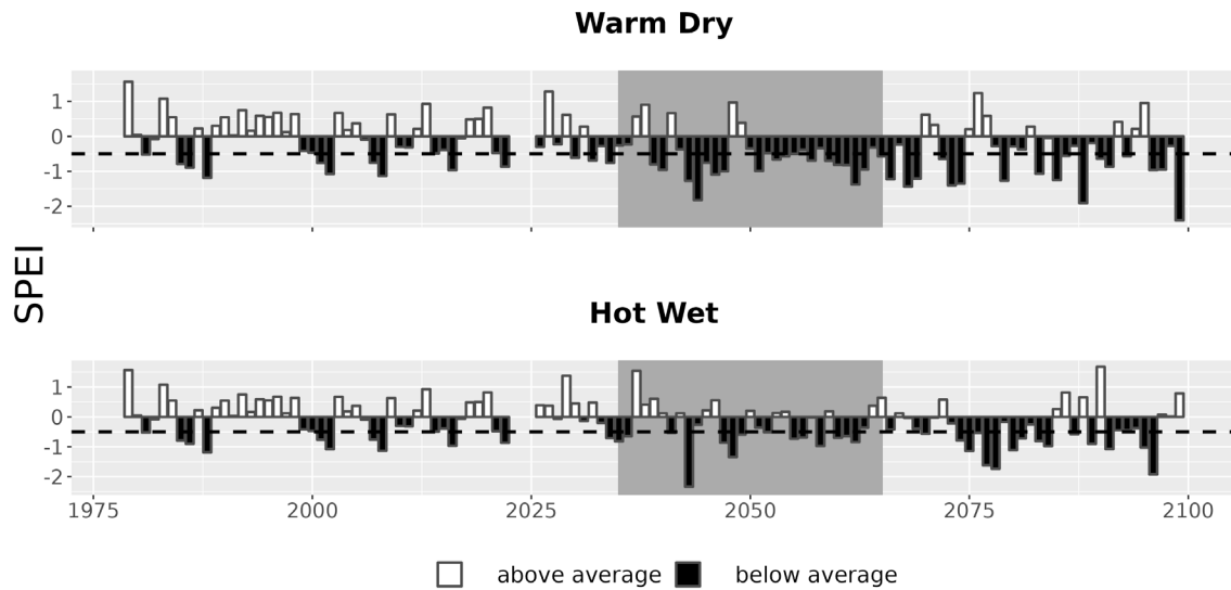
Figure 7. Drought metrics for APPA. Drought index (SPEI; units = standard deviations from historical) timeseries for each climate future. Below-average SPEI (black bars) indicates dry conditions. The dotted line (SPEI = -0.5) indicates drought conditions.
