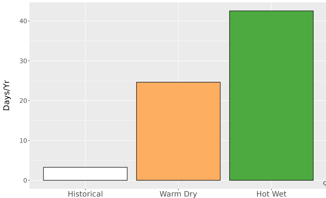
Figure 5. Metrics of extreme temperature at APPA. The bar graph represents the average number of days annually with temperatures greater than the historical 99th percentile (83 °F) historically (1979-2012) and for the two climate futures (2050).
