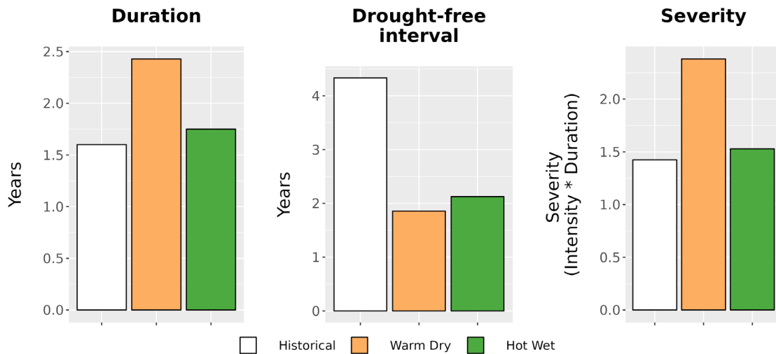
Figure 8. Drought metrics for APPA. (Left) Average drought duration (years) historically (1979-2012) and under each climate future. (Middle) Average drought return interval (years), indicating the expected amount of time between periods of drought, historically and under each climate future. (Right) Average drought severity, a measure of drought intensity multiplied by duration, historically and under each climate future.
