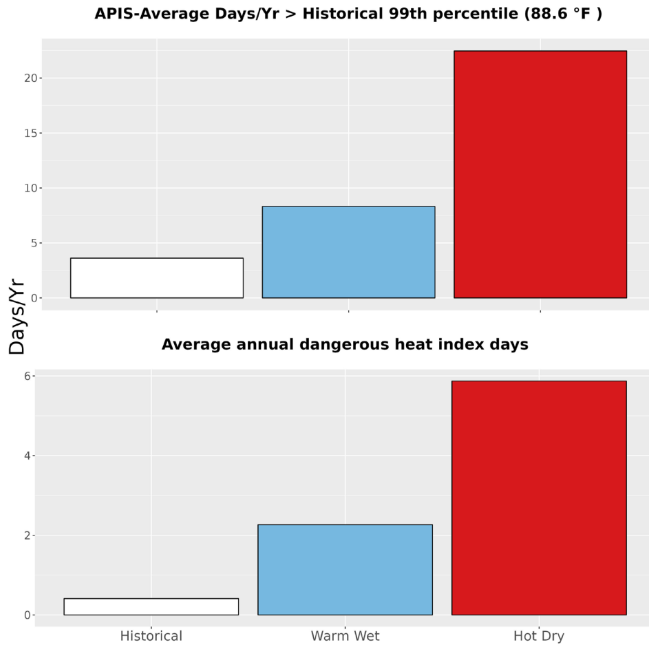
Figure 5. The upper bar graph represents the average number of days annually with temperatures greater than the historical 99th percentile (88.6 °F) historically (1979-2012) and for the two climate futures (2050). The bottom bar graph represents the average annual number of dangerous heat index days historically and for the two climate futures. Dangerous heat index days are days that exceed 105 °F.
