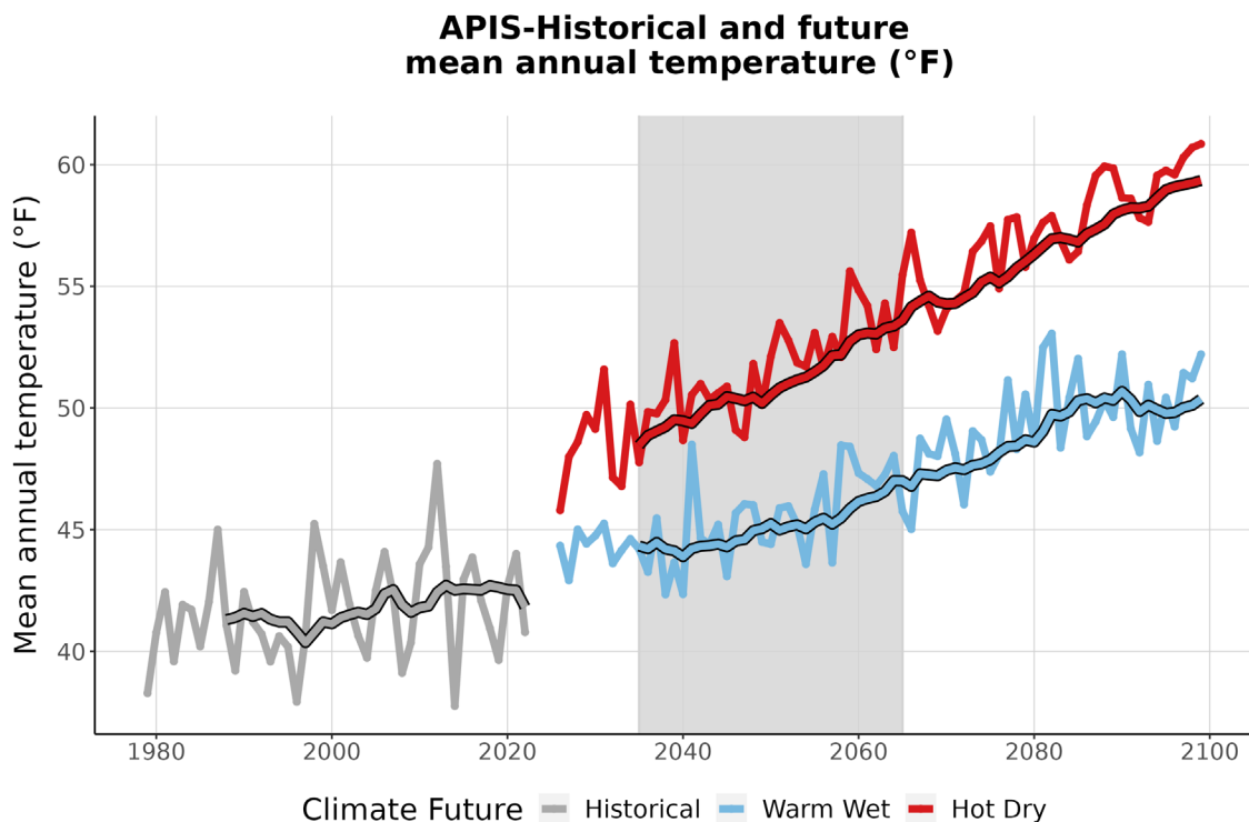
Figure 3. This graph compares observed average annual temperature at APIS (°F) (1979-2022) with projected average annual temperature for the two climate futures over the period 2023-2099. The historically observed data
