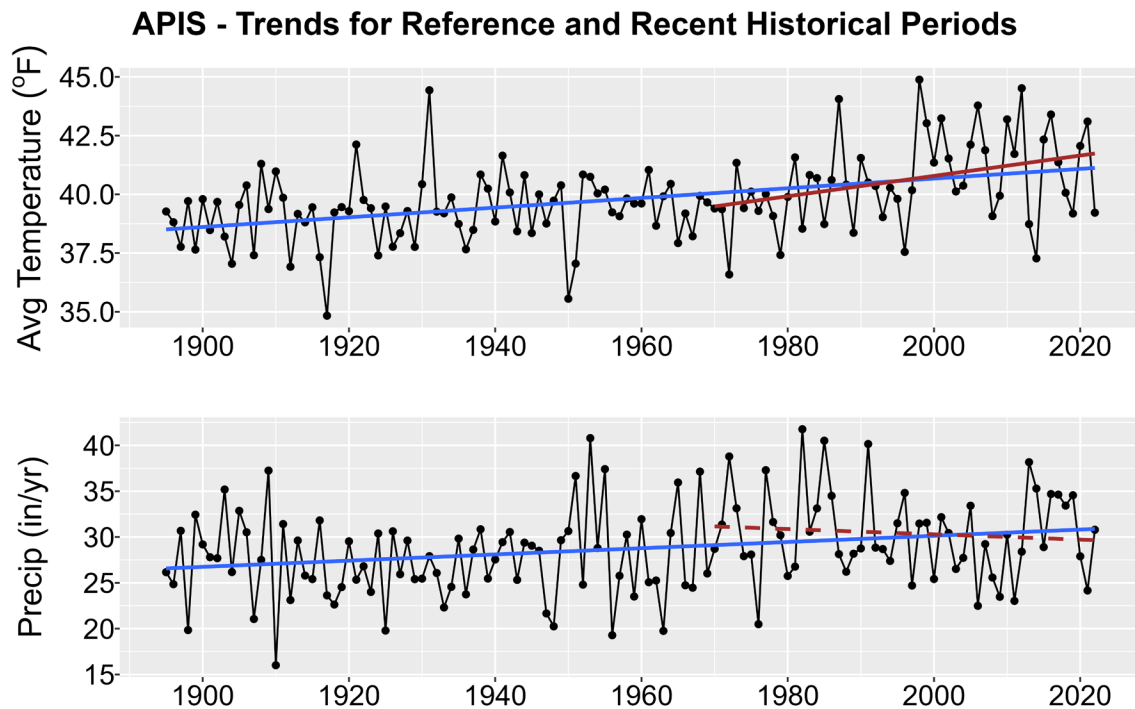
Figure 1. Historical trends in annual average temperature (upper plot) and annual total precipitation (lower plot) for APIS from 1895-2022. Black points show yearly values while blue lines are linear regressions for the entire period record and red lines for 1970-2022 trends. Solid lines are significant trends (i.e., p < 0.05 ); dashed lines are not statistically significant.
