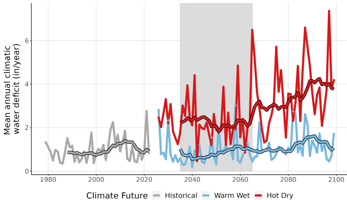
Figure 9. This line graph compares observed climatic water deficit at APIS (inches/year) (1979-2022) with projected climatic water deficit for the two climate futures over the period 2023-2099. The historical observation data is shown in gray, the Warm Wet climate future in blue, and the Hot Dry climate future in red. The smooth line running through each projection is the 10-year running average for historical observations and future projections. Gray-shaded area represents the time period that was averaged (2035-2065) to summarize future projections for the year 2050.
