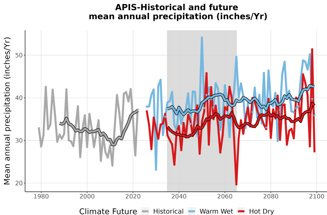
Figure 4. This graph compares observed average annual precipitation at APIS (inches/year) (1979-2022) with projected average annual precipitation for the two climate futures over the period 2023-2099. The historically observed data is shown in gray, the Warm Wet climate future in blue, and the Hot Dry climate future in red. The smooth line running through each projection is the 10-year running average for historical observations and future projections. The gray-shaded area represents the time period that was averaged (2035-2065) to summarize future projections for the year 2050 (Appendix 1).
