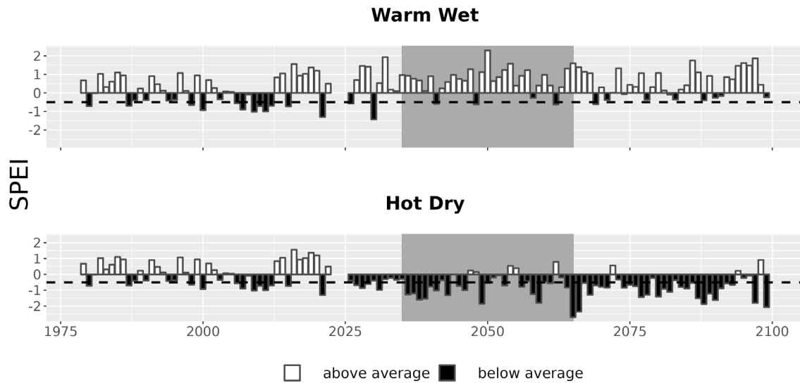
Figure 7. Drought metrics for APIS. Drought index (SPEI; units = standard deviations from historical) timeseries for each climate future. Below-average SPEI (black bars) indicates dry conditions. The dotted line (SPEI = -0.5) indicates drought conditions.
