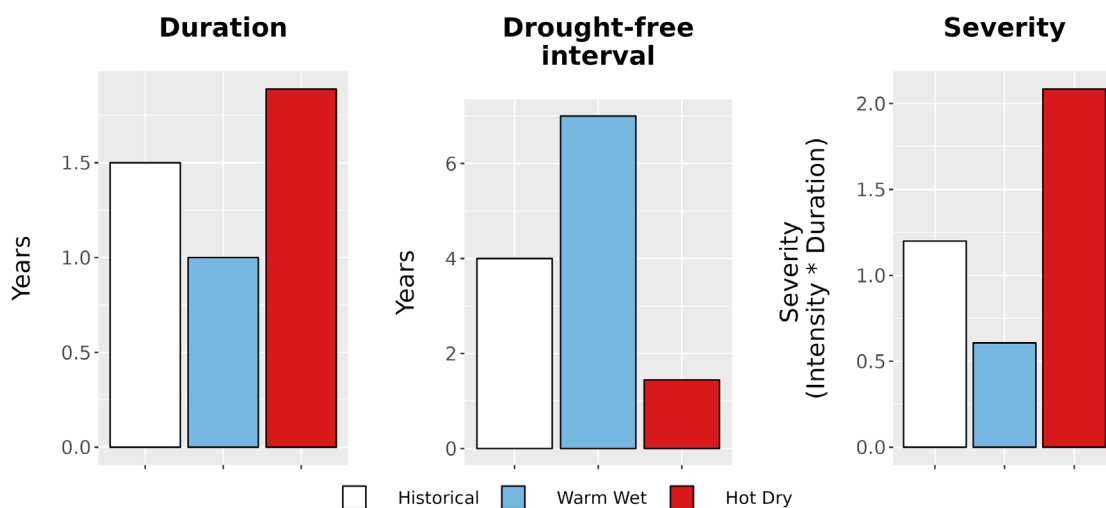
Figure 8. Drought metrics for APIS. (Left) Average drought duration (years) historically (1979-2012) and under each climate future. (Middle) Average drought return interval (years), indicating the expected amount of time between periods of drought, historically and under each climate future. (Right) Average drought severity, a measure of drought intensity multiplied by duration, historically and under each climate future.
