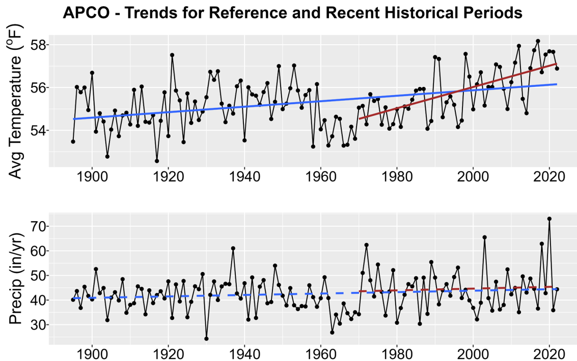
Figure 1. Historical trends in annual average temperature (upper plot) and annual total precipitation (lower plot) for APCO from 1895-2022. Black points show yearly values while blue lines are linear regressions for the entire period record and red lines for 1970-2022 trends. Solid lines are significant trends (i.e., p < 0.05 ); dashed lines are not statistically significant.
