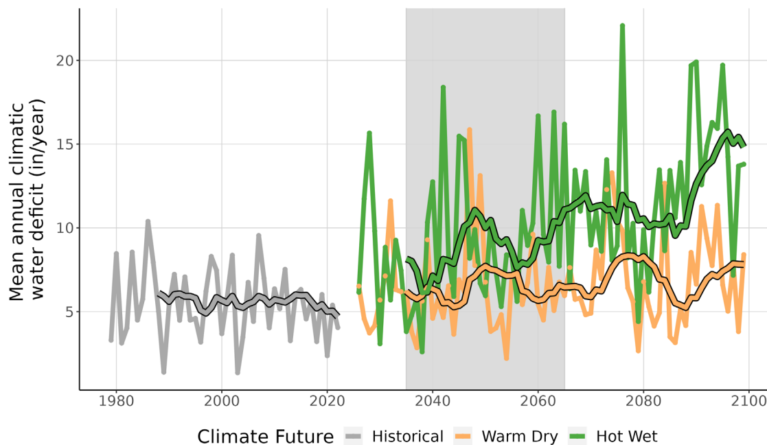
Figure 9. This line graph compares observed climatic water deficit at APCO (inches/year) (1979-2022) with projected climatic water deficit for the two climate futures over the period 2023-2099. The historical observation data is shown in gray, the Warm Dry climate future in orange, and the Hot Wet climate future in green. The smooth line running through each projection is the 10-year running average for historical observations and future projections. Gray-shaded area represents the time period that was averaged (2035-2065) to summarize future projections for the year 2050.
