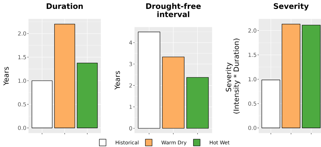
Figure 8. Drought metrics for APCO. (Left) Average drought duration (years) historically (1979-2012) and under each climate future. (Middle) Average drought return interval (years), indicating the expected amount of time between periods of drought, historically and under each climate future. (Right) Average drought severity, a measure of drought intensity multiplied by duration, historically and under each climate future.
