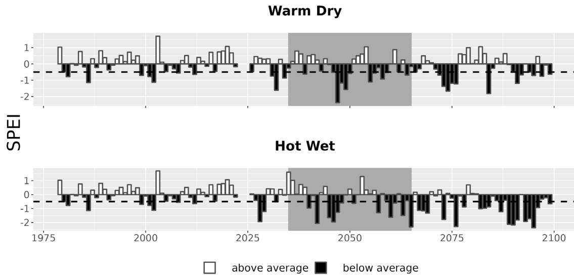
Figure 7. Drought metrics for APCO. Drought index (SPEI; units = standard deviations from historical) timeseries for each climate future. Below-average SPEI (black bars) indicates dry conditions. The dotted line (SPEI = -0.5) indicates drought conditions.
