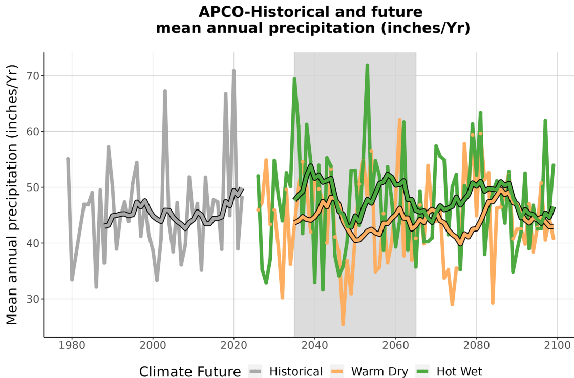
Figure 4. This graph compares observed average annual precipitation at APCO (inches/year) (1979-2022) with projected average annual precipitation for the two climate futures over the period 2023-2099. The historically observed data is shown in gray, the Warm Dry climate future in orange, and the Hot Wet climate future in green. The smooth line running through each projection is the 10-year running average for historical observations and future projections. The gray-shaded area represents the time period that was averaged (2035-2065) to summarize future projections for the year 2050 (Appendix 1).
