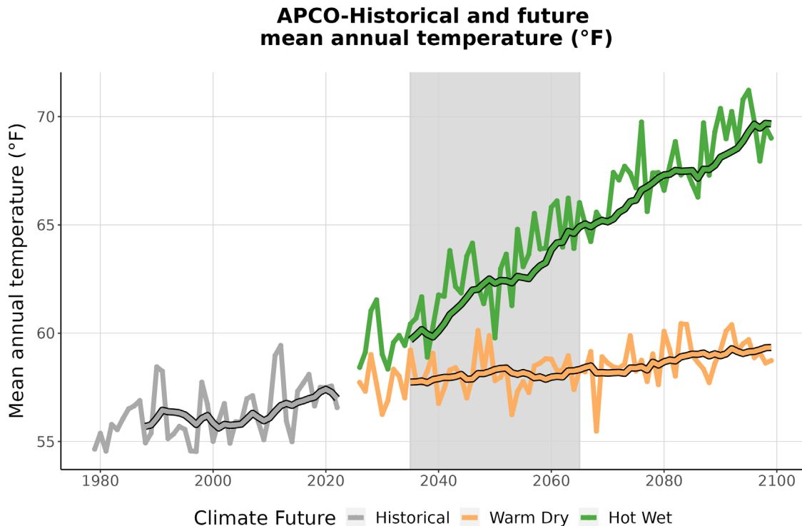
Figure 3. This graph compares observed average annual temperature at APCO (°F) (1979-2022) with projected average annual temperature for the two climate futures over the period 2023-2099. The historically observed data
