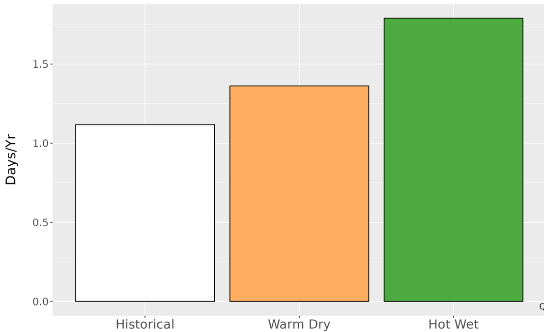
Figure 6. Average number of days annually with precipitation exceeding the 99th percentile (2 in.) of precipitation from the historical period 1979-2012 and for each climate future.
