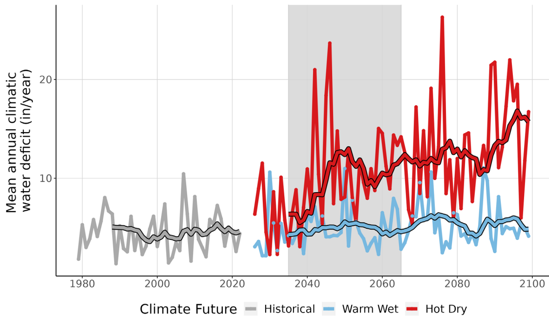
Figure 9. This line graph compares observed climatic water deficit at ANJO (inches/year) (1979-2022) with projected climatic water deficit for the two climate futures over the period 2023-2099. The historical observation data is shown in gray, the Warm Wet climate future in blue, and the Hot Dry climate future in red. The smooth line running through each projection is the 10-year running average for historical observations and future projections. Gray-shaded area represents the time period that was averaged (2035-2065) to summarize future projections for the year 2050.
