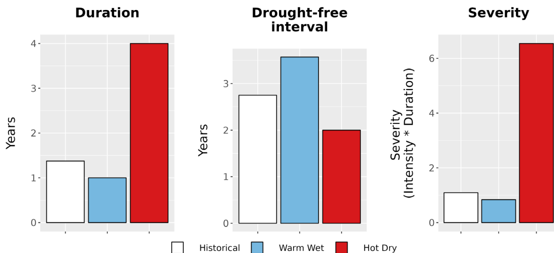
Figure 8. Drought metrics for ANDE. (Left) Average drought duration (years) historically (1979-2012) and under each climate future. (Middle) Average drought return interval (years), indicating the expected amount of time between periods of drought, historically and under each climate future. (Right) Average drought severity, a measure of drought intensity multiplied by duration, historically and under each climate future.
