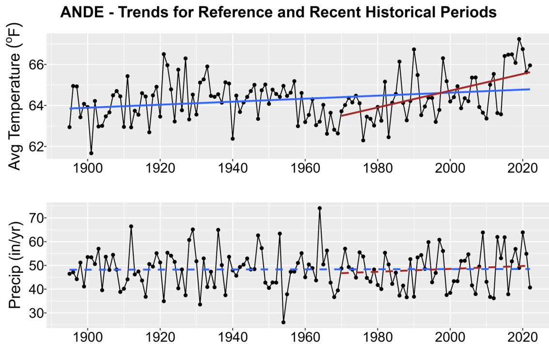
Figure 1. Historical trends in annual average temperature (upper plot) and annual total precipitation (lower plot) for ANDE from 1895-2022. Black points show yearly values while blue lines are linear regressions for the entire period record and red lines for 1970-2022 trends. Solid lines are significant trends (i.e., p < 0.05 ); dashed lines are not statistically significant.
