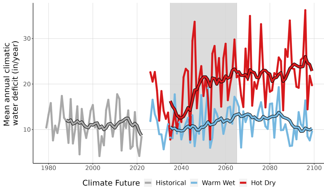
Figure 9. This line graph compares observed climatic water deficit at ANDE (inches/year) (1979-2022) with projected climatic water deficit for the two climate futures over the period 2023-2099. The historical observation data is shown in gray, the Warm Wet climate future in blue, and the Hot Dry climate future in red. The smooth line running through each projection is the 10-year running average for historical observations and future projections. Gray-shaded area represents the time period that was averaged (2035-2065) to summarize future projections for the year 2050.
