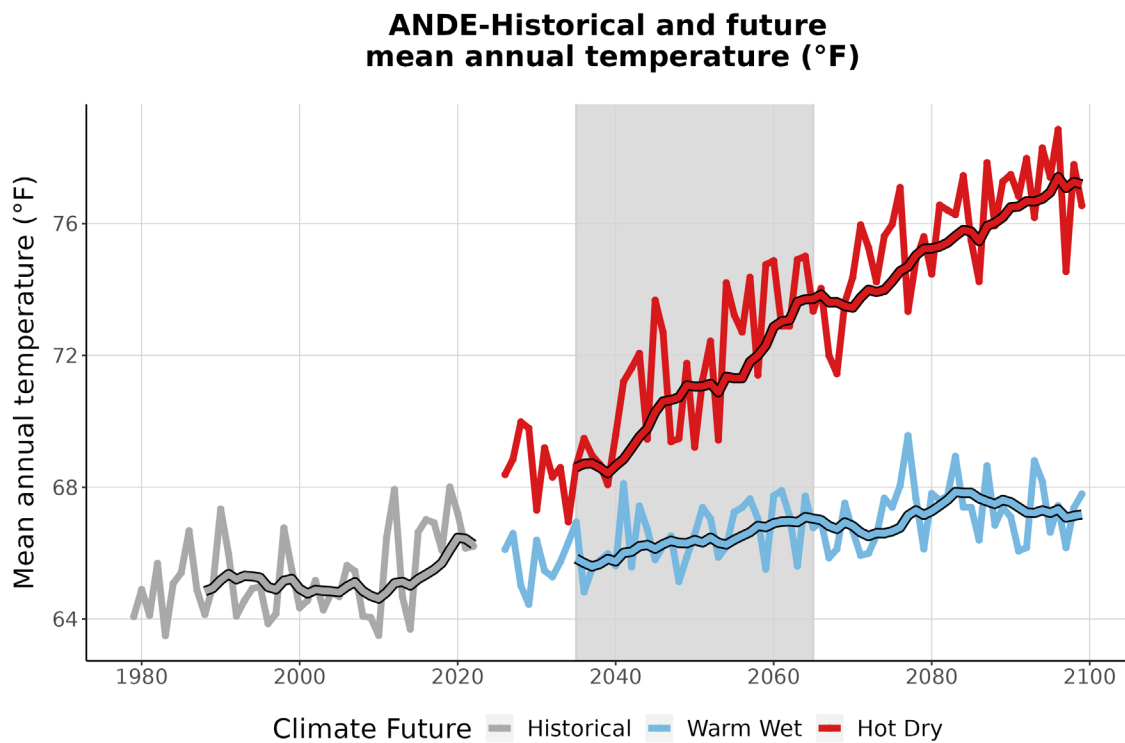
Figure 3. This graph compares observed average annual temperature at ANDE (°F) (1979-2022) with projected average annual temperature for the two climate futures over the period 2023-2099. The historically observed data
