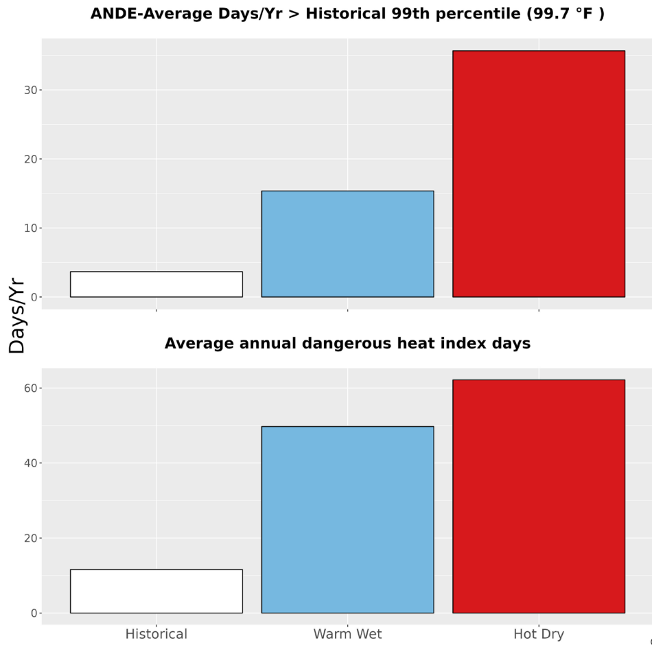
Figure 5. The upper bar graph represents the average number of days annually with temperatures greater than the historical 99th percentile (99.7 °F) historically (1979-2012) and for the two climate futures (2050). The bottom bar graph represents the average annual number of dangerous heat index days historically and for the two climate futures. Dangerous heat index days are days that exceed 105 °F.
