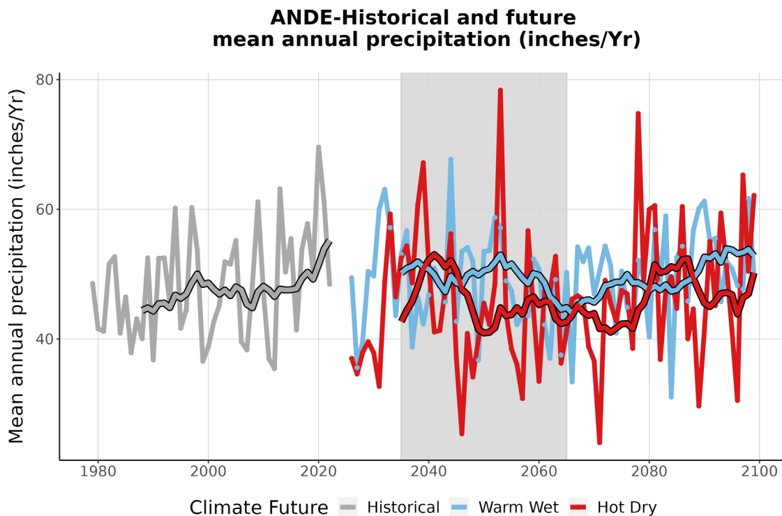
Figure 4. This graph compares observed average annual precipitation at ANDE (inches/year) (1979-2022) with projected average annual precipitation for the two climate futures over the period 2023-2099. The historically observed data is shown in gray, the Warm Wet climate future in blue, and the Hot Dry climate future in red. The smooth line running through each projection is the 10-year running average for historical observations and future projections. The gray-shaded area represents the time period that was averaged (2035-2065) to summarize future projections for the year 2050 (Appendix 1).
