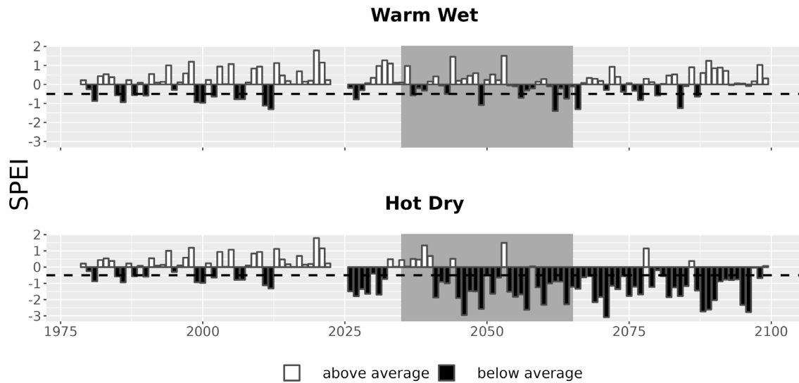
Figure 7. Drought metrics for ANDE. Drought index (SPEI; units = standard deviations from historical) timeseries for each climate future. Below-average SPEI (black bars) indicates dry conditions. The dotted line (SPEI = -0.5) indicates drought conditions.
