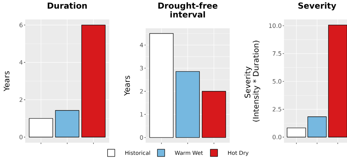
Figure 8. Drought metrics for ALFL. (Left) Average drought duration (years) historically (1979-2012) and under each climate future. (Middle) Average drought return interval (years), indicating the expected amount of time between periods of drought, historically and under each climate future. (Right) Average drought severity, a measure of drought intensity multiplied by duration, historically and under each climate future.
