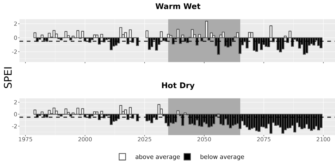
Figure 7. Drought metrics for ALFL. Drought index (SPEI; units = standard deviations from historical) timeseries for each climate future. Below-average SPEI (black bars) indicates dry conditions. The dotted line (SPEI = -0.5) indicates drought conditions.
