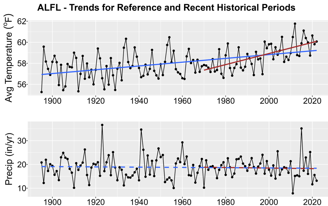
Figure 1. Historical trends in annual average temperature (upper plot) and annual total precipitation (lower plot) for ALFL from 1895-2022. Black points show yearly values while blue lines are linear regressions for the entire period record and red lines for 1970-2022 trends. Solid lines are significant trends (i.e., p < 0.05 ); dashed lines are not statistically significant.
