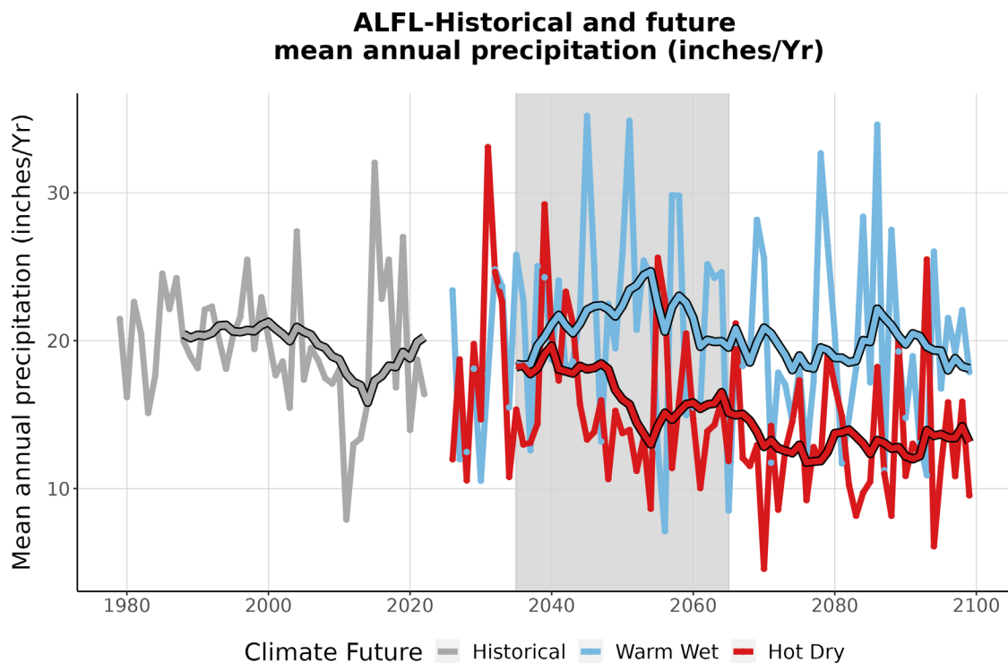
Figure 4. This graph compares observed average annual precipitation at ALFL (inches/year) (1979-2022) with projected average annual precipitation for the two climate futures over the period 2023-2099. The historically observed data is shown in gray, the Warm Wet climate future in blue, and the Hot Dry climate future in red. The smooth line running through each projection is the 10-year running average for historical observations and future projections. The gray-shaded area represents the time period that was averaged (2035-2065) to summarize future projections for the year 2050 (Appendix 1).
