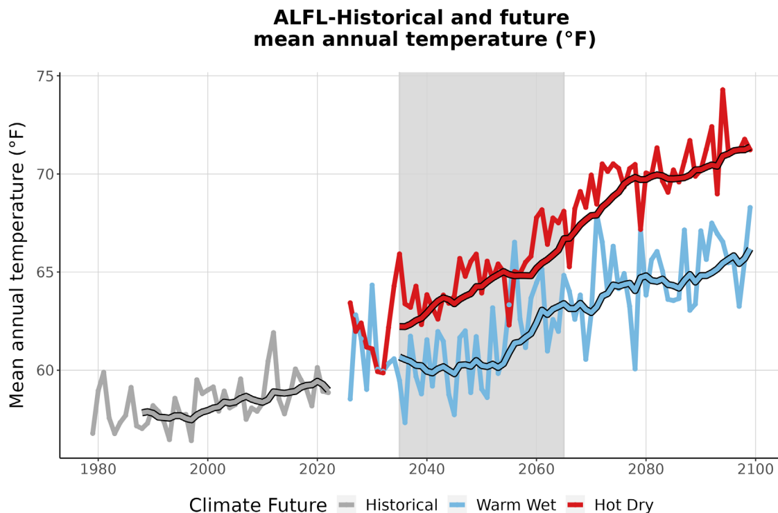
Figure 3. This graph compares observed average annual temperature at ALFL (°F) (1979-2022) with projected average annual temperature for the two climate futures over the period 2023-2099. The historically observed data
