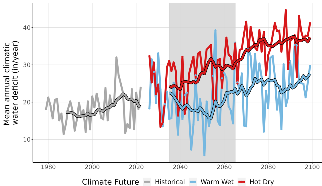
Figure 9. This line graph compares observed climatic water deficit at ALFL (inches/year) (1979-2022) with projected climatic water deficit for the two climate futures over the period 2023-2099. The historical observation data is shown in gray, the Warm Wet climate future in blue, and the Hot Dry climate future in red. The smooth line running through each projection is the 10-year running average for historical observations and future projections. Gray-shaded area represents the time period that was averaged (2035-2065) to summarize future projections for the year 2050.
