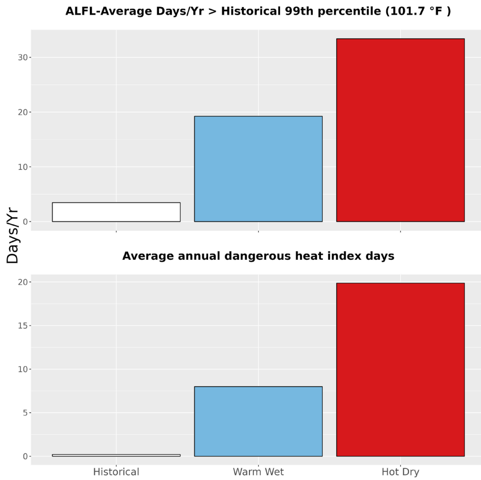
Figure 5. The upper bar graph represents the average number of days annually with temperatures greater than the historical 99th percentile (101.7 °F) historically (1979-2012) and for the two climate futures (2050). The bottom bar graph represents the average annual number of dangerous heat index days historically and for the two climate futures. Dangerous heat index days are days that exceed 105 °F.
