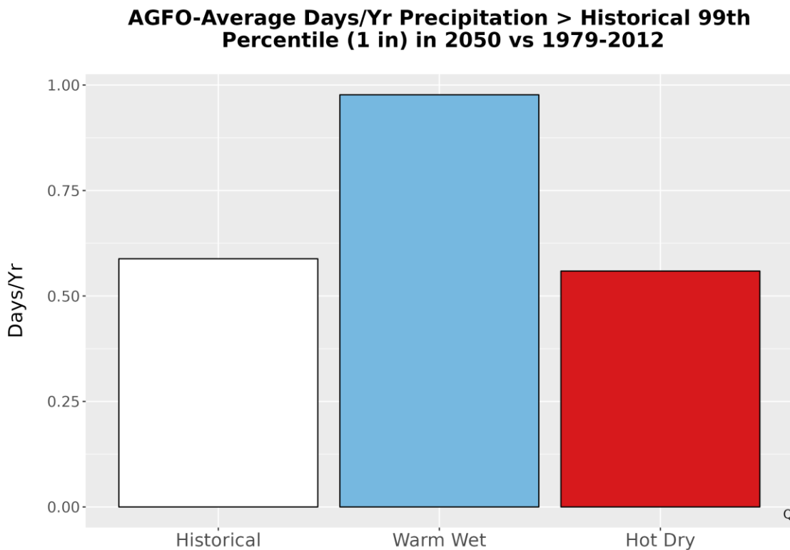
Figure 6. Average number of days annually with precipitation exceeding the 99th percentile (1 in.) of precipitation from the historical period 1979-2012 and for each climate future.
