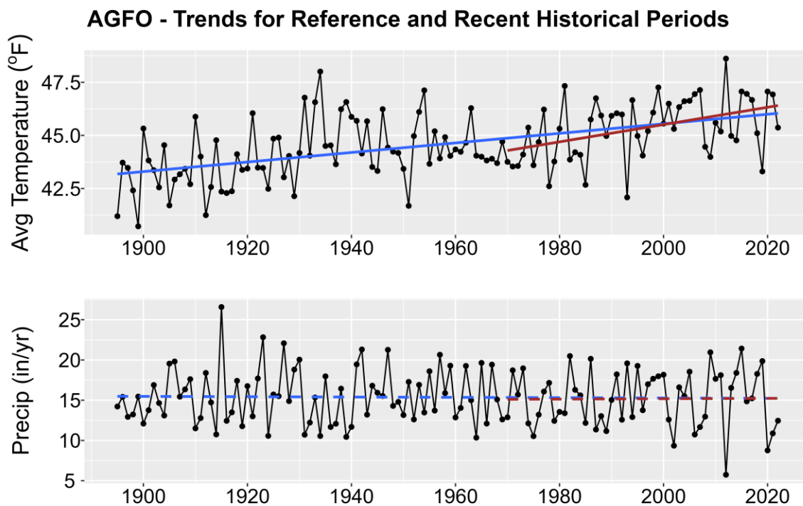
Figure 1. Historical trends in annual average temperature (upper plot) and annual total precipitation (lower plot) for AGFO from 1895-2022. Black points show yearly values while blue lines are linear regressions for the entire period record and red lines for 1970-2022 trends. Solid lines are significant trends (i.e., p < 0.05 ); dashed lines are not statistically significant.
