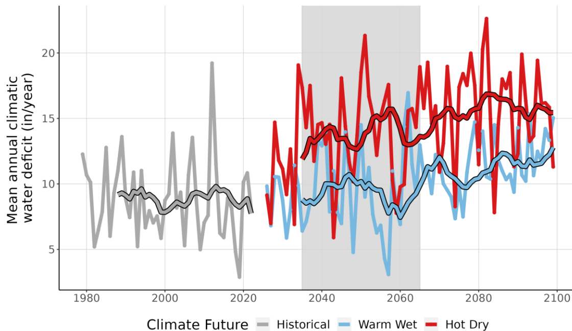
Figure 9. This line graph compares observed climatic water deficit at AGFO (inches/year) (1979-2022) with projected climatic water deficit for the two climate futures over the period 2023-2099. The historical observation data is shown in gray, the Warm Wet climate future in blue, and the Hot Dry climate future in red. The smooth line running through each projection is the 10-year running average for historical observations and future projections. Gray-shaded area represents the time period that was averaged (2035-2065) to summarize future projections for the year 2050.
