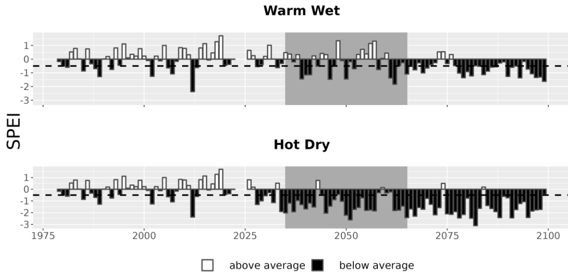
Figure 7. Drought metrics for AGFO. Drought index (SPEI; units = standard deviations from historical) timeseries for each climate future. Below-average SPEI (black bars) indicates dry conditions. The dotted line (SPEI = -0.5) indicates drought conditions.
