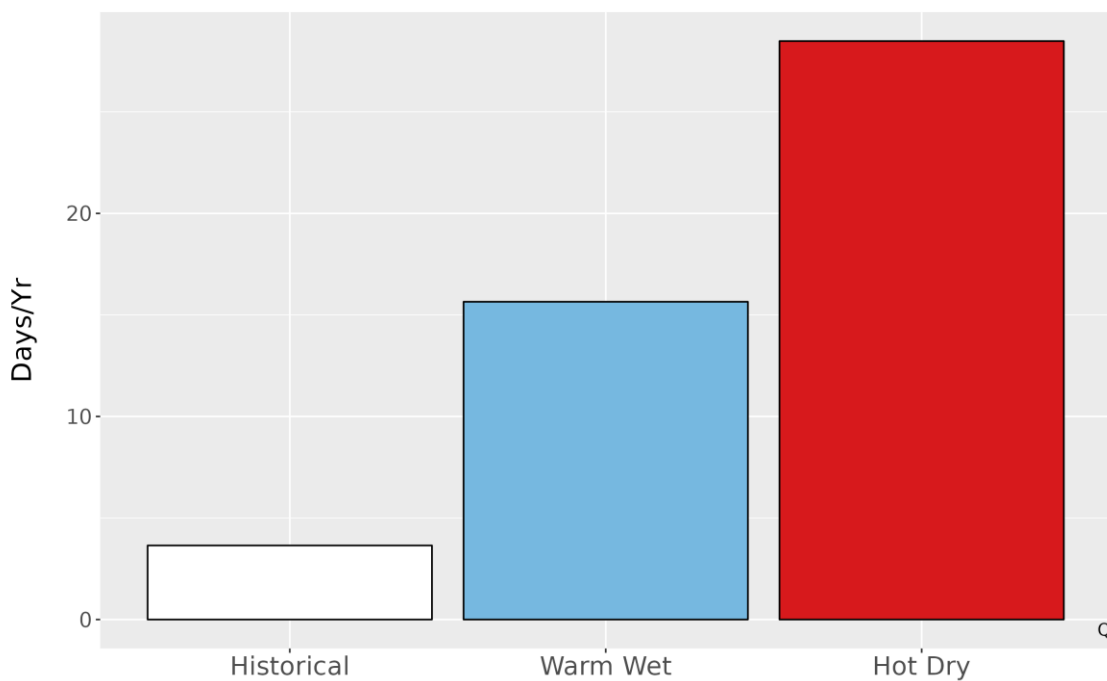
Figure 5. Metrics of extreme temperature at AGFO. The bar graph represents the average number of days annually with temperatures greater than the historical 99th percentile (97.8 °F) historically (1979-2012) and for the two climate futures (2050).
