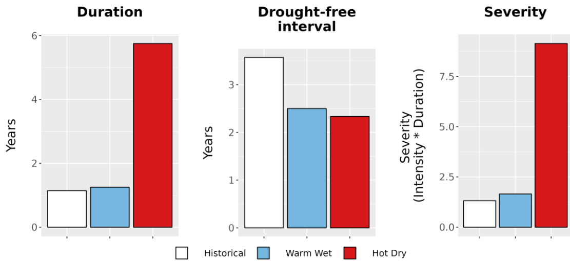
Figure 8. Drought metrics for AGFO. (Left) Average drought duration (years) historically (1979-2012) and under each climate future. (Middle) Average drought return interval (years), indicating the expected amount of time between periods of drought, historically and under each climate future. (Right) Average drought severity, a measure of drought intensity multiplied by duration, historically and under each climate future.
