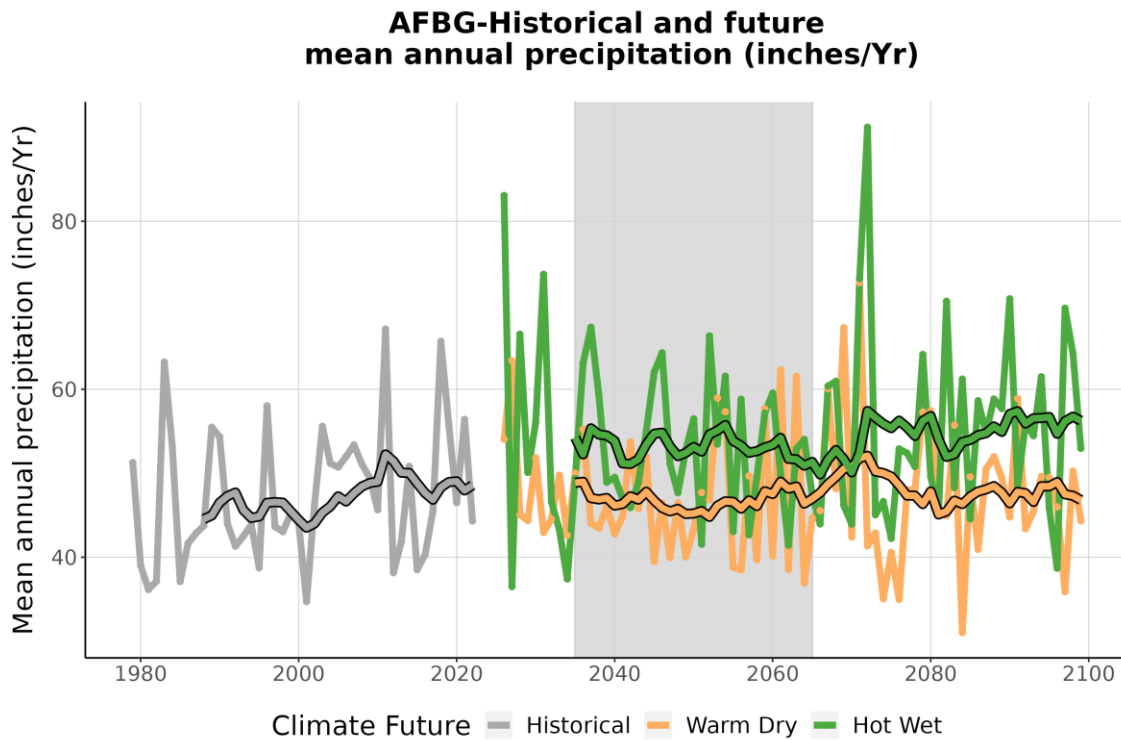
Figure 4. This graph compares observed average annual precipitation at AFBG (inches/year) (1979-2022) with projected average annual precipitation for the two climate futures over the period 2023-2099. The historically observed data is shown in gray, the Warm Dry climate future in orange, and the Hot Wet climate future in green. The smooth line running through each projection is the 10-year running average for historical observations and future projections. The gray-shaded area represents the time period that was averaged (2035-2065) to summarize future projections for the year 2050 (Appendix 1).
