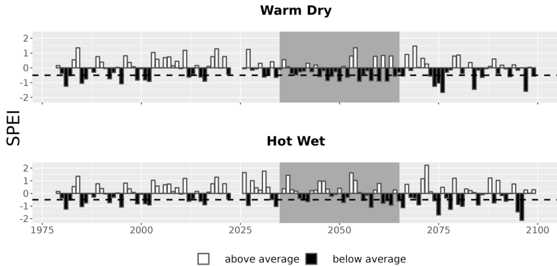
Figure 7. Drought metrics for AFBG. Drought index (SPEI; units = standard deviations from historical) timeseries for each climate future. Below-average SPEI (black bars) indicates dry conditions. The dotted line (SPEI = -0.5) indicates drought conditions.
