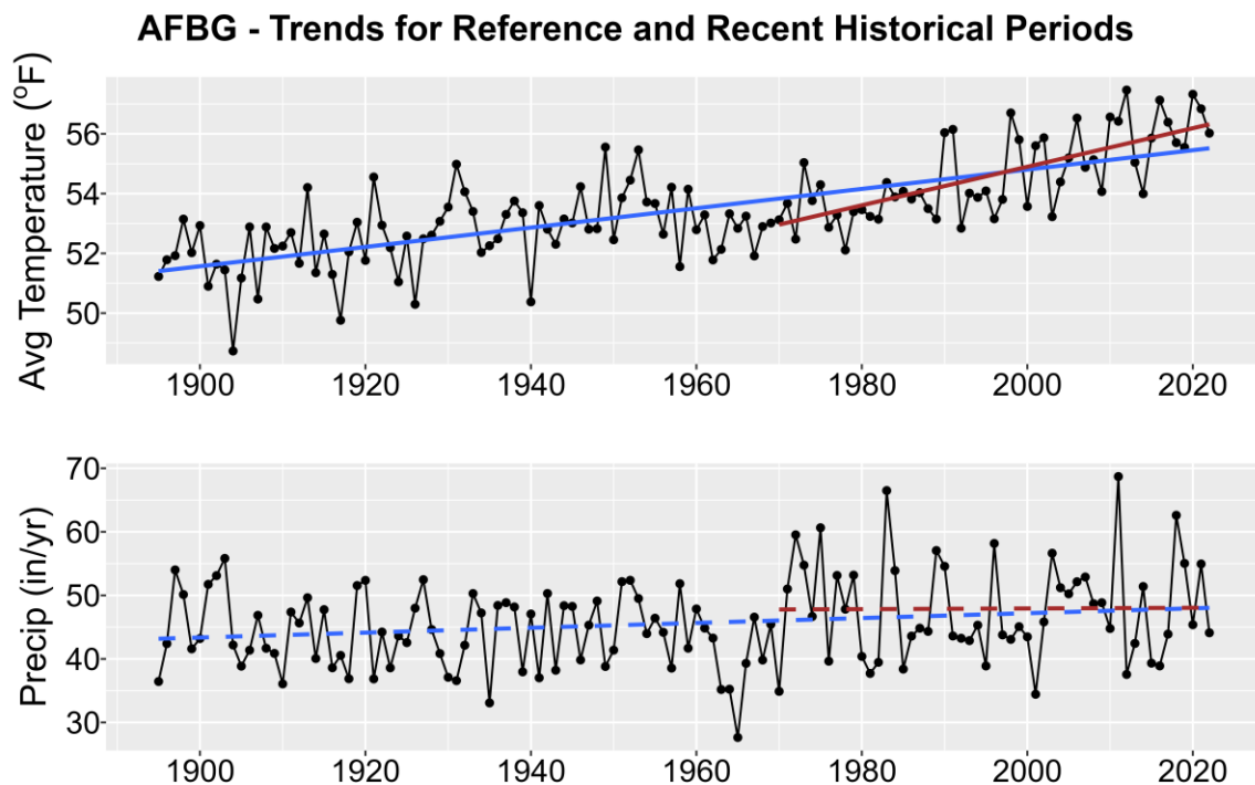
Figure 1. Historical trends in annual average temperature (upper plot) and annual total precipitation (lower plot) for AFBG from 1895-2022. Black points show yearly values while blue lines are linear regressions for the entire period record and red lines for 1970-2022 trends. Solid lines are significant trends (i.e., p < 0.05 ); dashed lines are not statistically significant.
