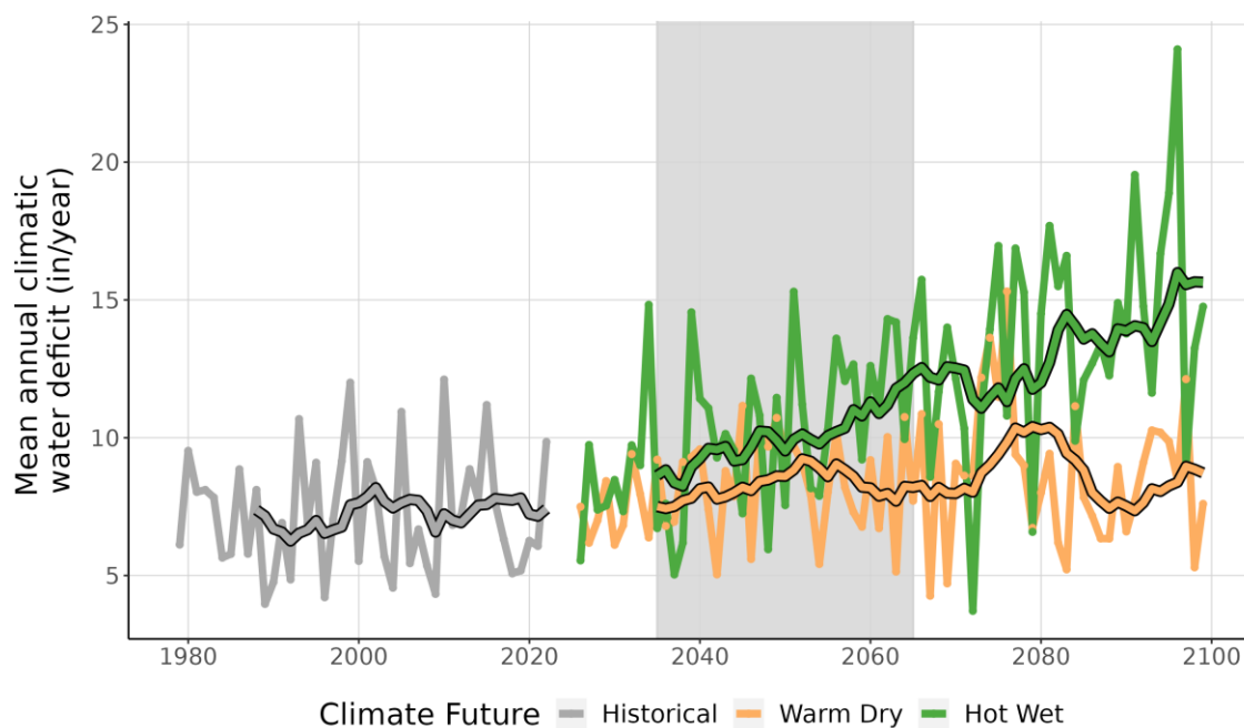
Figure 9. This line graph compares observed climatic water deficit at AFBG (inches/year) (1979-2022) with projected climatic water deficit for the two climate futures over the period 2023-2099. The historical observation data is shown in gray, the Warm Dry climate future in orange, and the Hot Wet climate future in green. The smooth line running through each projection is the 10-year running average for historical observations and future projections. Gray-shaded area represents the time period that was averaged (2035-2065) to summarize future projections for the year 2050.
