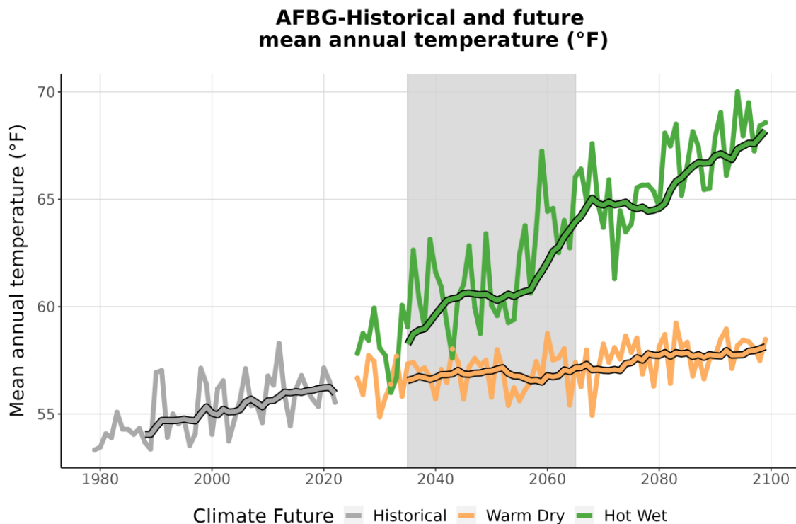
Figure 3. This graph compares observed average annual temperature at AFBG (°F) (1979-2022) with projected average annual temperature for the two climate futures over the period 2023-2099. The historically observed data
