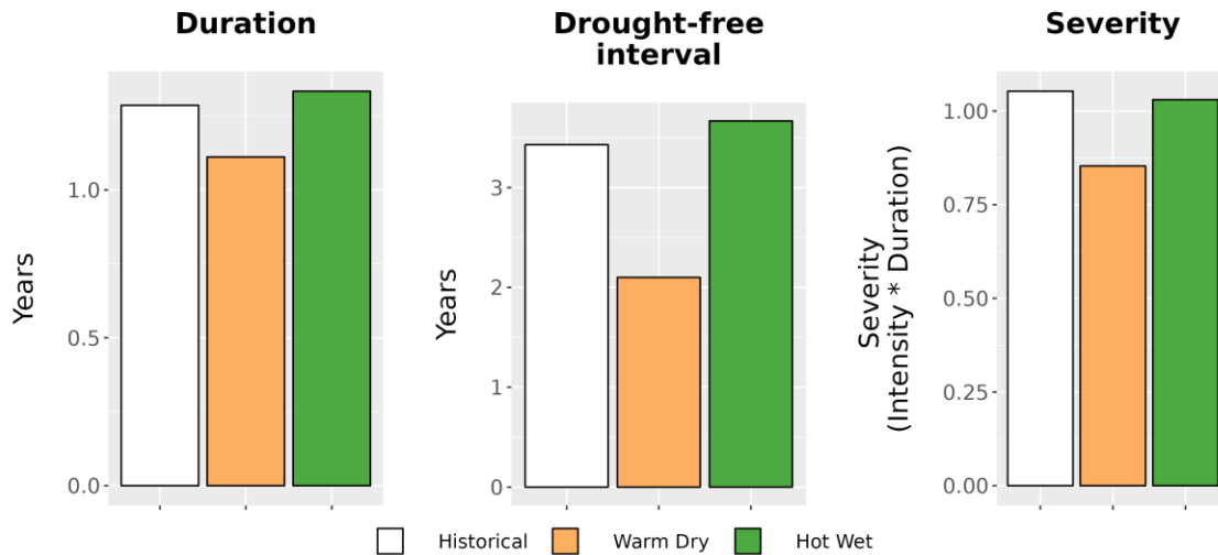
Figure 8. Drought metrics for AFBG. (Left) Average drought duration (years) historically (1979-2012) and under each climate future. (Middle) Average drought return interval (years), indicating the expected amount of time between periods of drought, historically and under each climate future. (Right) Average drought severity, a measure of drought intensity multiplied by duration, historically and under each climate future.
