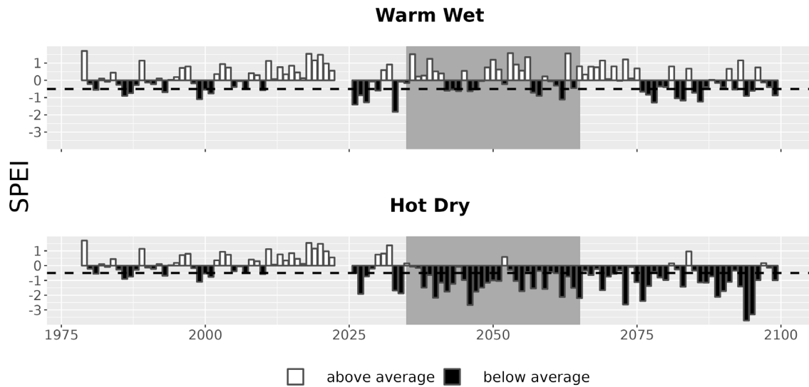
Figure 7. Drought metrics for ABLI. Drought index (SPEI; units = standard deviations from historical) timeseries for each climate future. Below-average SPEI (black bars) indicates dry conditions. The dotted line (SPEI = -0.5) indicates drought conditions.
