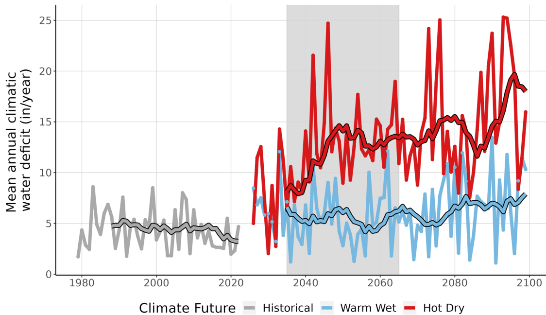
Figure 9. This line graph compares observed climatic water deficit at ABLI (inches/year) (1979-2022) with projected climatic water deficit for the two climate futures over the period 2023-2099. The historical observation data is shown in gray, the Warm Wet climate future in blue, and the Hot Dry climate future in red. The smooth line running through each projection is the 10-year running average for historical observations and future projections. Gray-shaded area represents the time period that was averaged (2035-2065) to summarize future projections for the year 2050.
