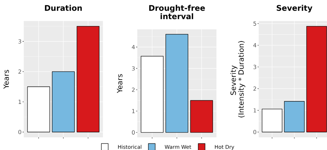
Figure 8. Drought metrics for ABLI. (Left) Average drought duration (years) historically (1979-2012) and under each climate future. (Middle) Average drought return interval (years), indicating the expected amount of time between periods of drought, historically and under each climate future. (Right) Average drought severity, a measure of drought intensity multiplied by duration, historically and under each climate future.
