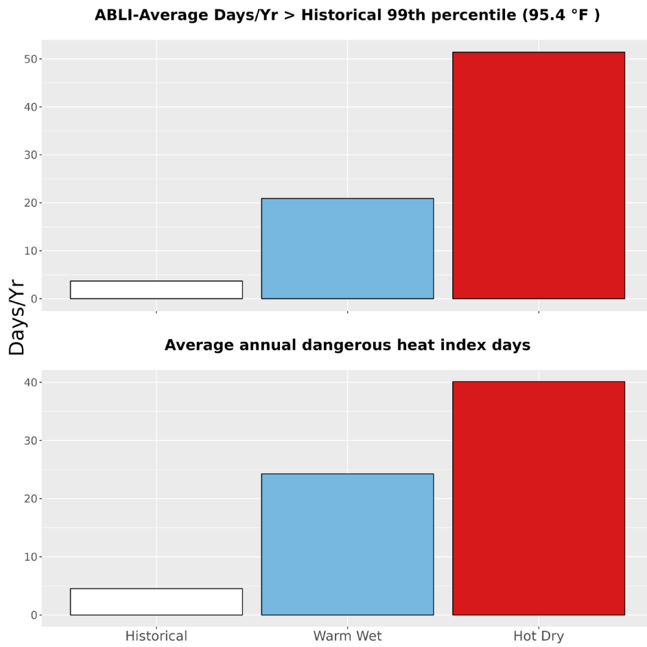
Figure 5. The upper bar graph represents the average number of days annually with temperatures greater than the historical 99th percentile (95.4 °F) historically (1979-2012) and for the two climate futures (2050). The bottom bar graph represents the average annual number of dangerous heat index days historically and for the two climate futures. Dangerous heat index days are days that exceed 105 °F.
