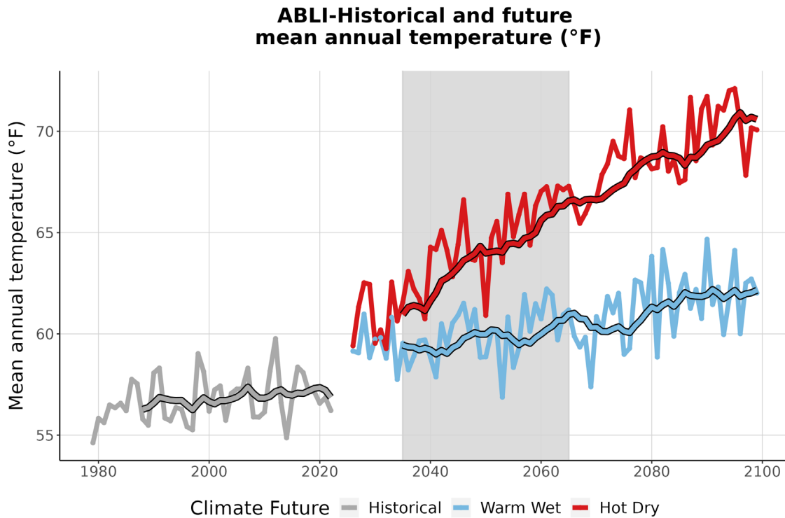
Figure 3. This graph compares observed average annual temperature at ABLI (°F) (1979-2022) with projected average annual temperature for the two climate futures over the period 2023-2099. The historically observed data
