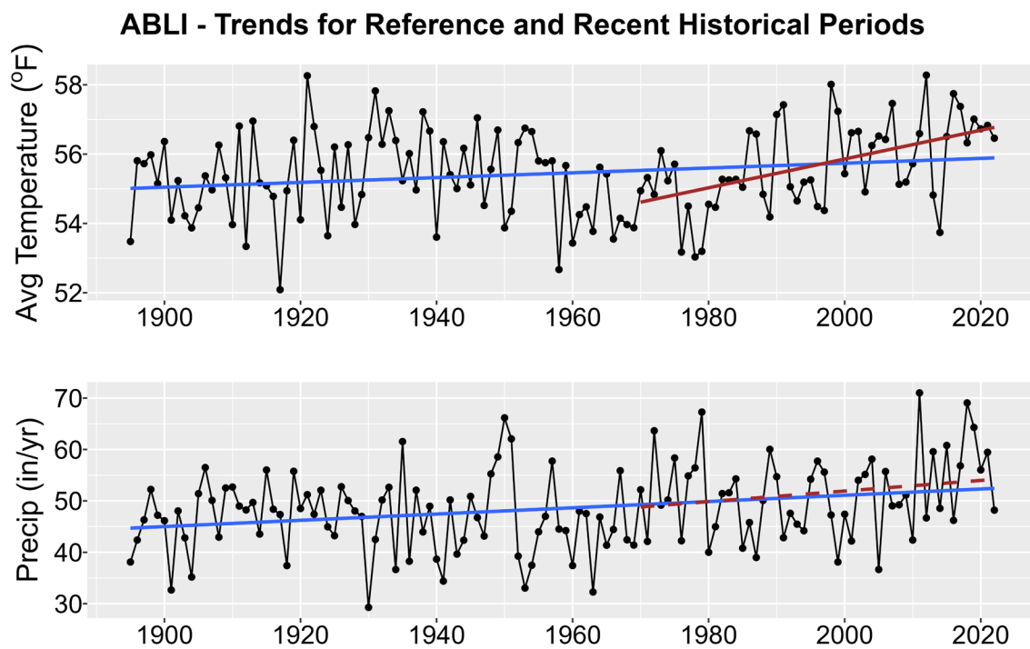
Figure 1. Historical trends in annual average temperature (upper plot) and annual total precipitation (lower plot) for ABLI from 1895-2022. Black points show yearly values while blue lines are linear regressions for the entire period record and red lines for 1970-2022 trends. Solid lines are significant trends (i.e., p < 0.05 ); dashed lines are not statistically significant.
