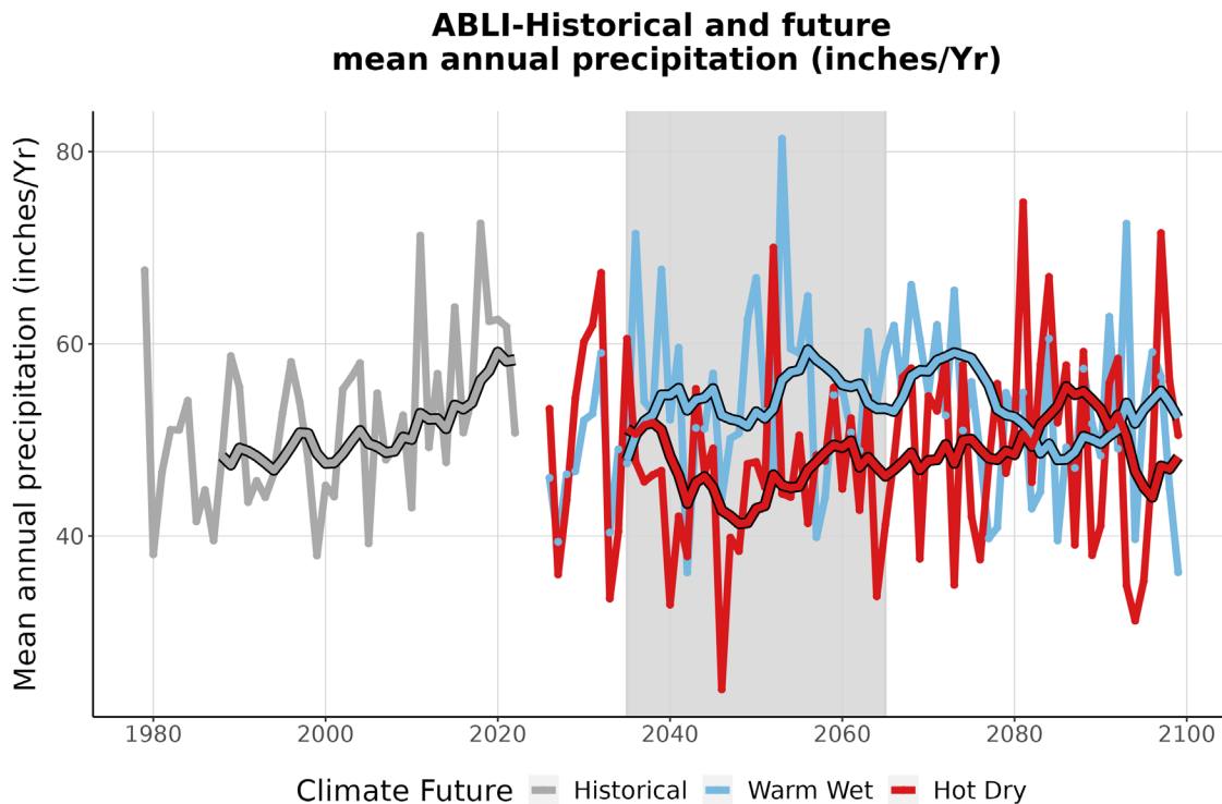
Figure 4. This graph compares observed average annual precipitation at ABLI (inches/year) (1979-2022) with projected average annual precipitation for the two climate futures over the period 2023-2099. The historically observed data is shown in gray, the Warm Wet climate future in blue, and the Hot Dry climate future in red. The smooth line running through each projection is the 10-year running average for historical observations and future projections. The gray-shaded area represents the time period that was averaged (2035-2065) to summarize future projections for the year 2050 (Appendix 1).
